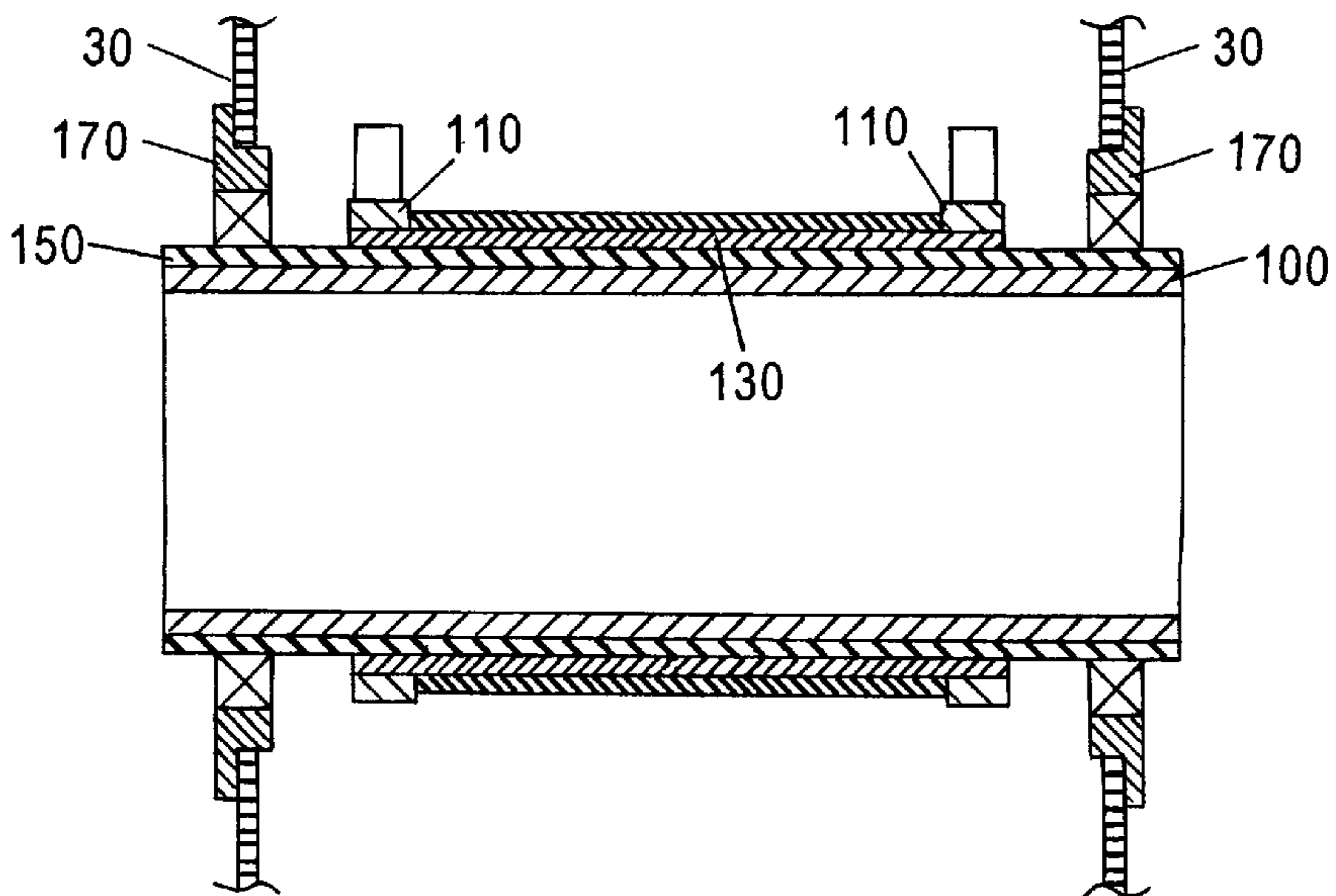
Fig.9 (Prior Art)
