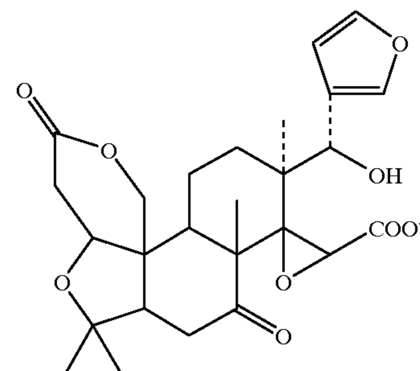
Limonoate A-ring lactone
