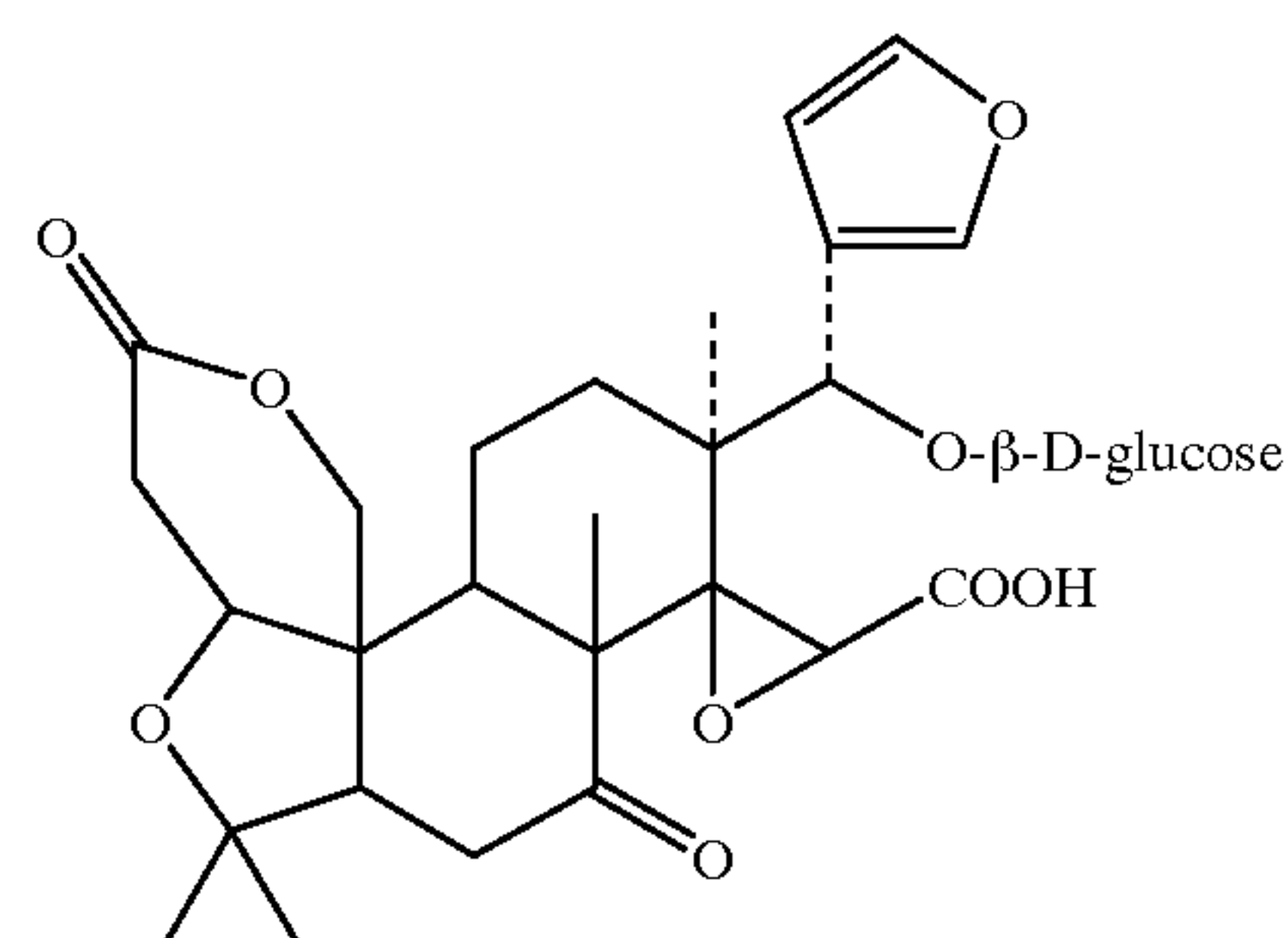
Limonin 17-β-D-glucopyranoside
