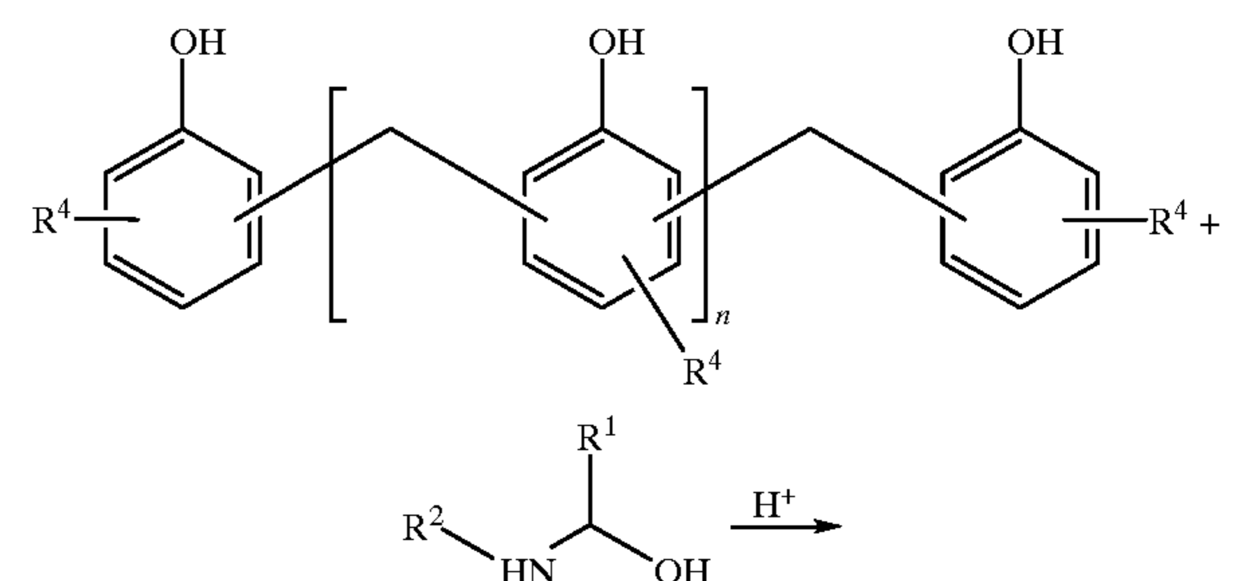
REACTION I
