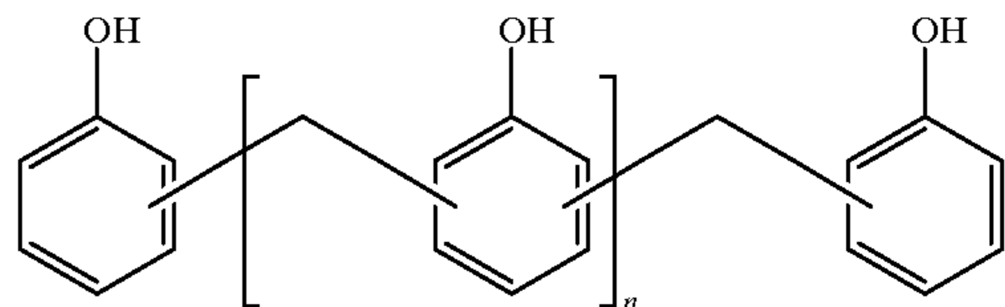
CHEMICAL STRUCTURE A
