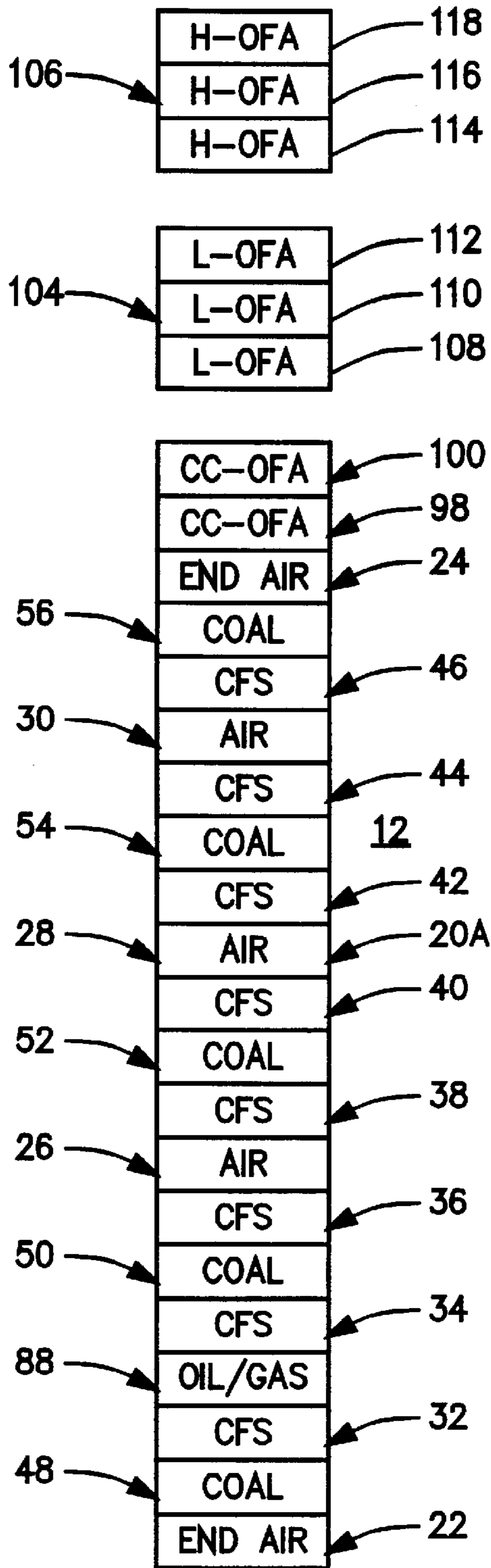
Fig. 10 (PRIOR ART)
