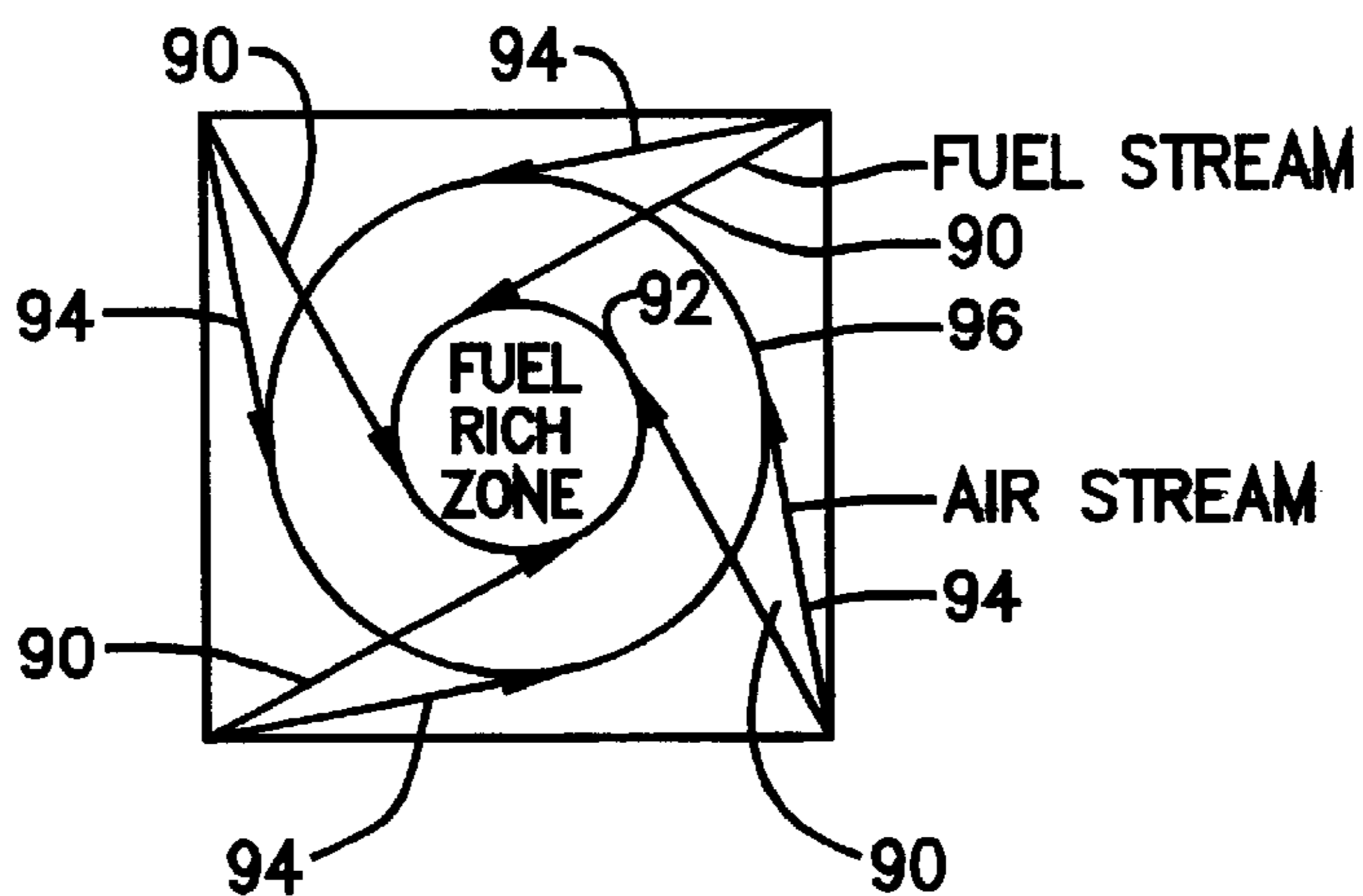
Fig. 5 (PRIOR ART)
