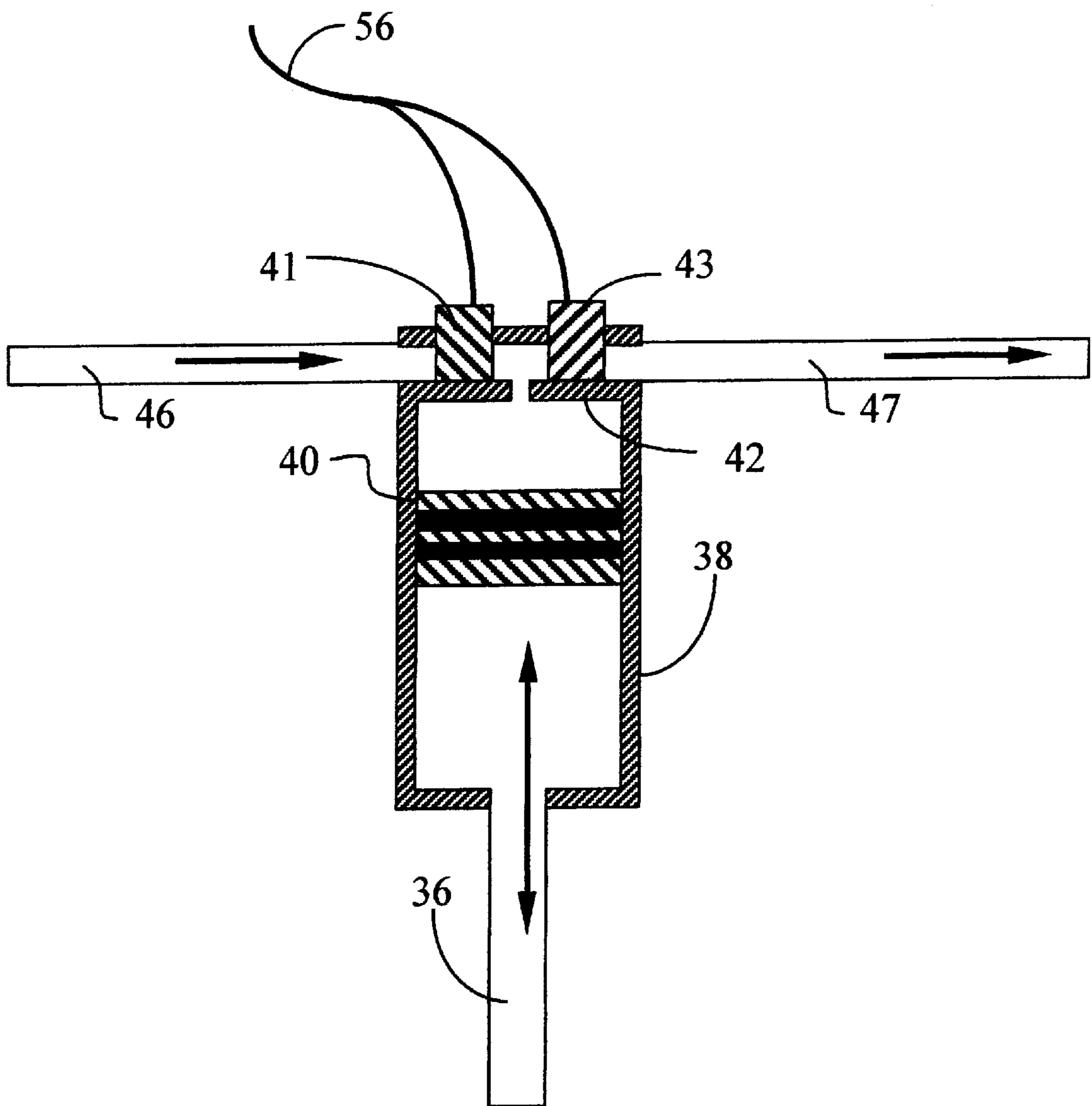
Isolation Metering Cylinder (IMC)
