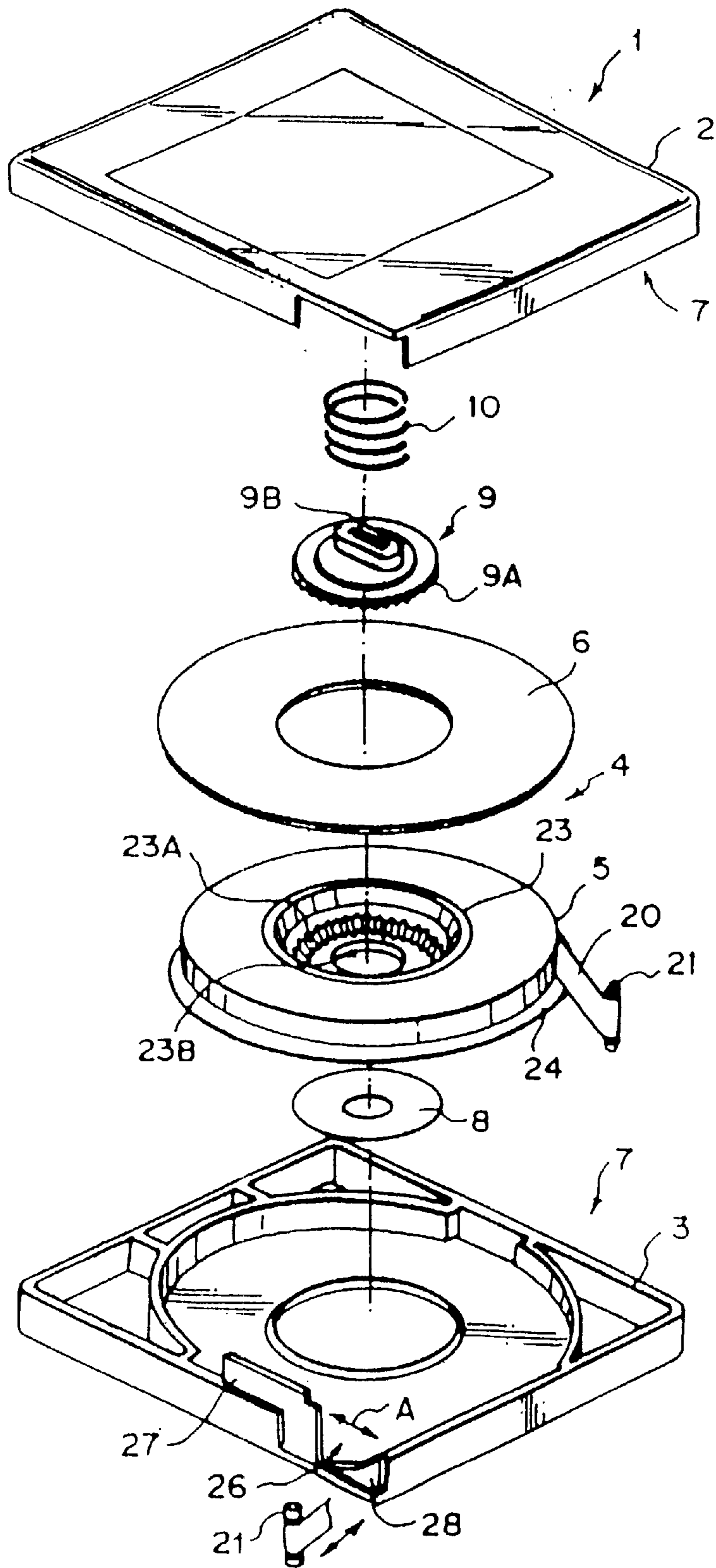
FIG. 1 PRIOR ART
