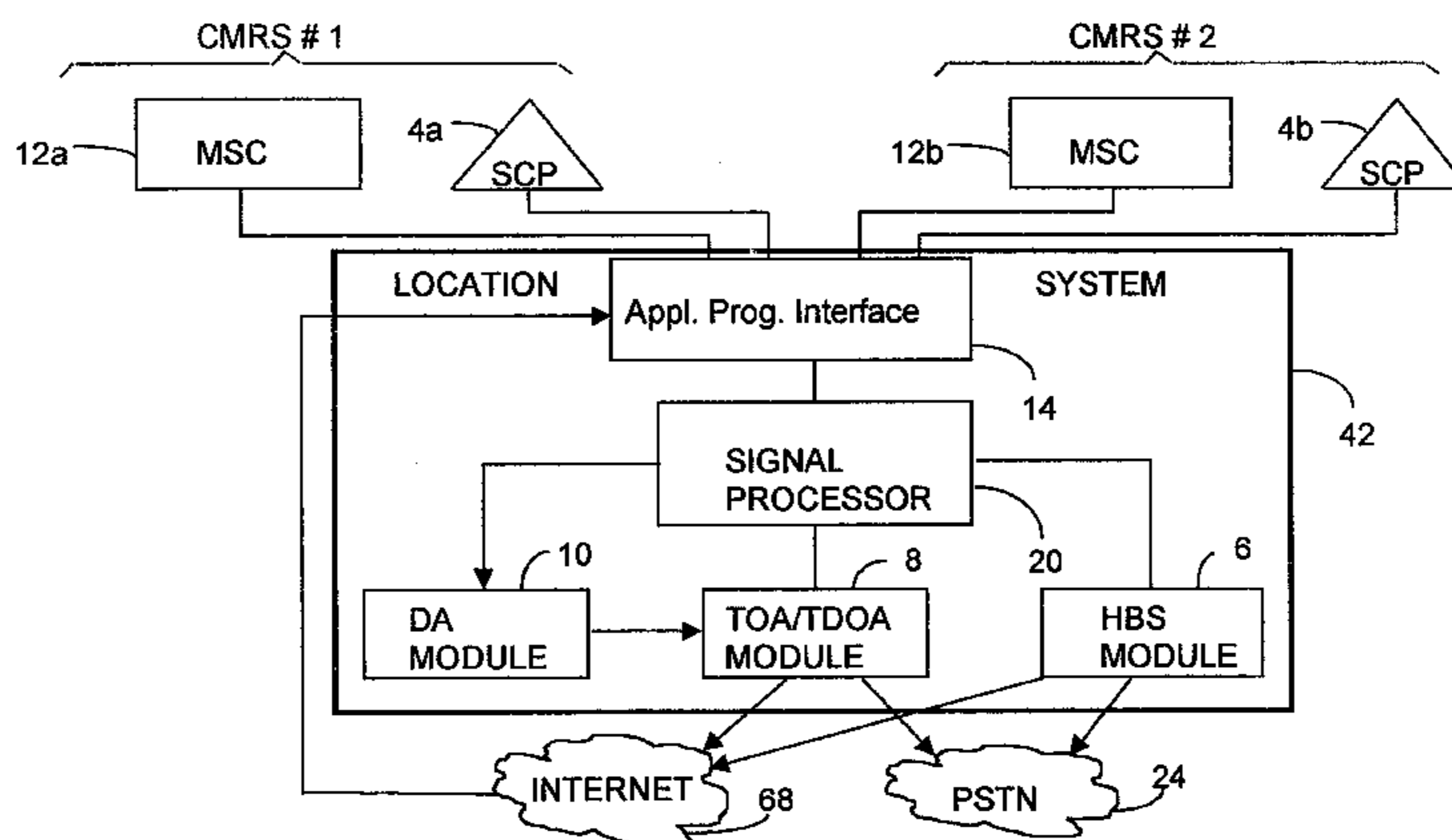
WIRELESS LOCATION USING MULTIPLE CMRSs
