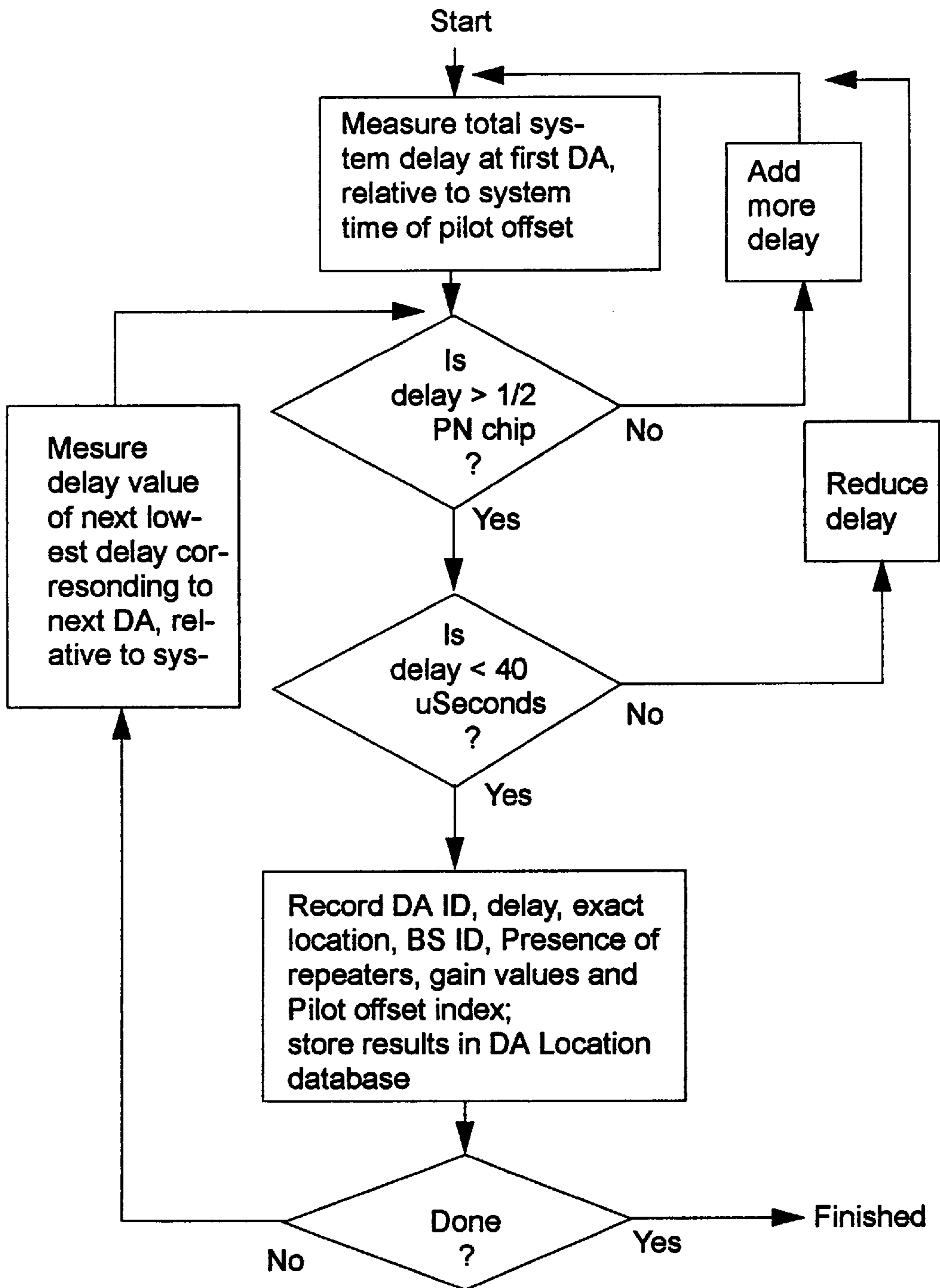
FIG. 8: DA Installation Procedure for Wireless Location
