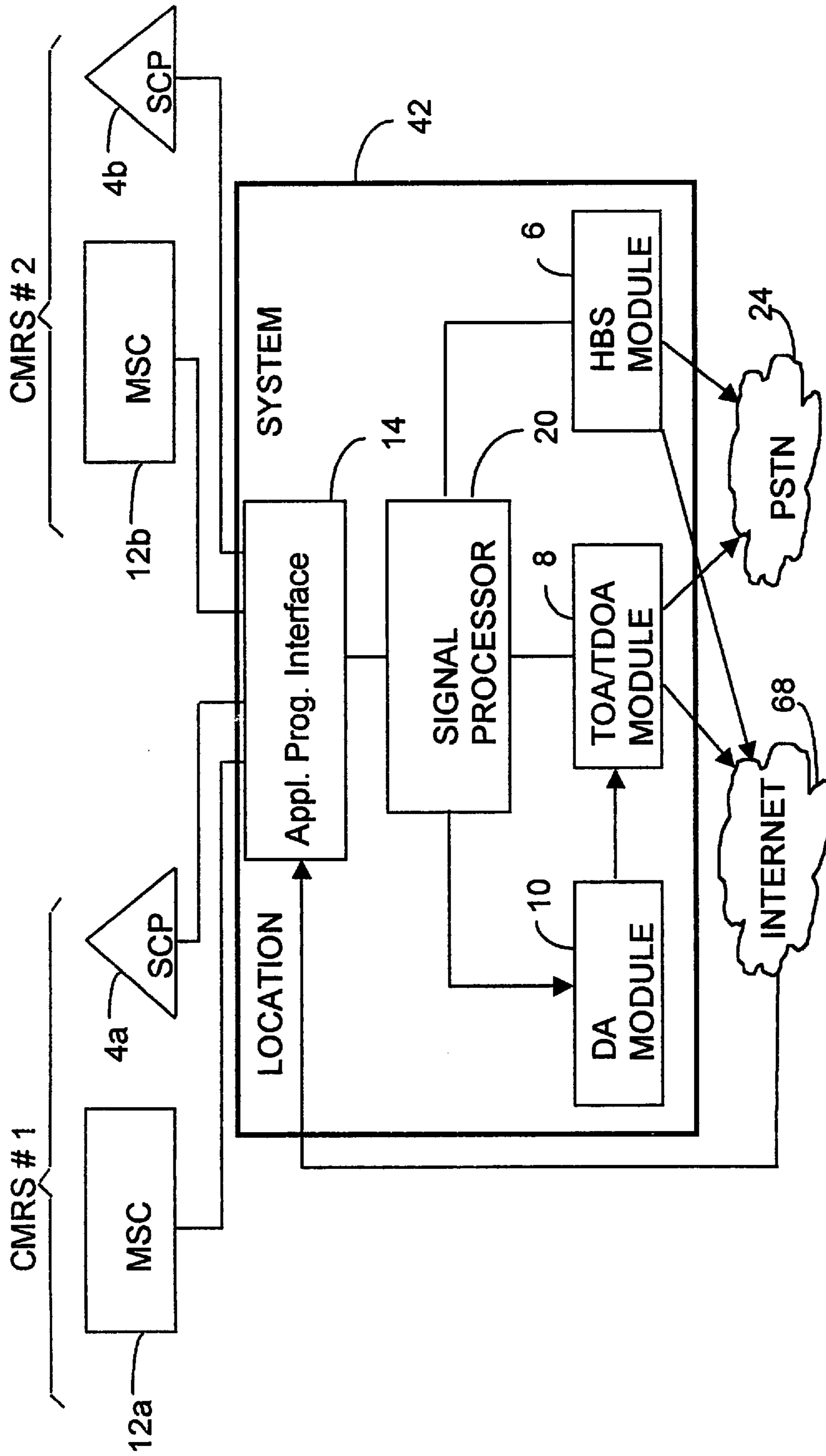
FIG. 1: WIRELESS LOCATION USING MULTIPLE CMRSS
