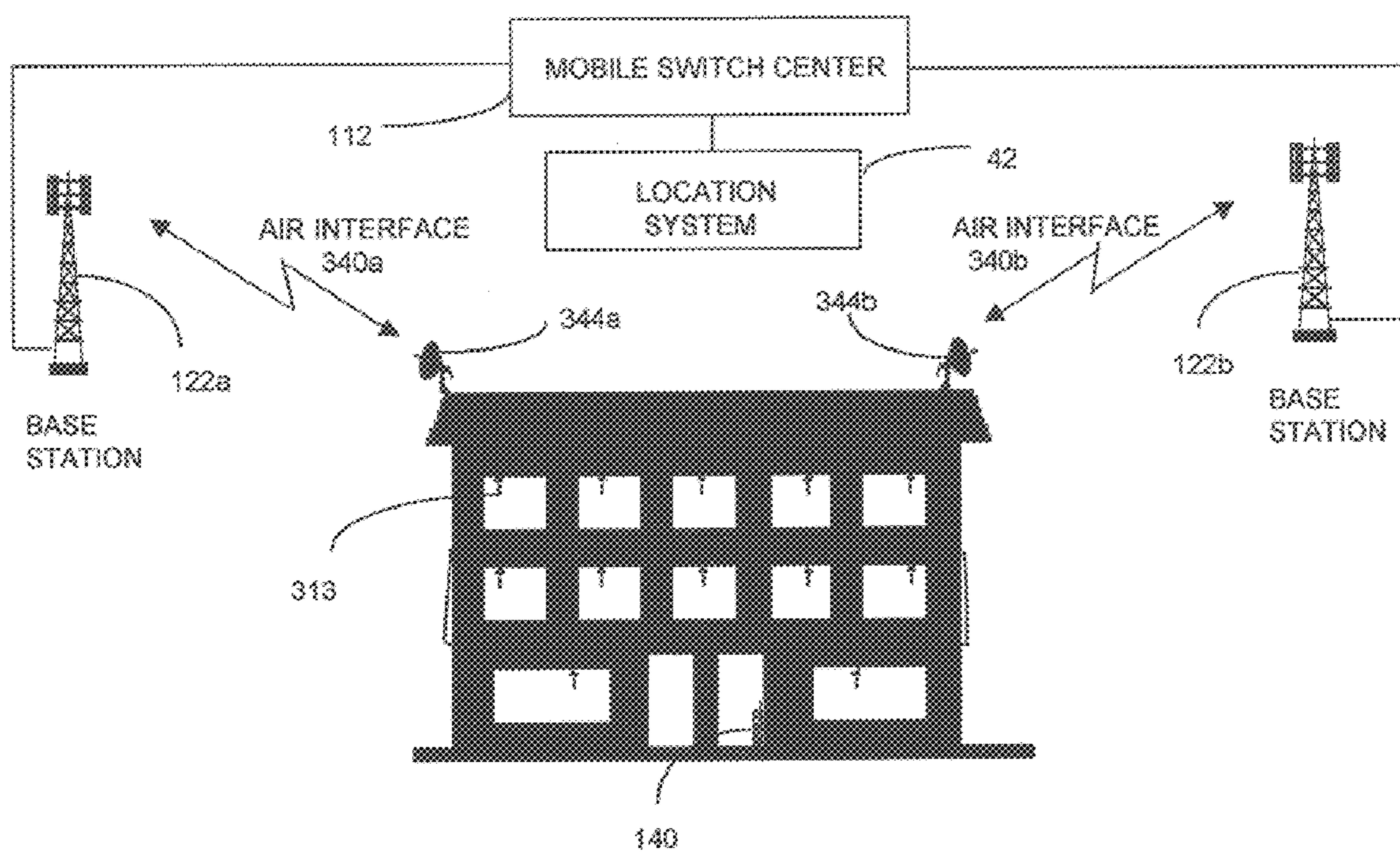
FIG. 11: Dual-Microwave Access Distributed Antenna Example
