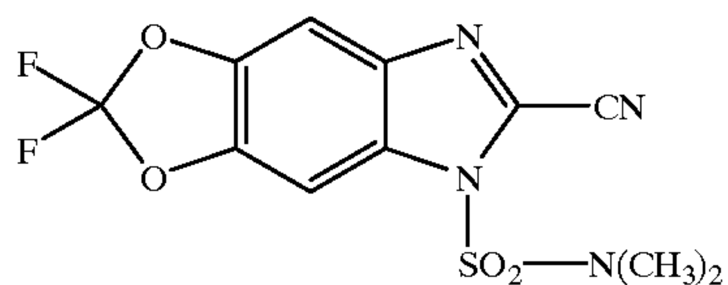
2-Cyano-6,6-difluoro-1-dimethylaminosulphonyl-[1,3]dioxolo[4,5-f]benzimidazole
