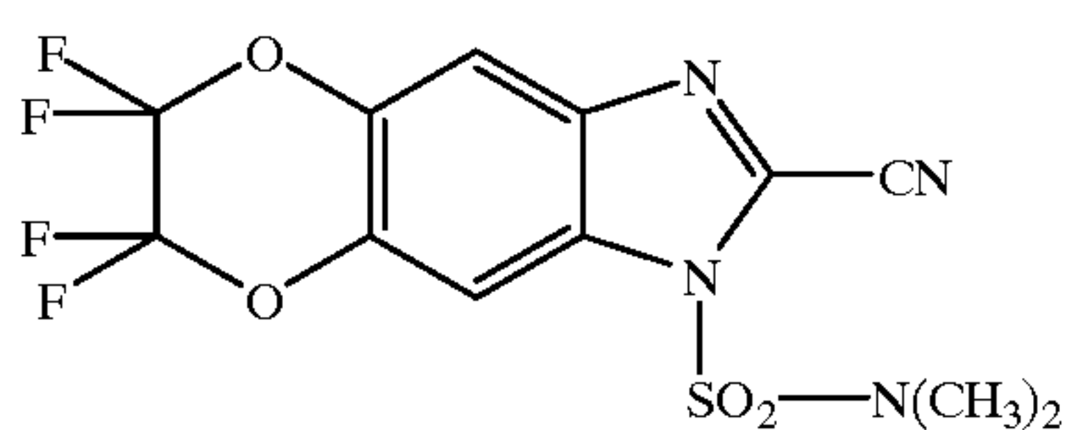
2-Cyano-1-dimethylaminosulphonyl-6,6,7,7-tetrafluoro-[1,4]dioxino[2,3-f]benzimidazole
