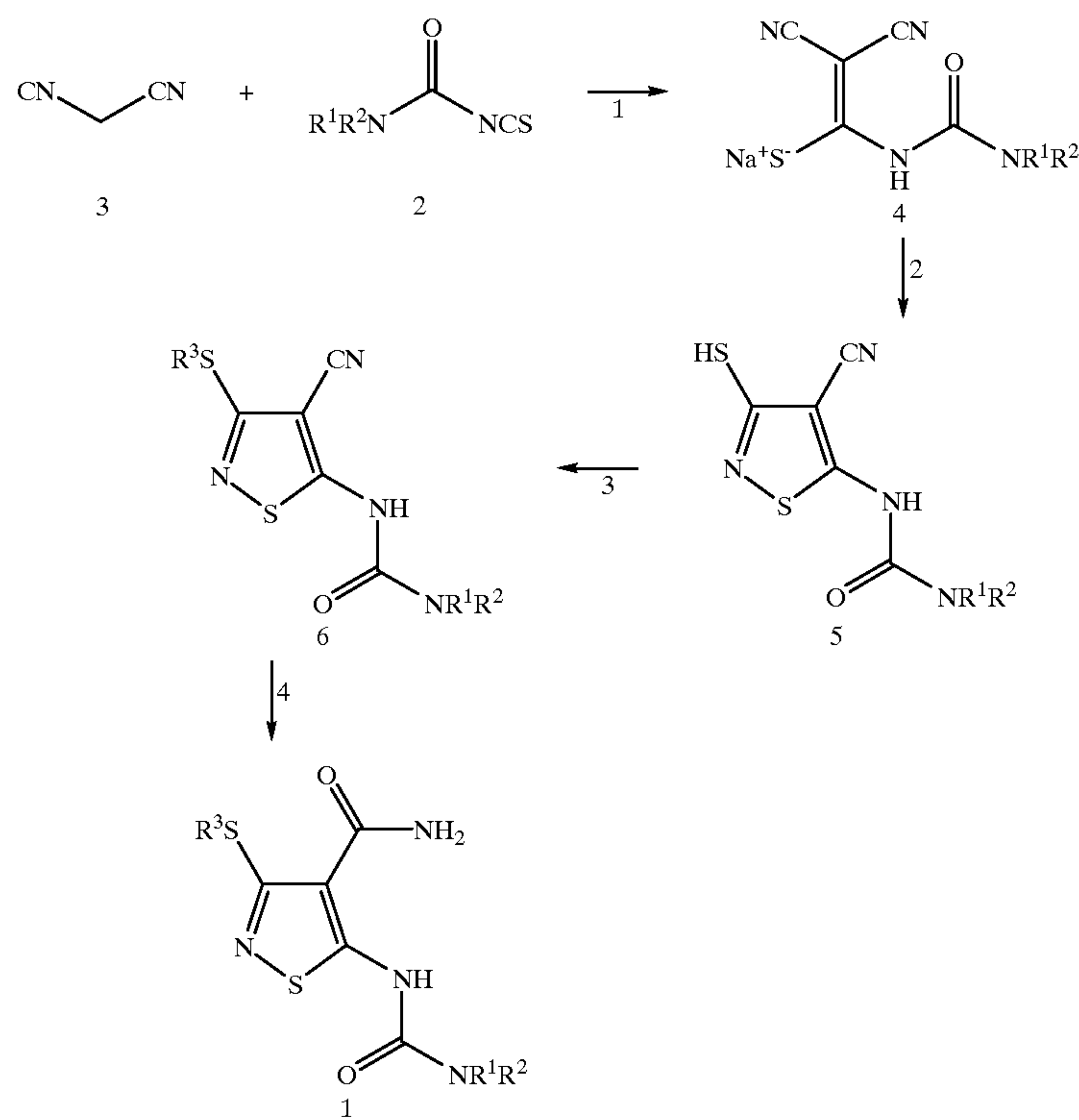
Scheme 1
