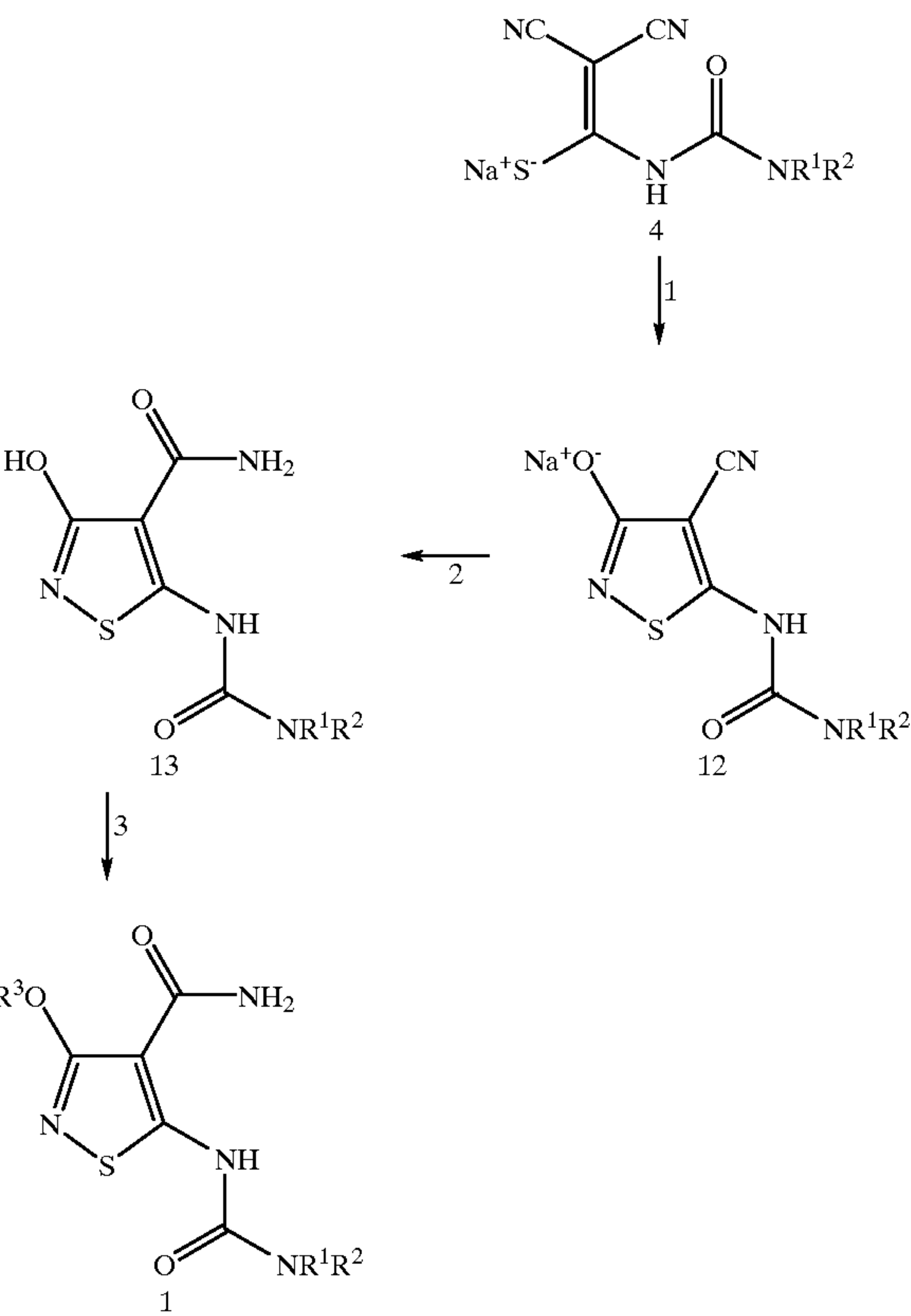
Scheme 3
