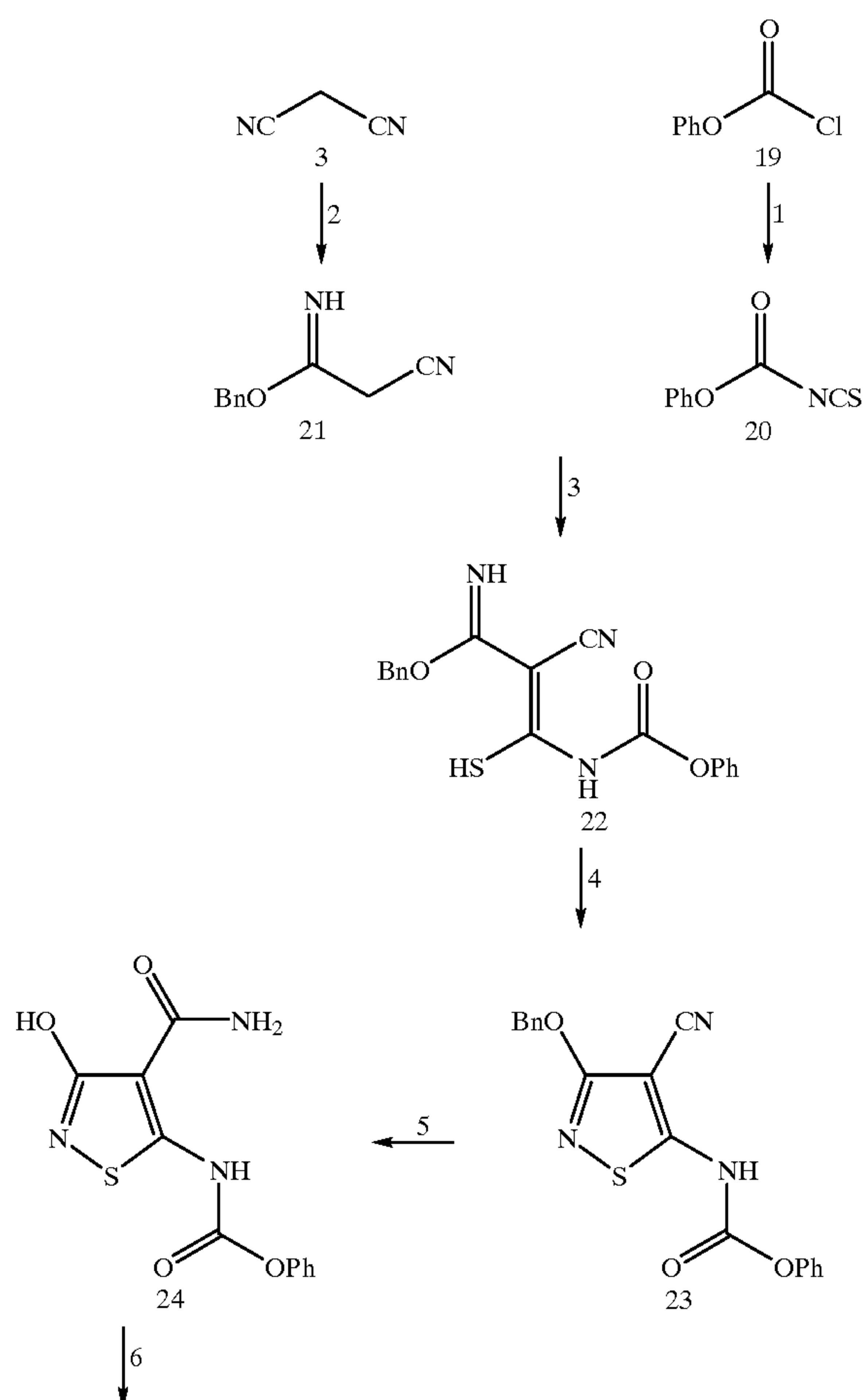
Scheme 5
