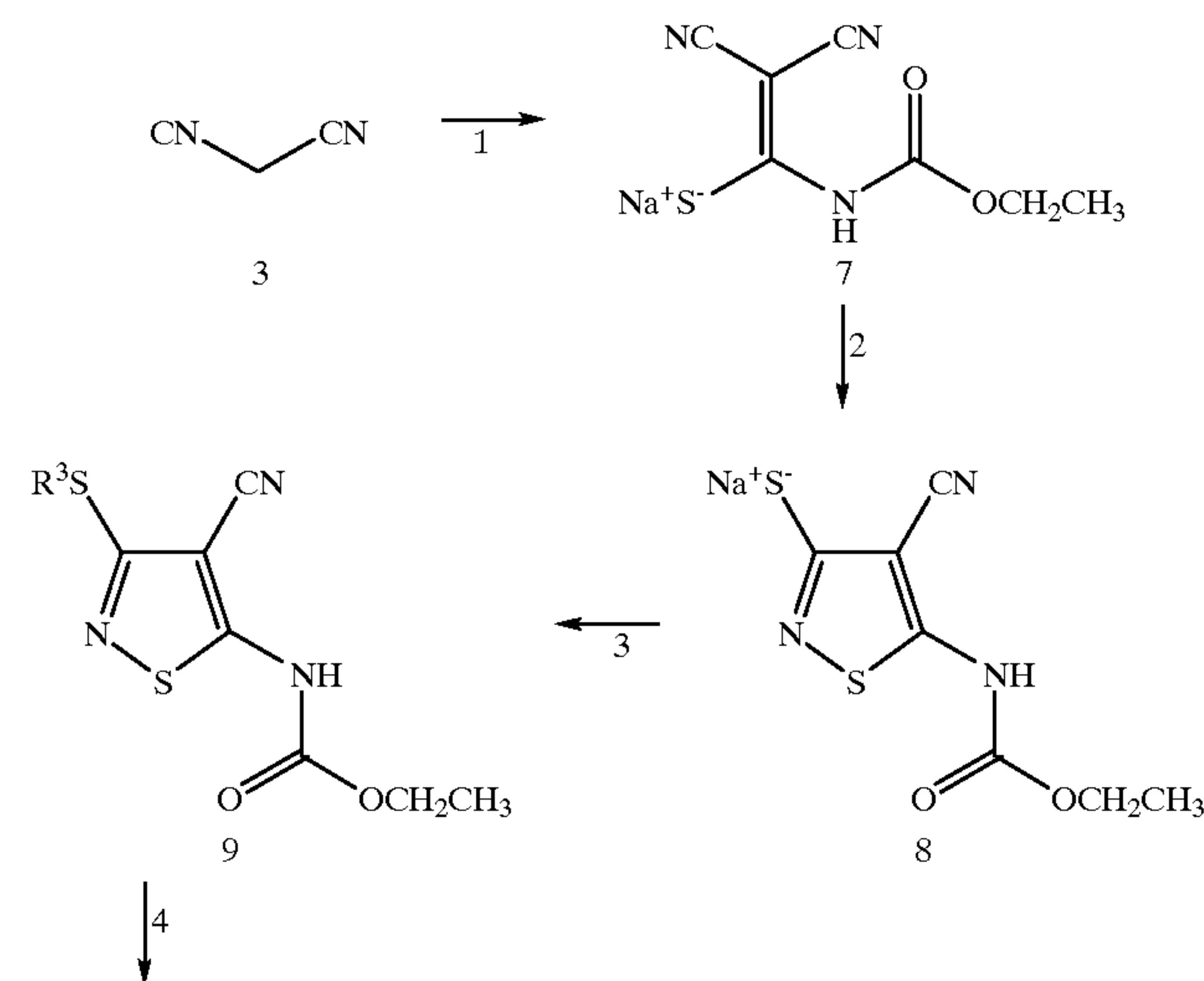
Scheme 2
