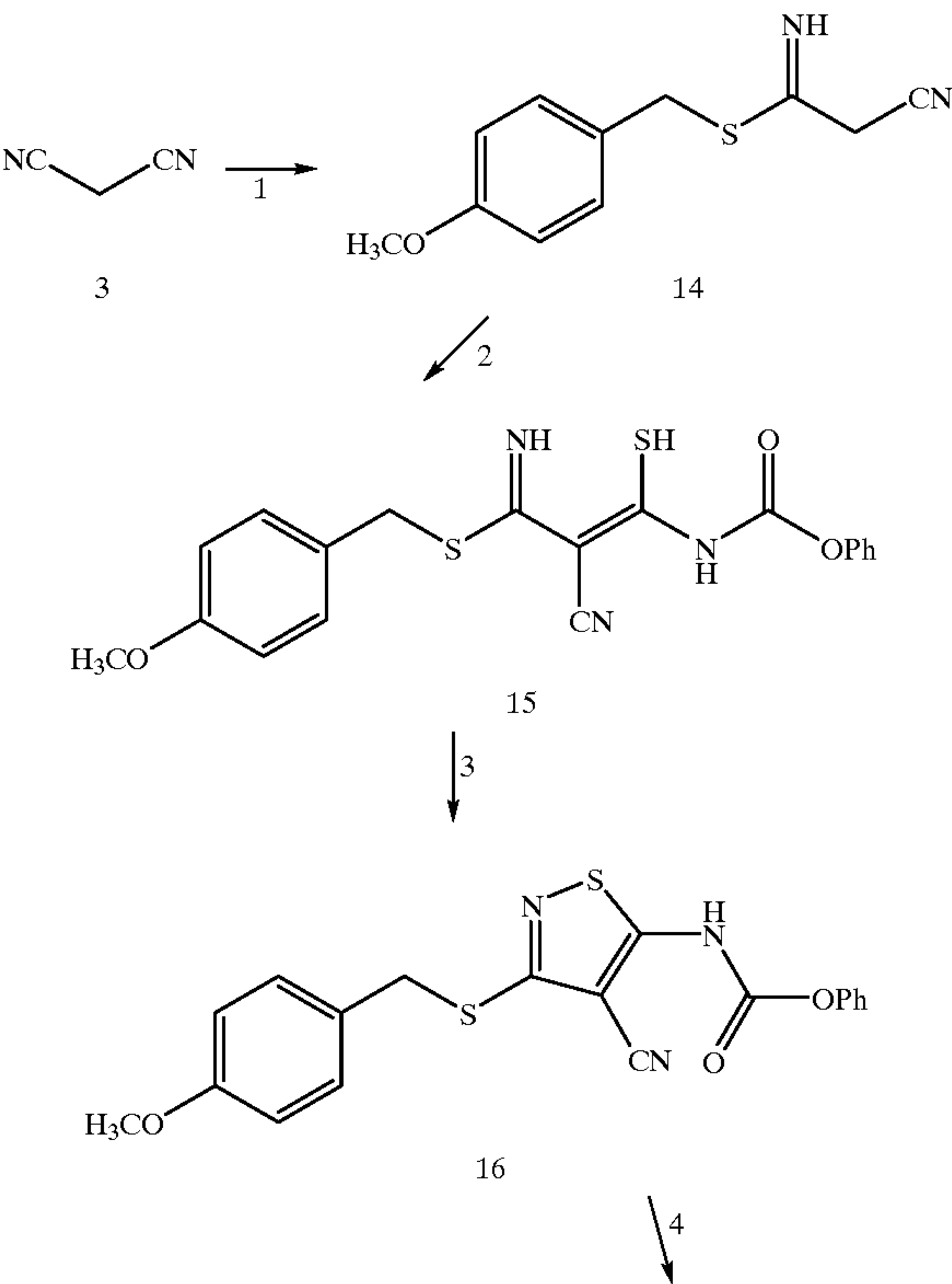
Scheme 4
