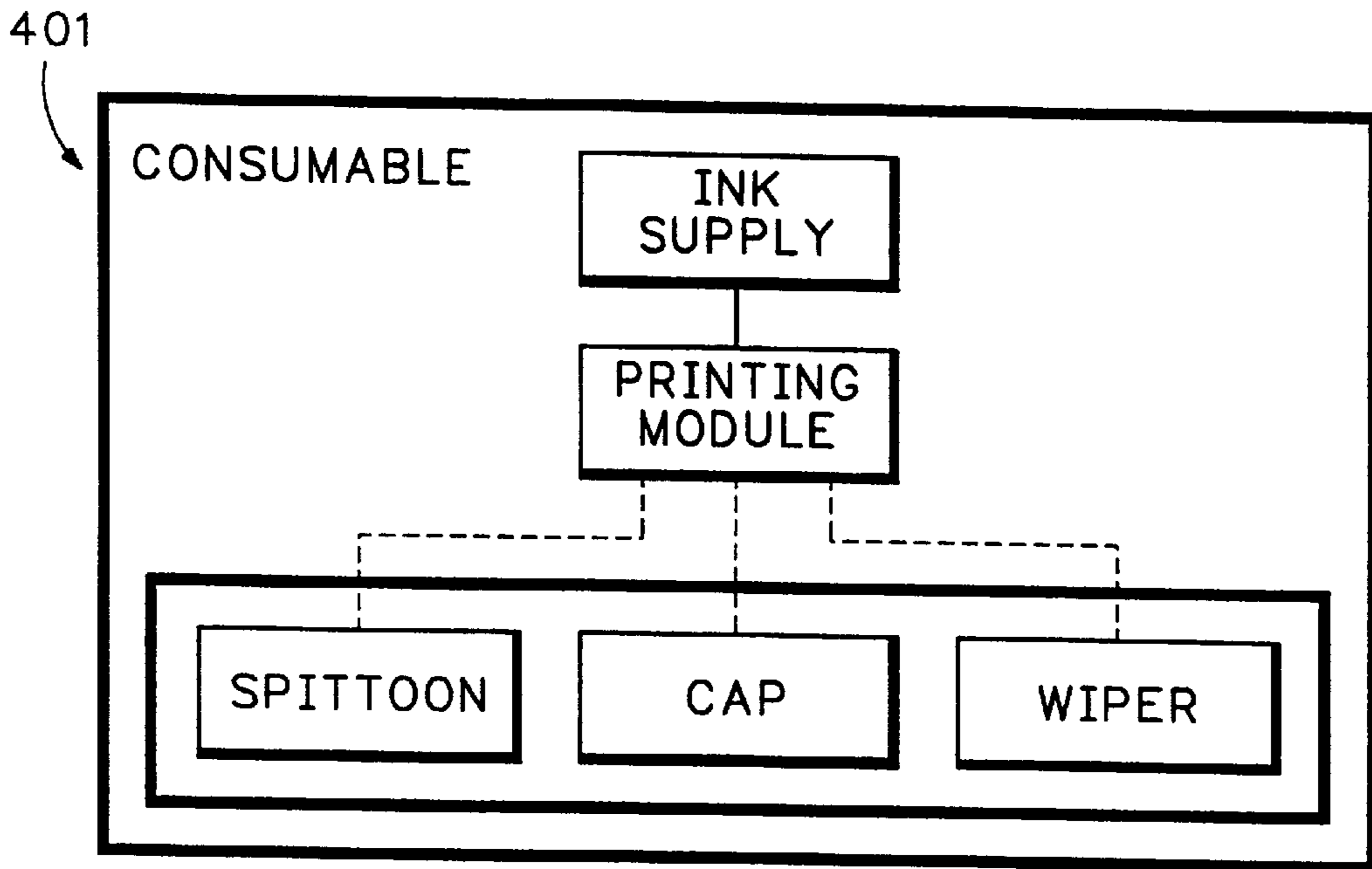
FLUIDIC BLOCK DIAGRAM
