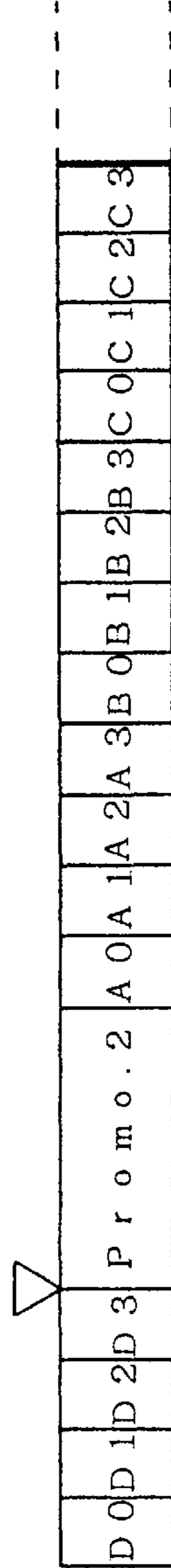
FIG. 3D Output Of # 2 Channel
