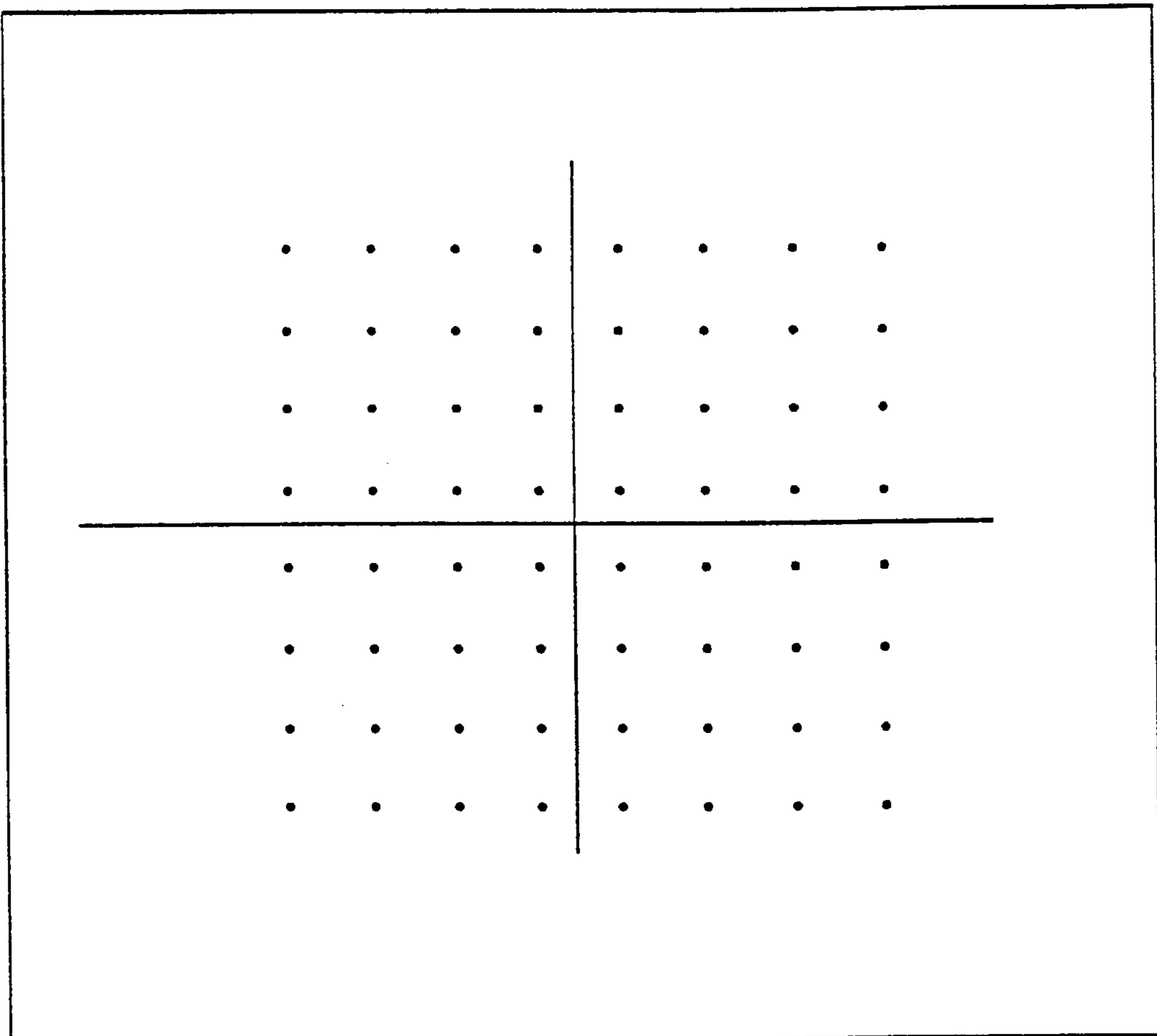
IDEAL 64-QAM
