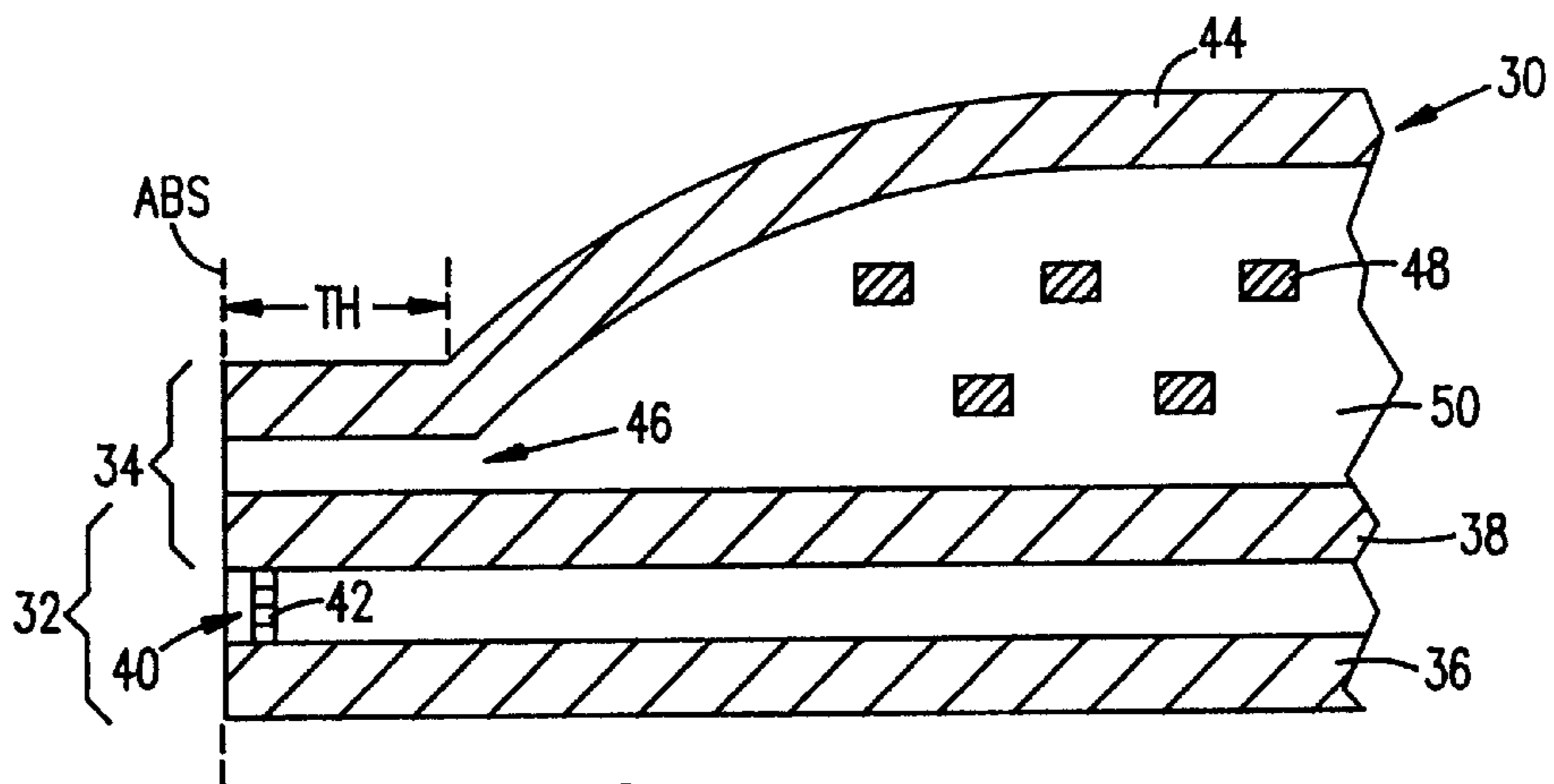
FIG. 1C PRIOR ART
