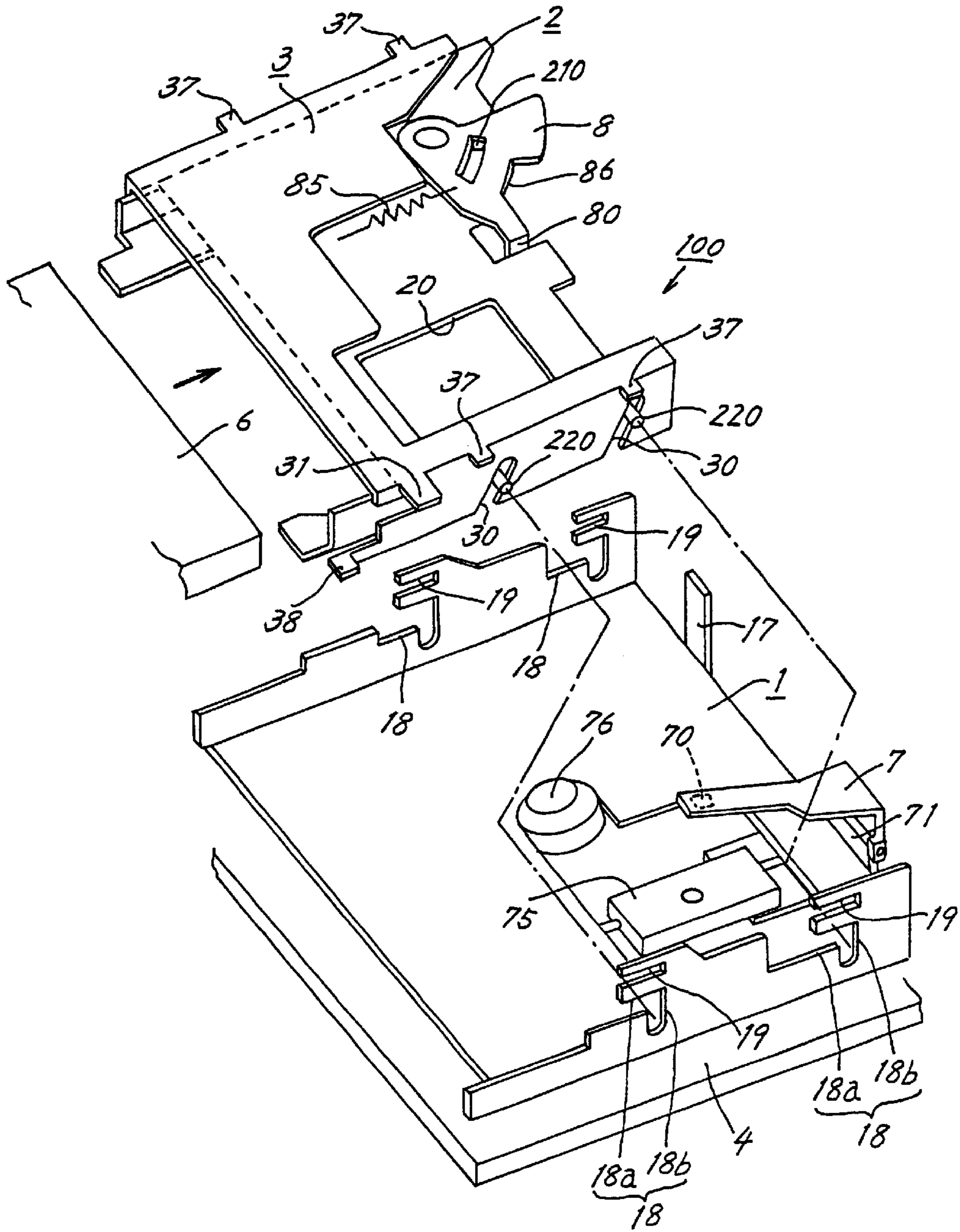
FIG.17 PRIOR ART
