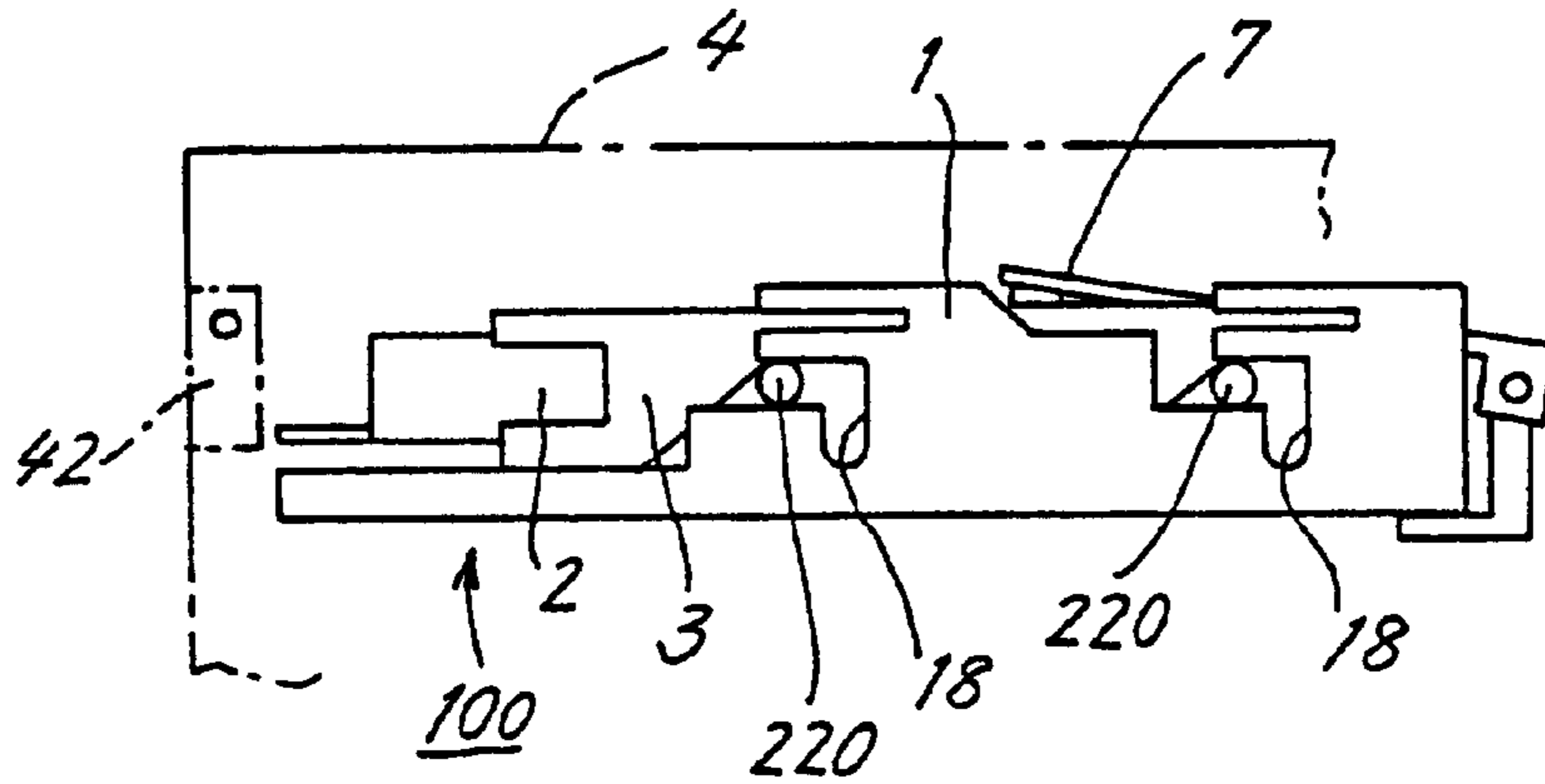
FIG. 21 PRIOR ART
