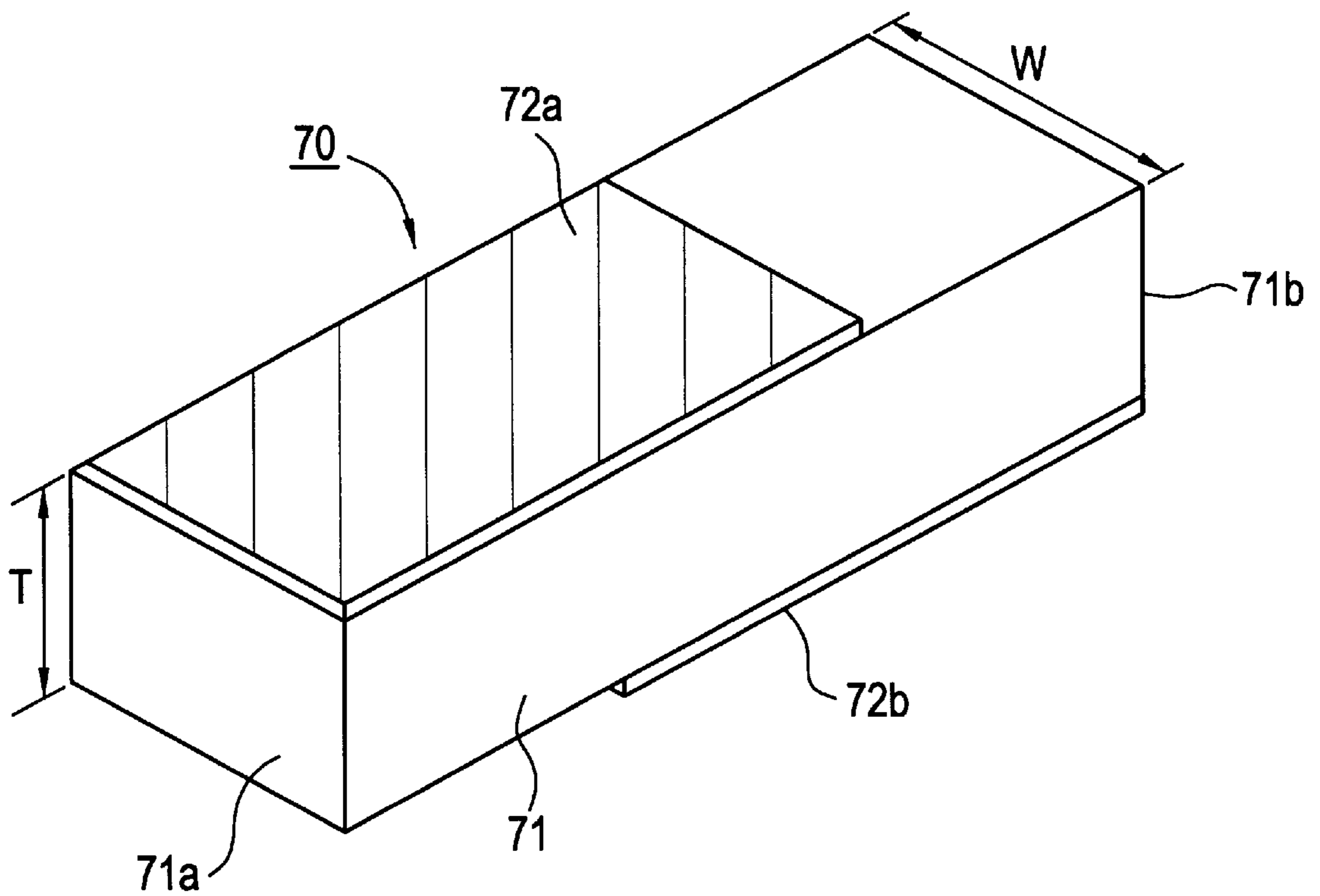
FIG. 19 PRIOR ART
