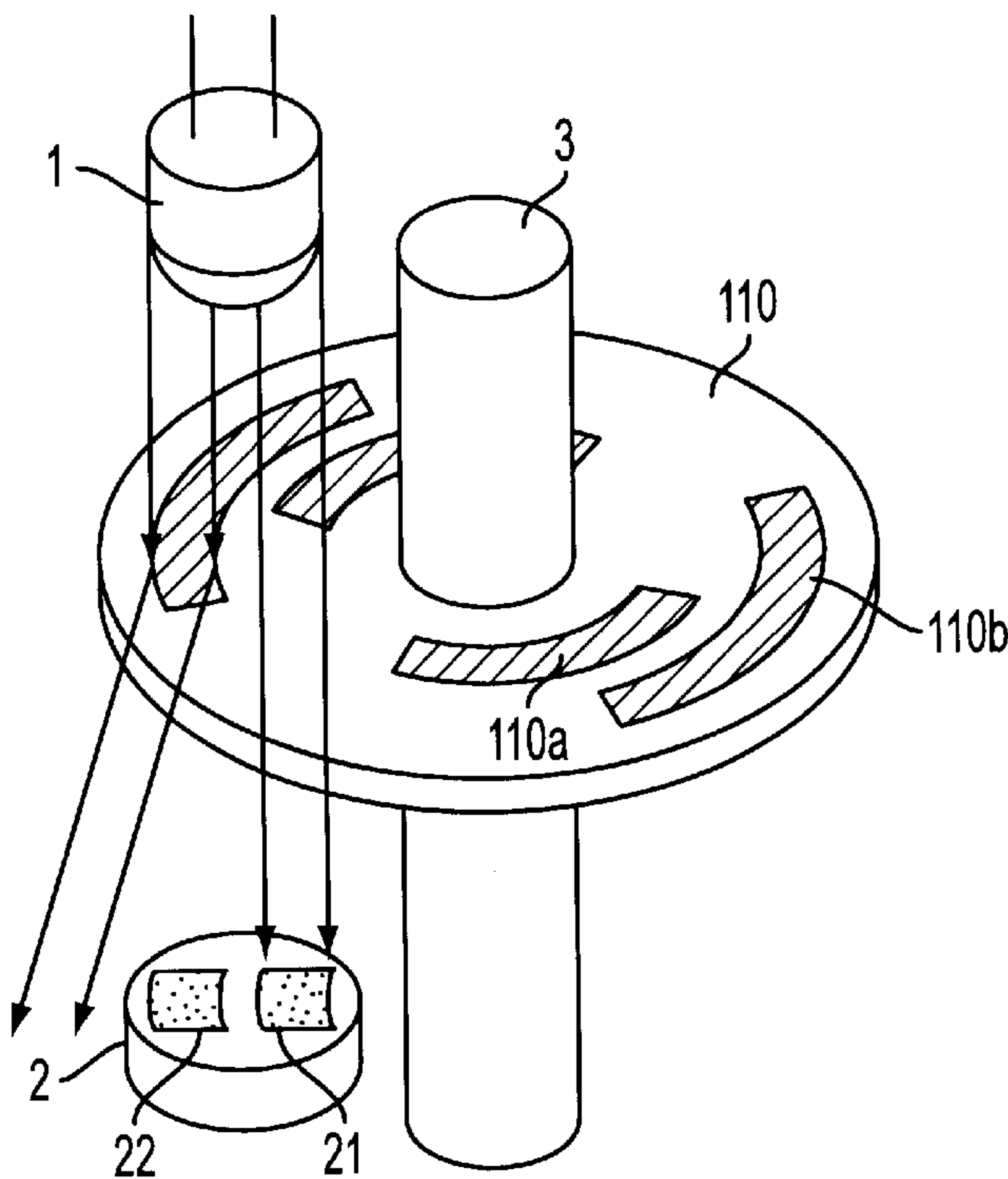
FIG. 24 (PRIOR ART)
