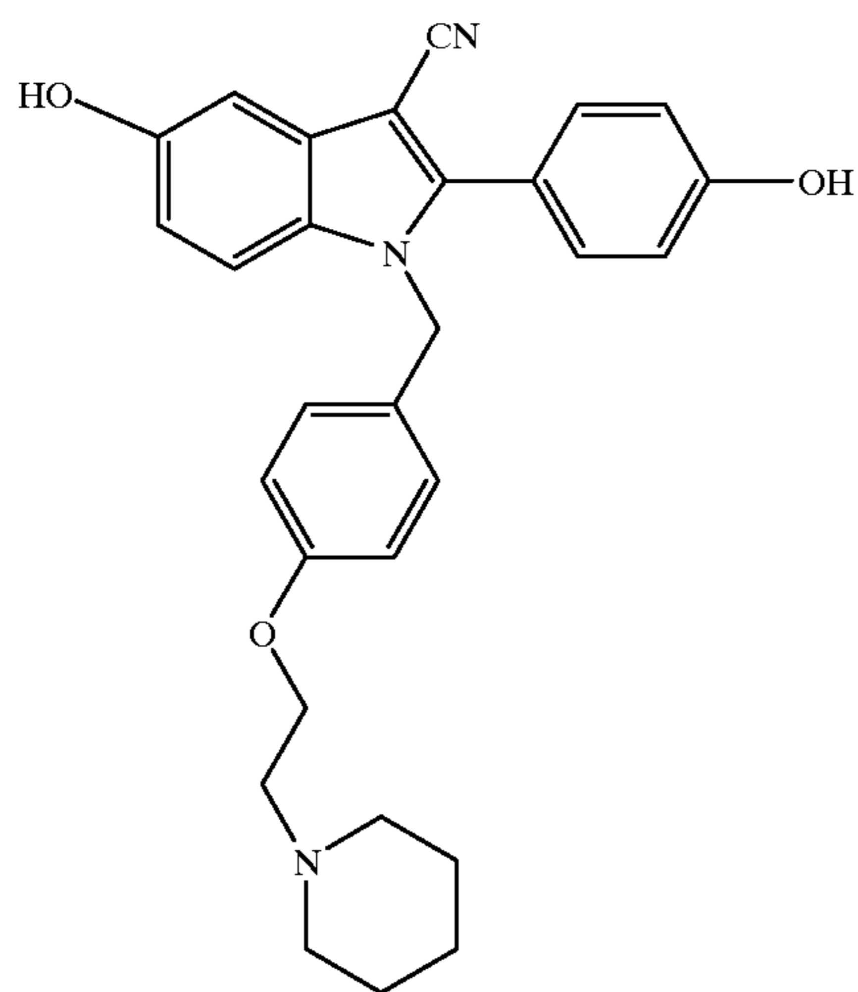
Example No. 138
