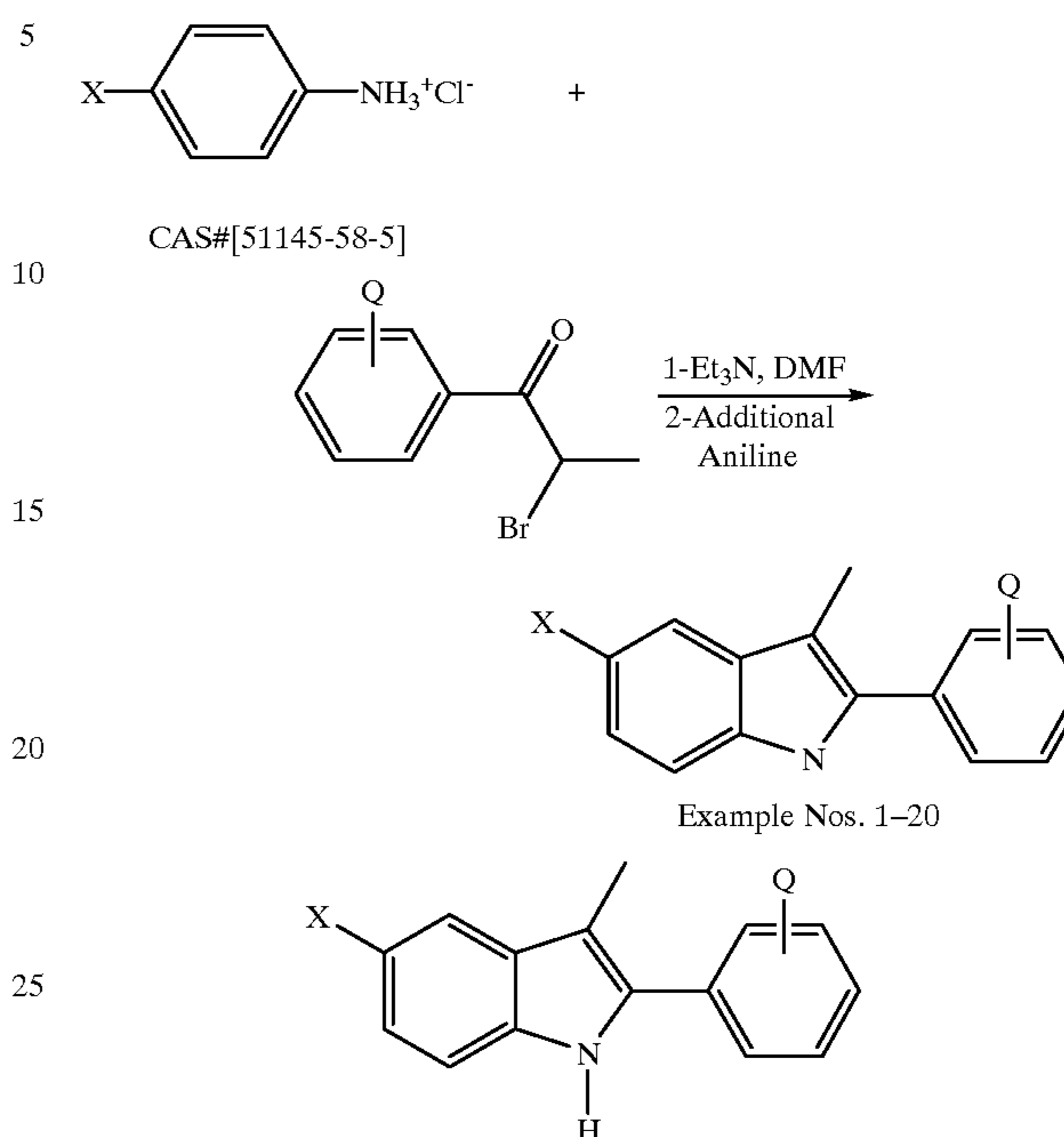
Scheme 8
