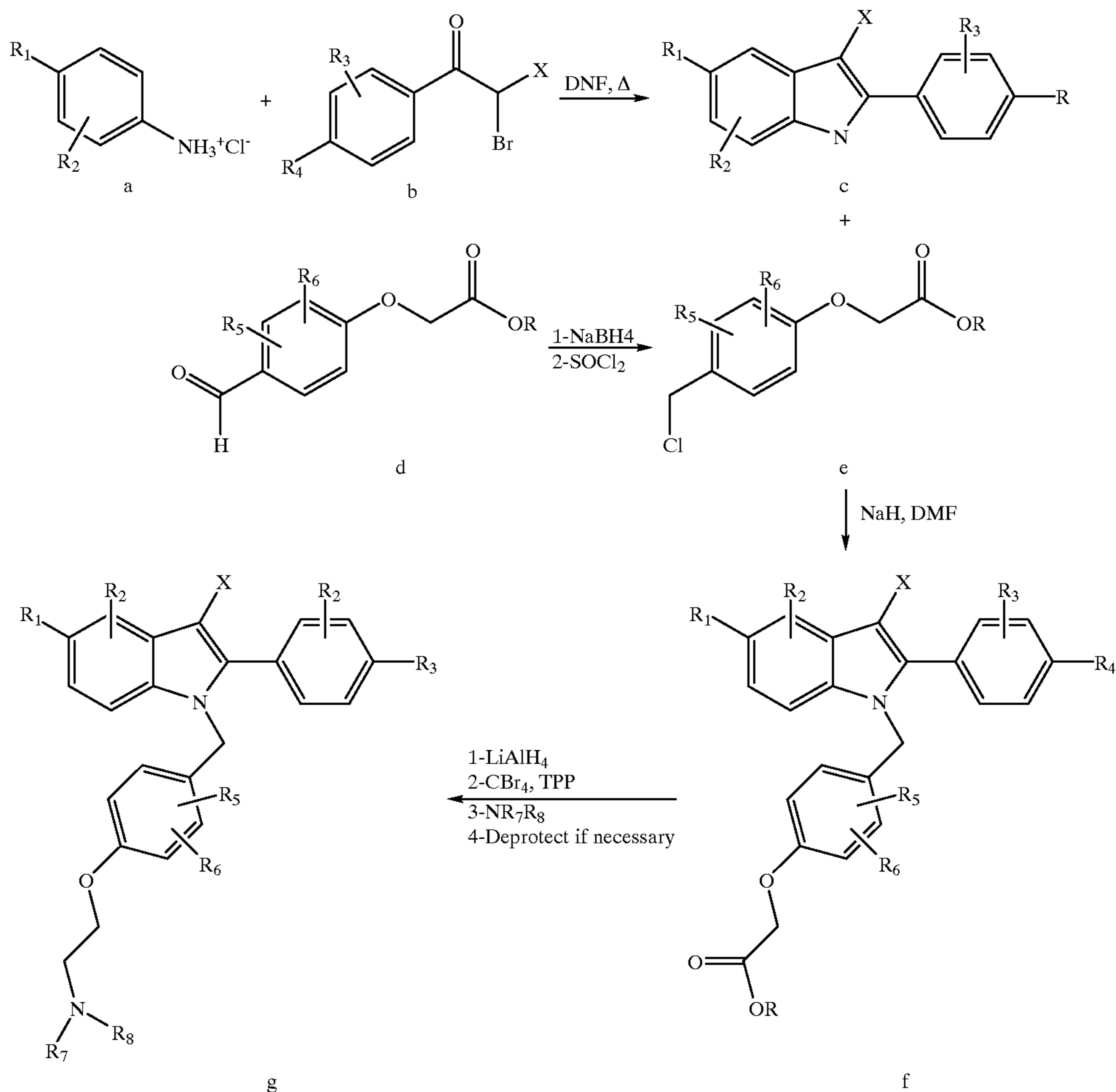
Scheme 1
