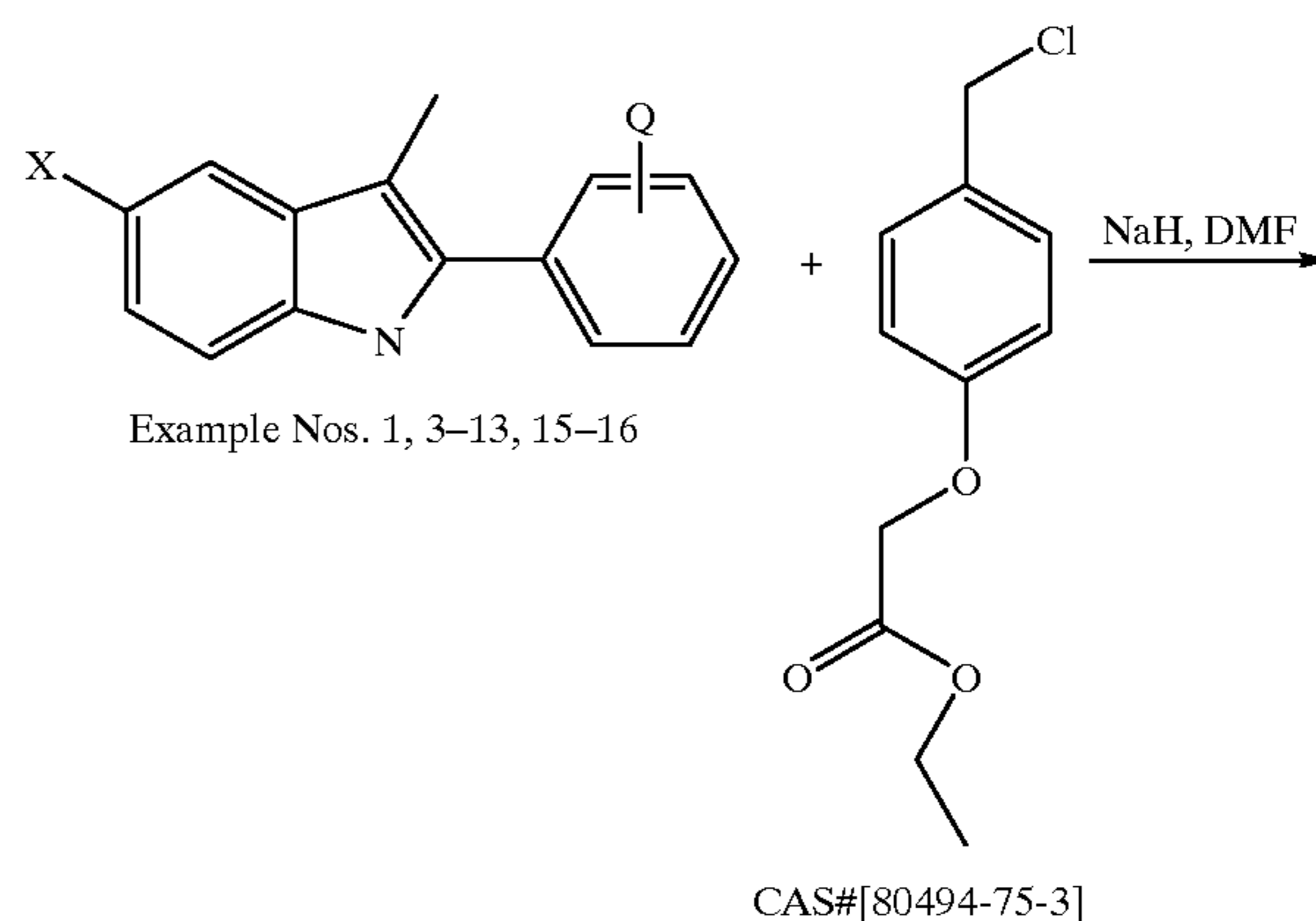
Scheme 9
