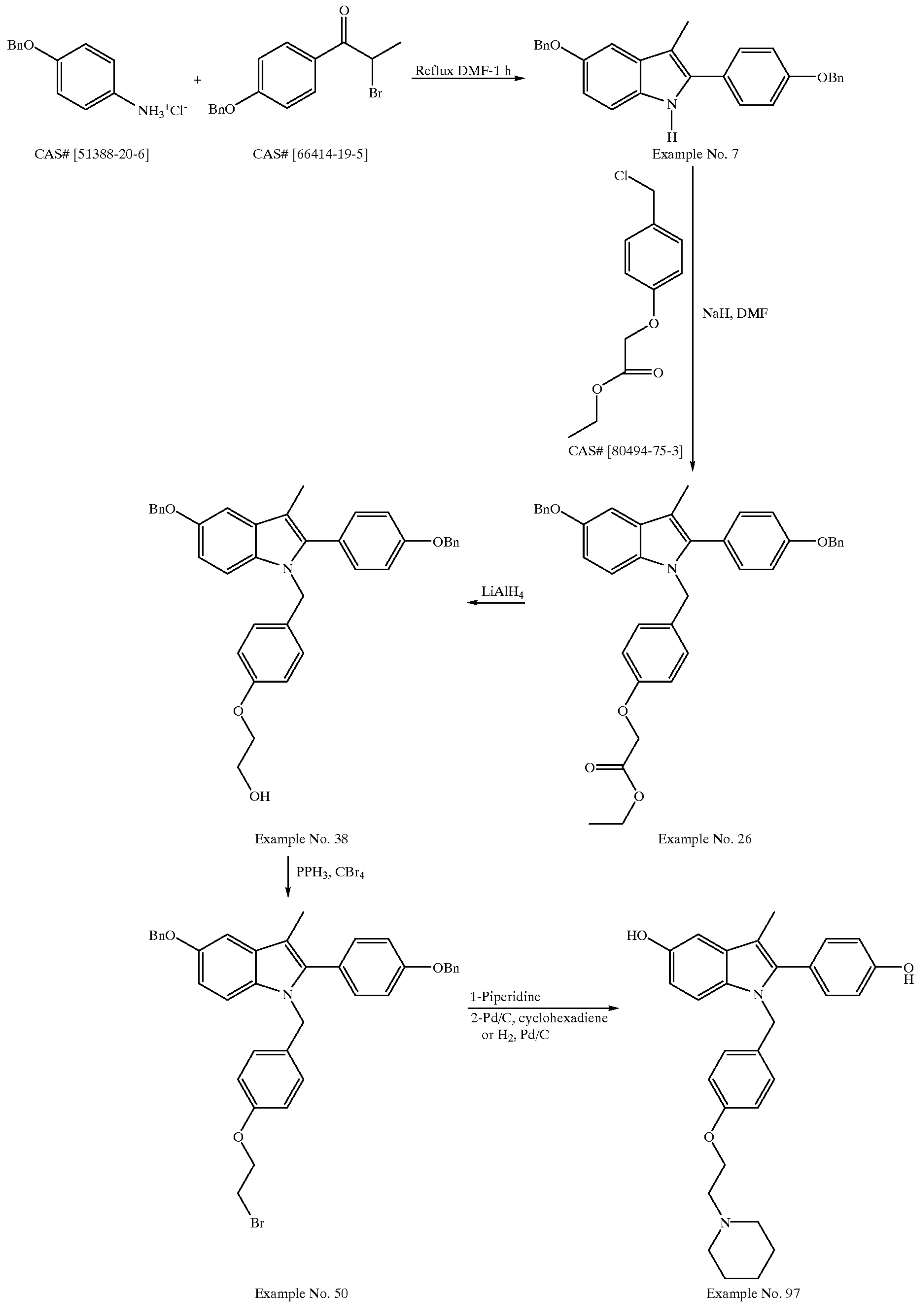
Scheme 3
