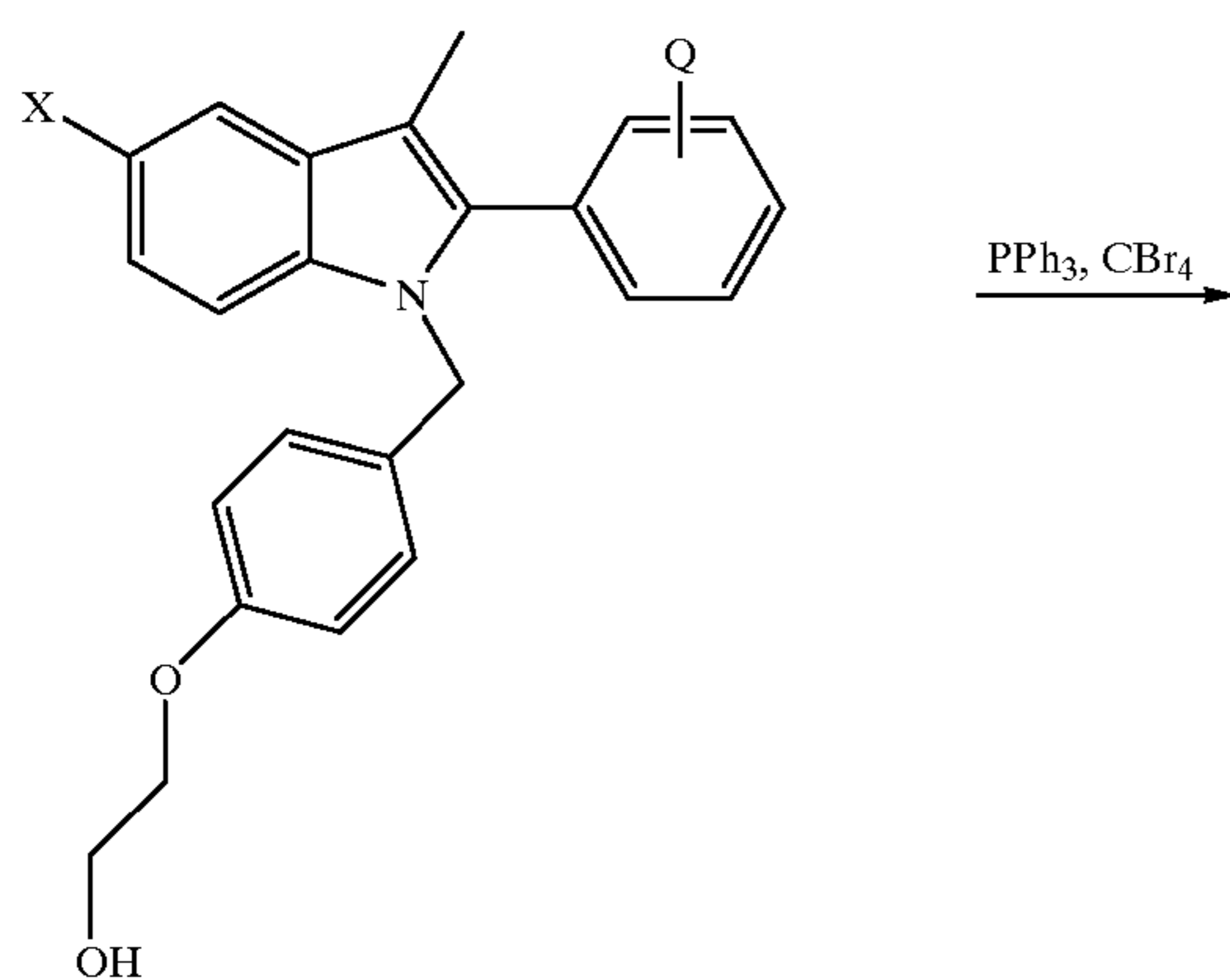
Scheme 11
