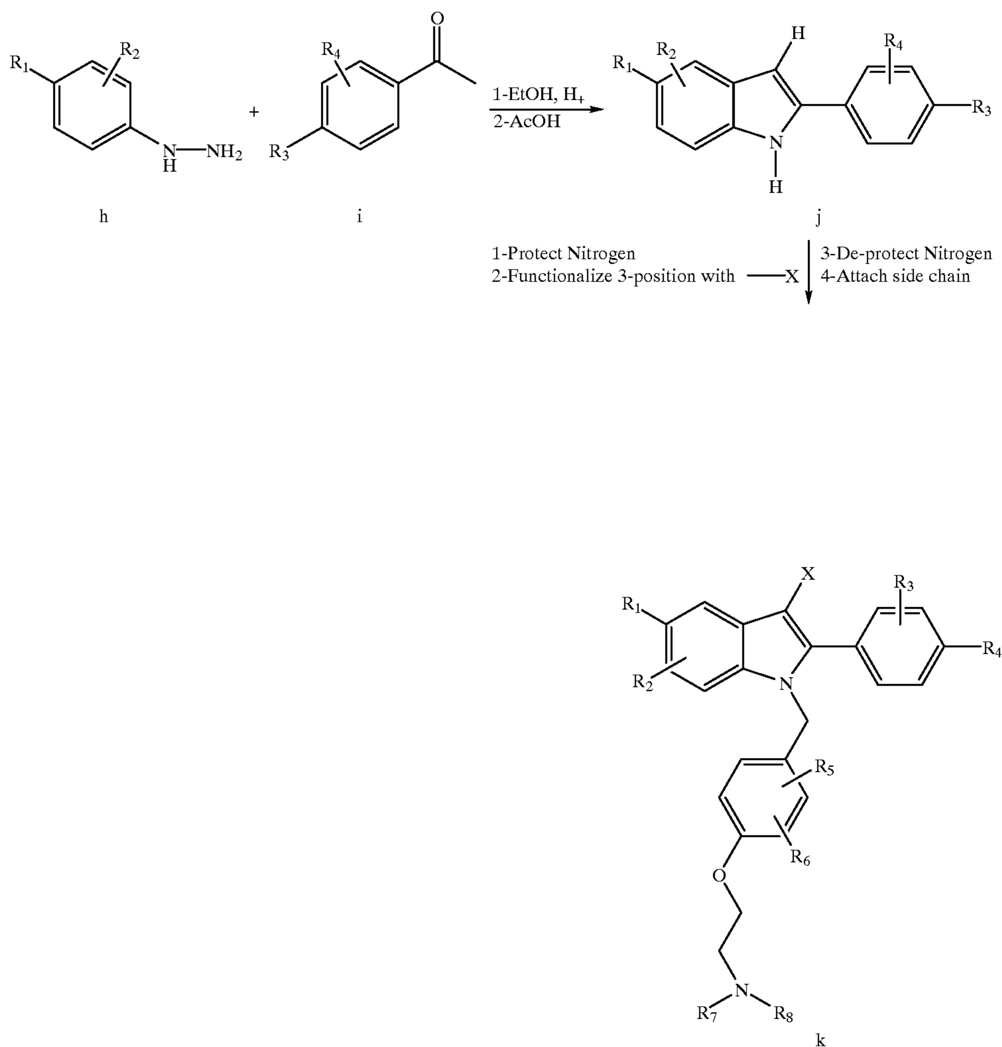
Scheme 2
