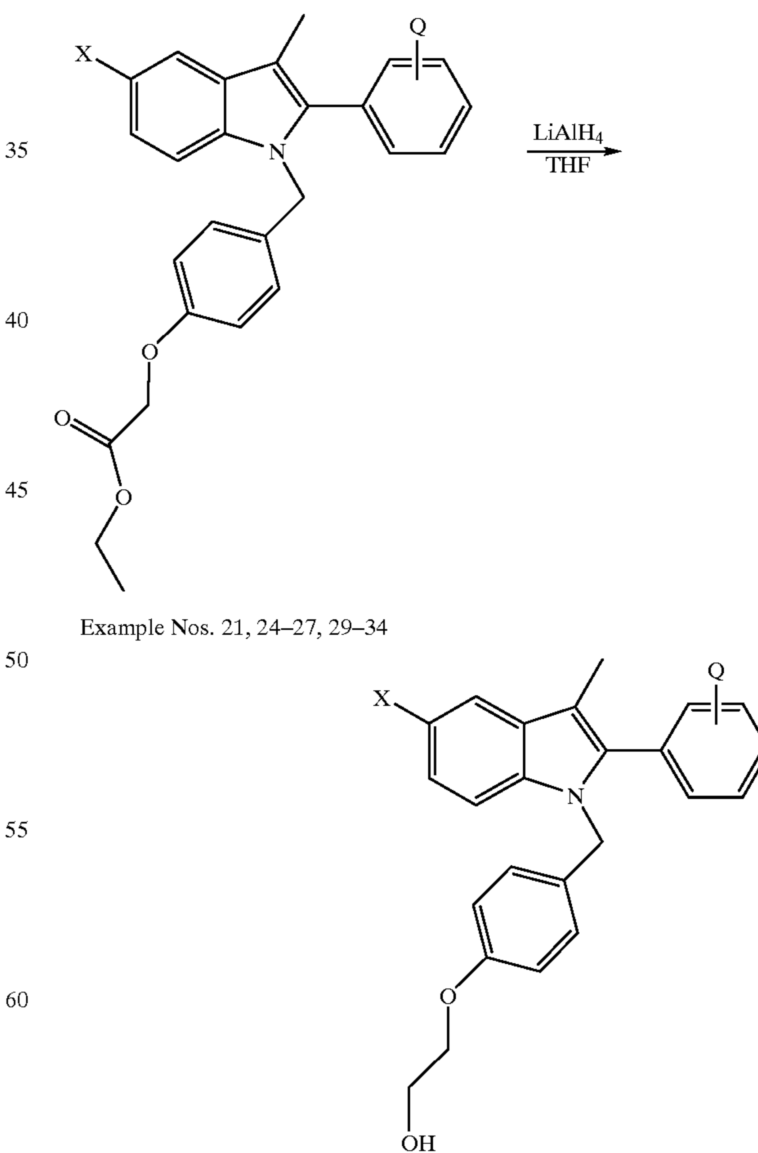
Scheme 10
