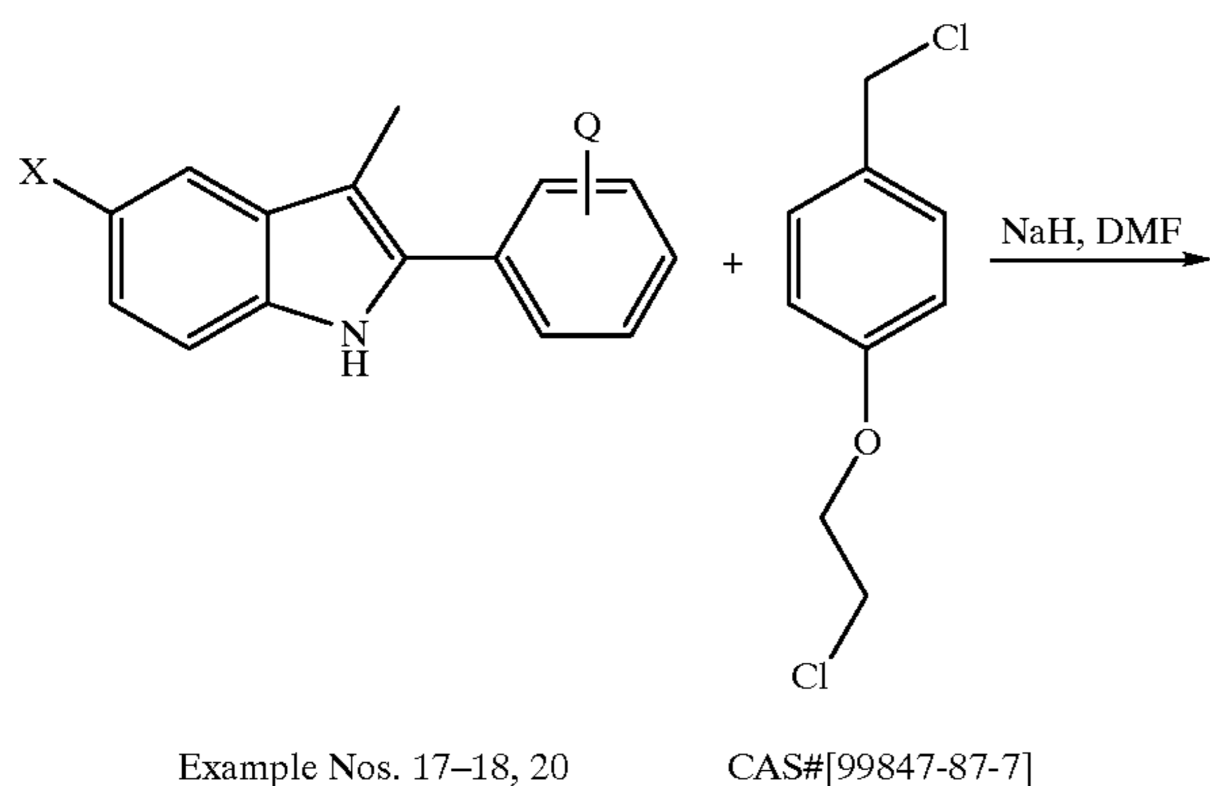
Scheme 12
