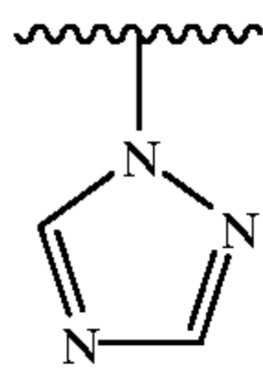
TRIAZOLE GROUP
