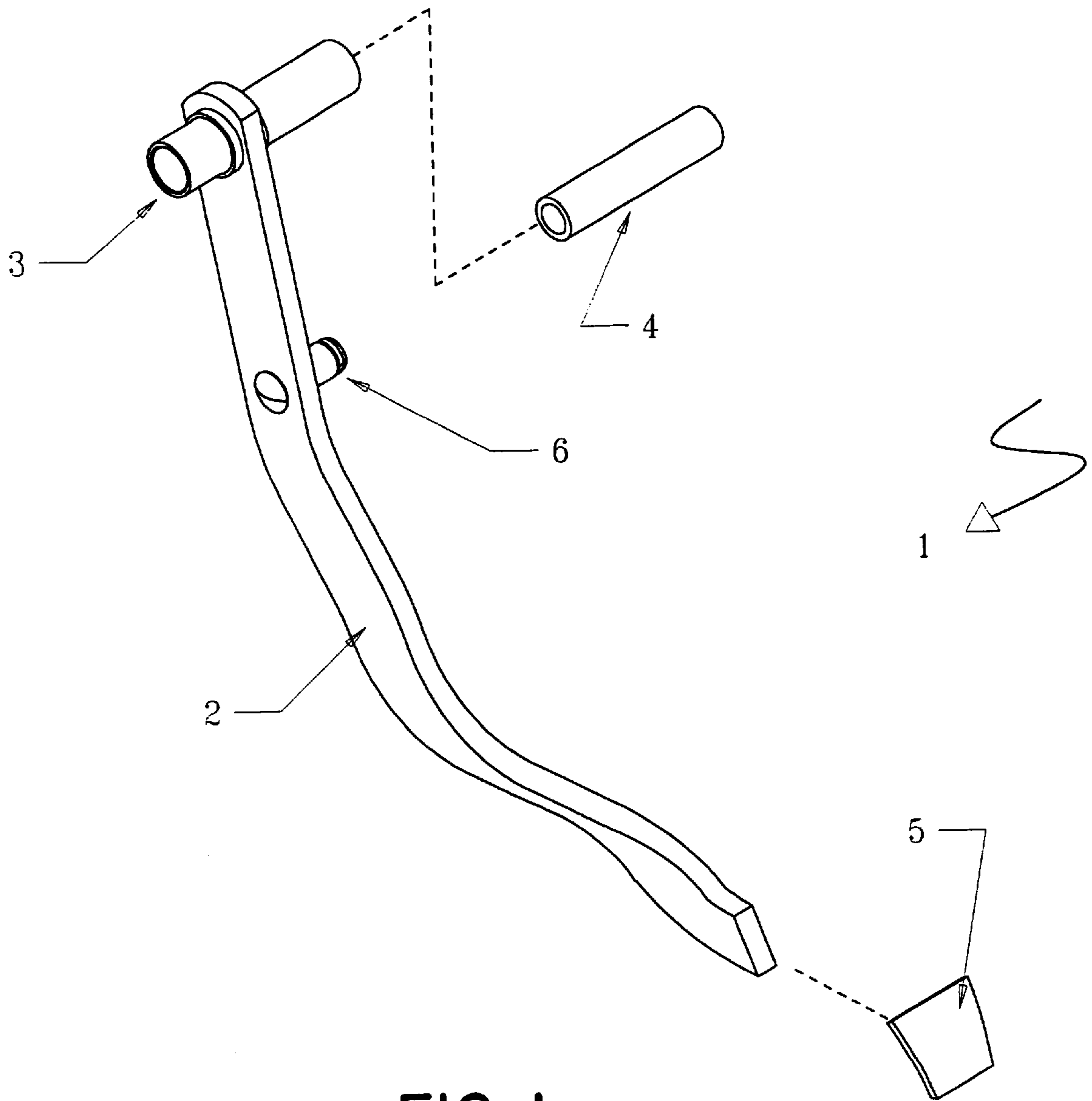
FIG. 1 (PRIOR ART)
