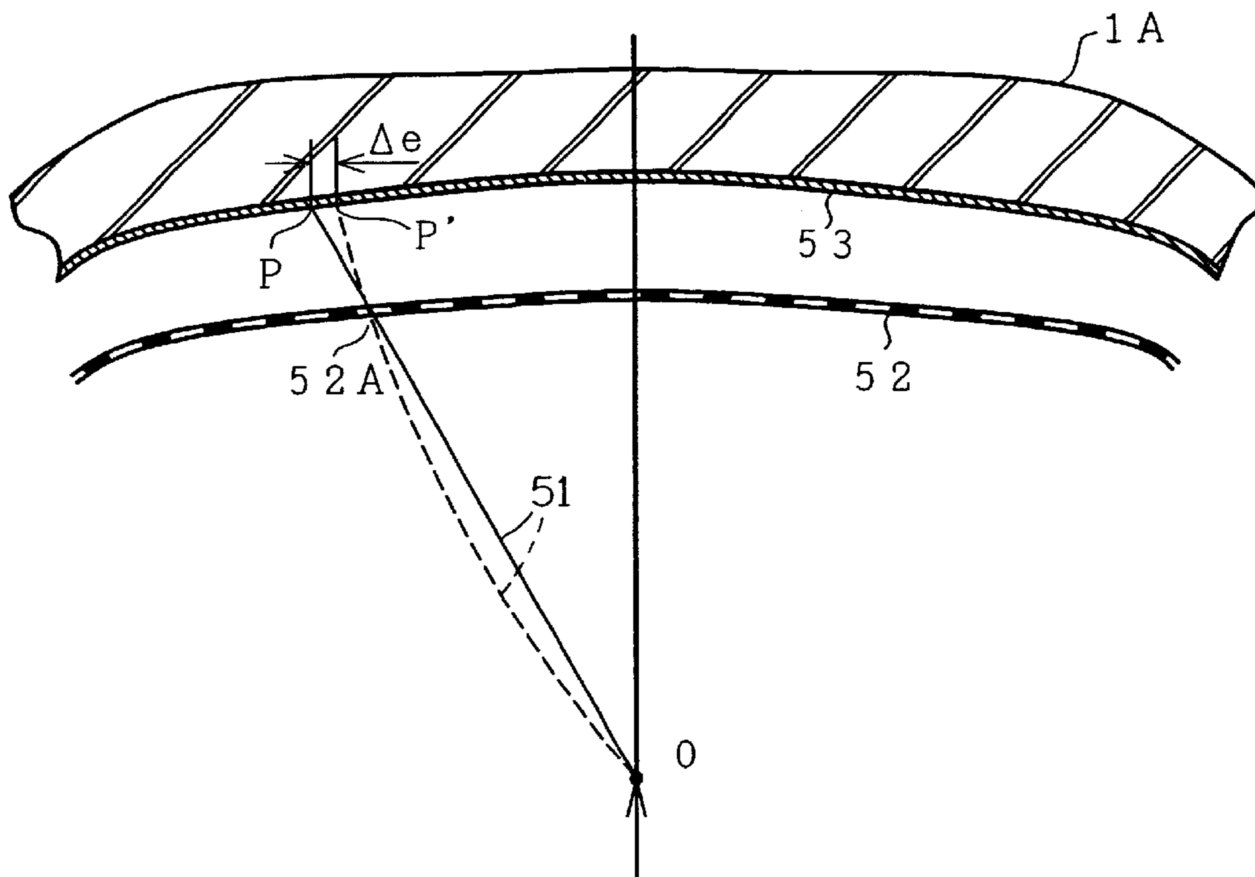
FIG. 5 (PRIOR ART)
