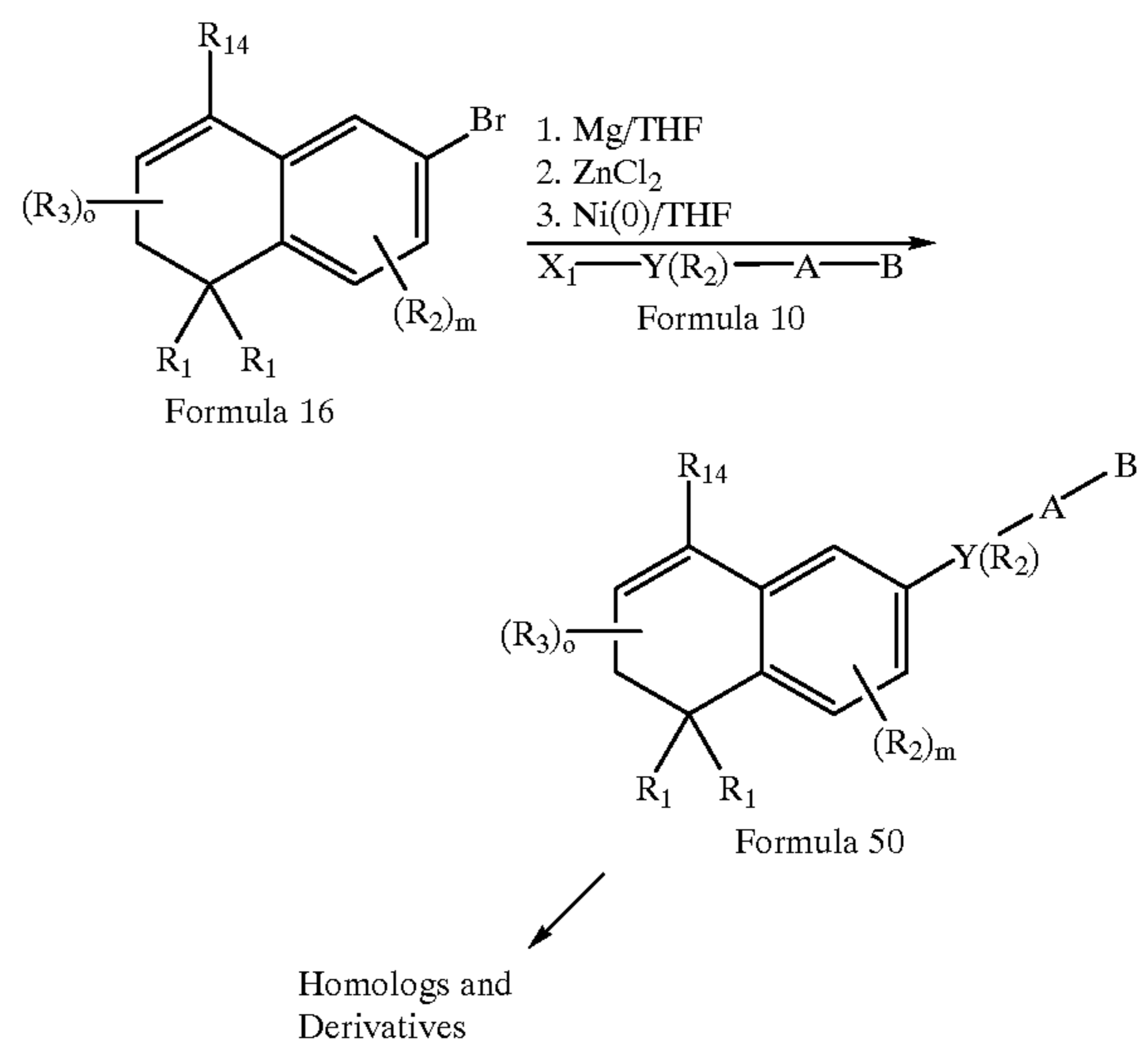
Reaction Scheme 7
