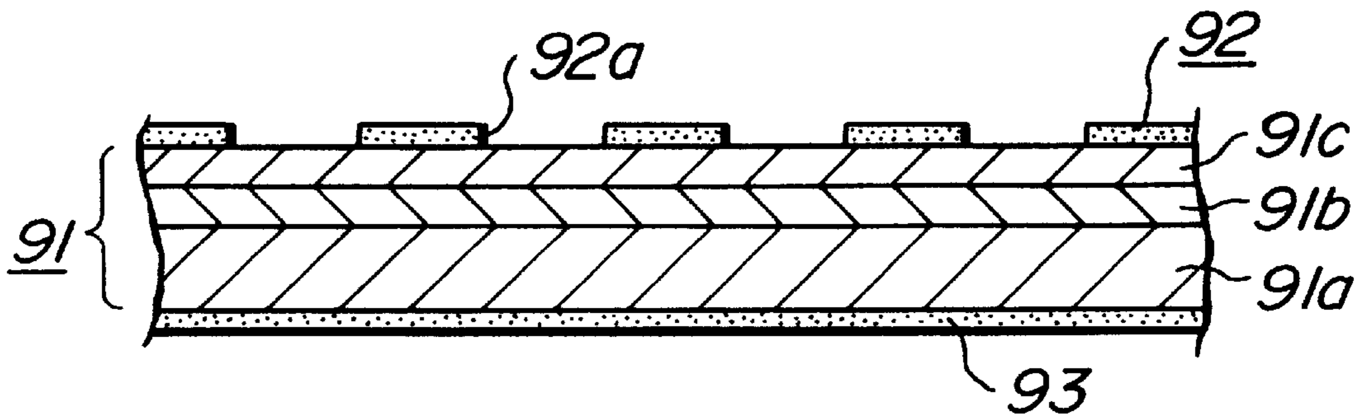
Fig. 1 Prior Art
