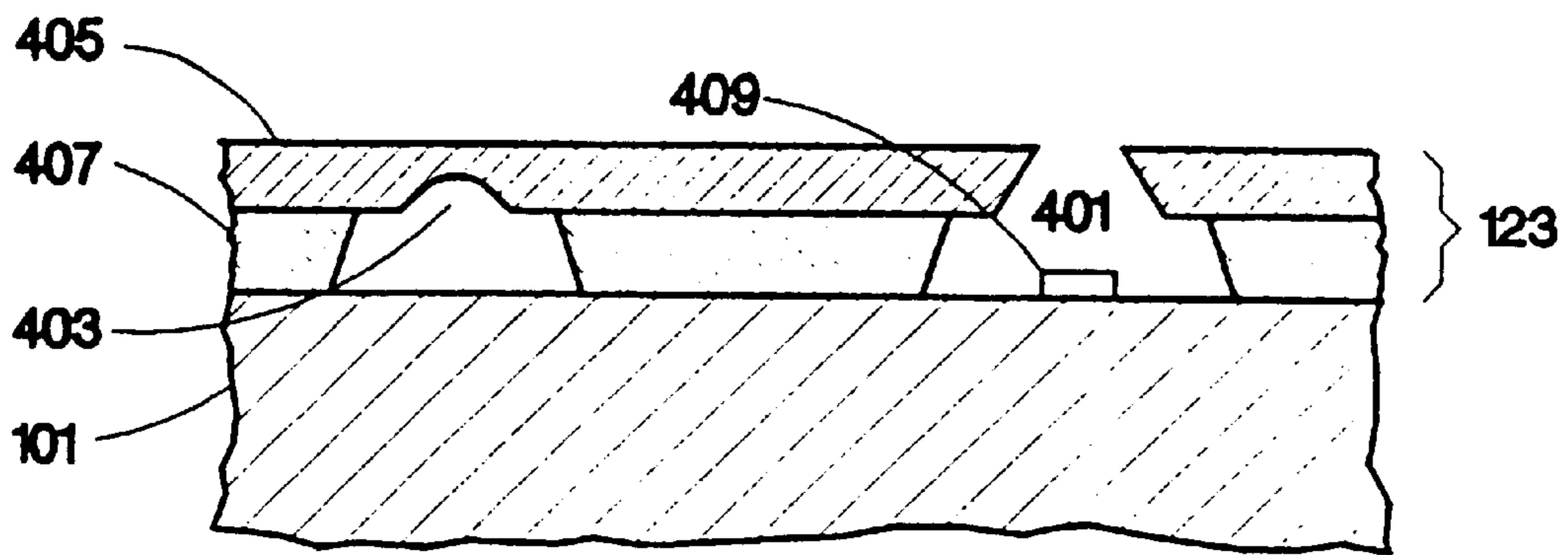
SECTION B-B
