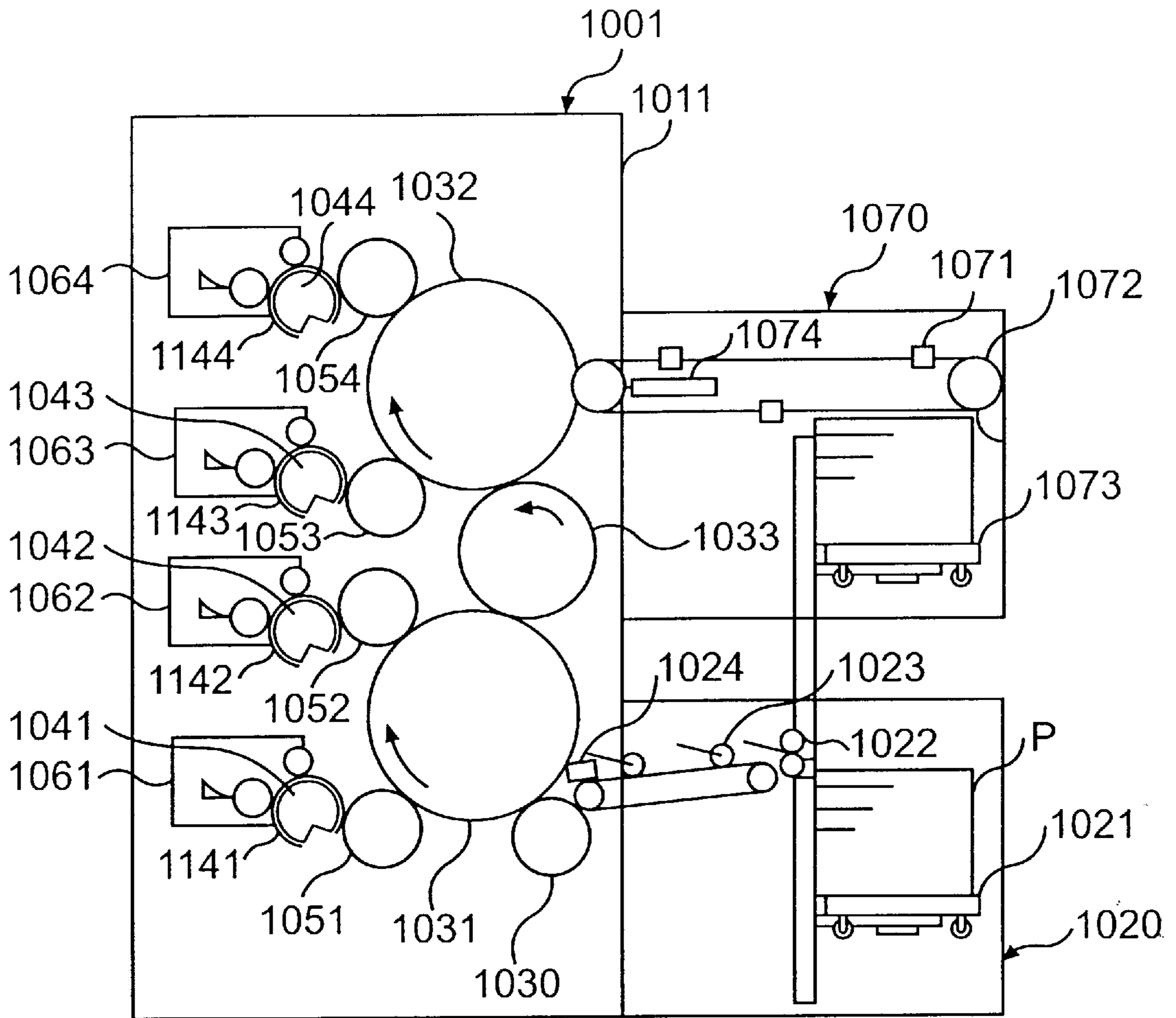
FIG. 3 PRIOR ART
