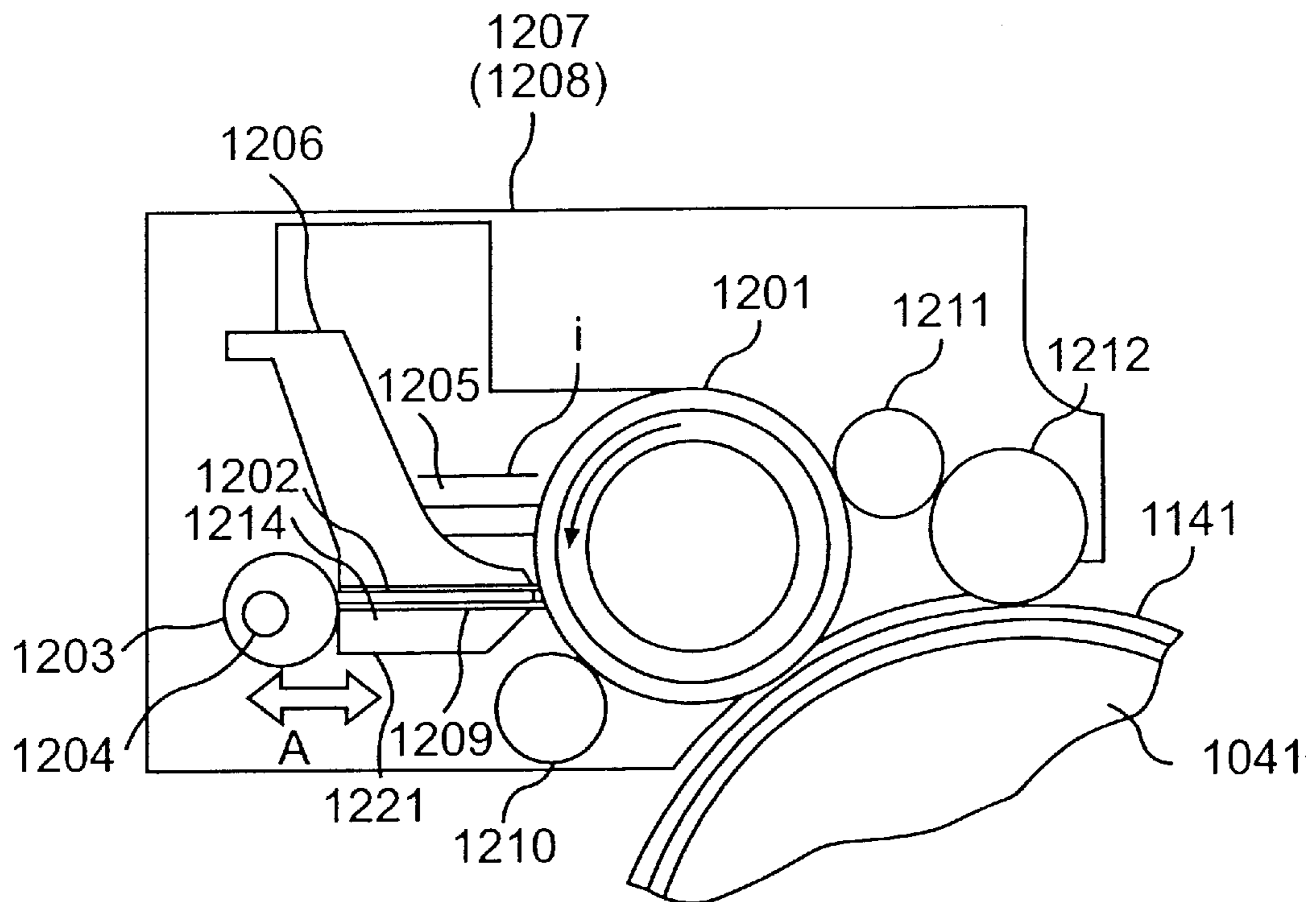
FIG. 4 PRIOR ART
