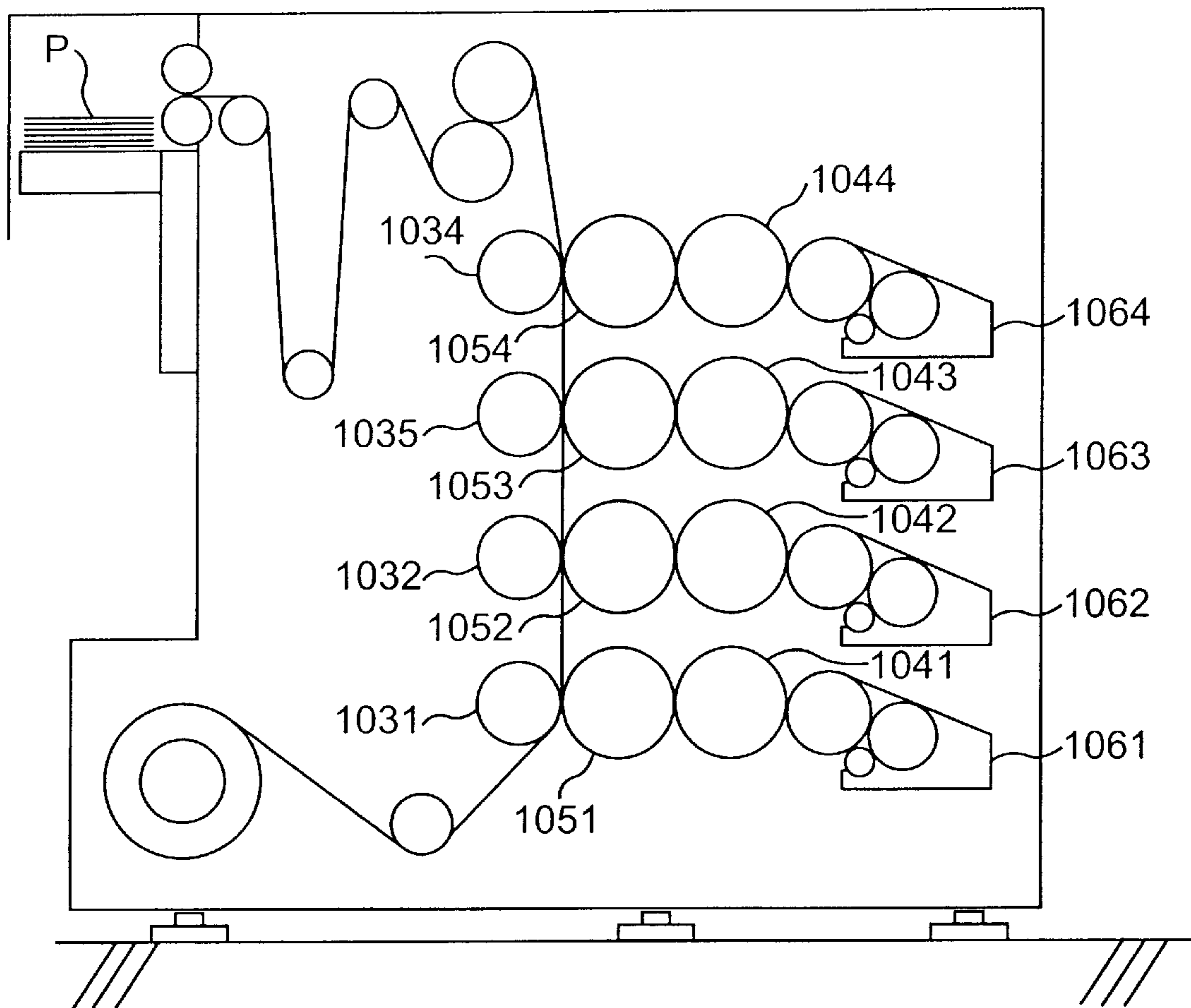
FIG. 30 PRIOR ART
