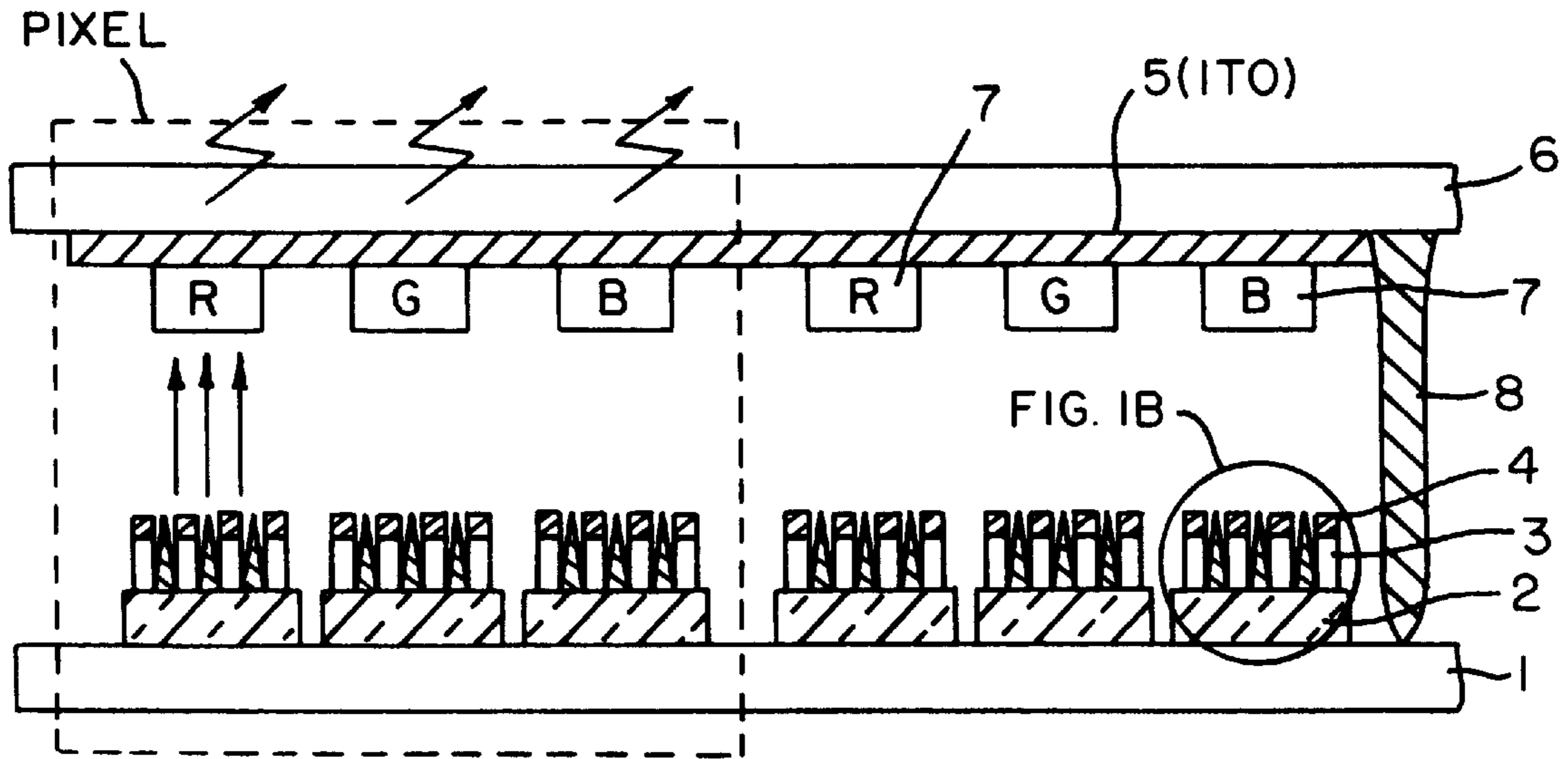
FIG. IA PRIOR ART
