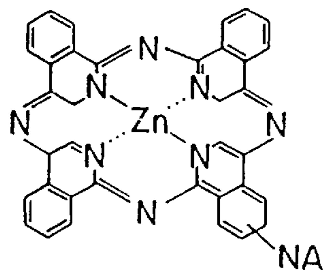
Zinc Phthalocyanine
