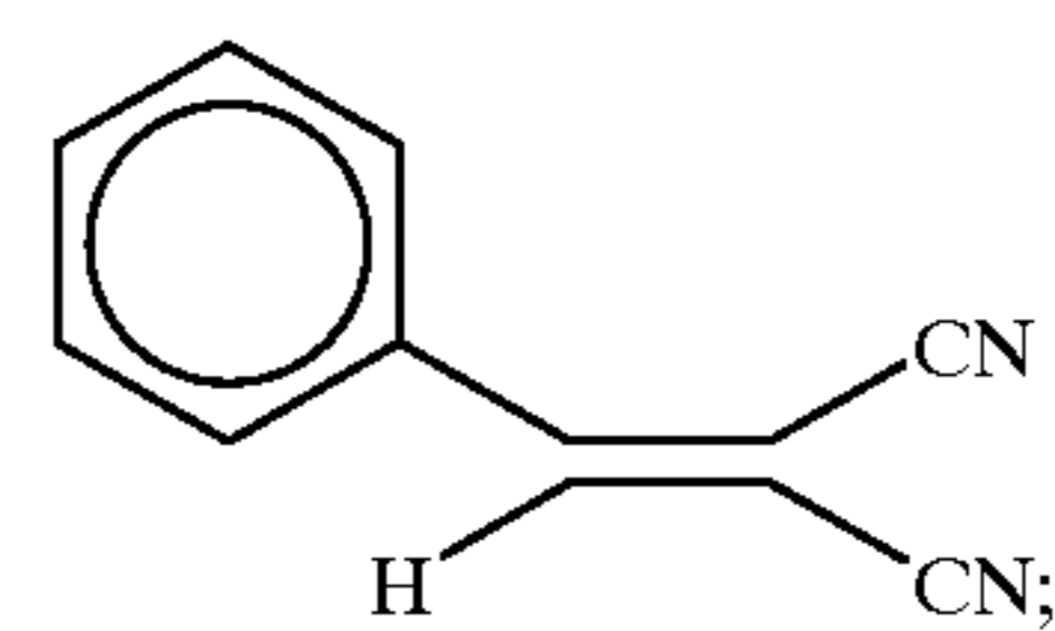
benzylidene malonitrile
