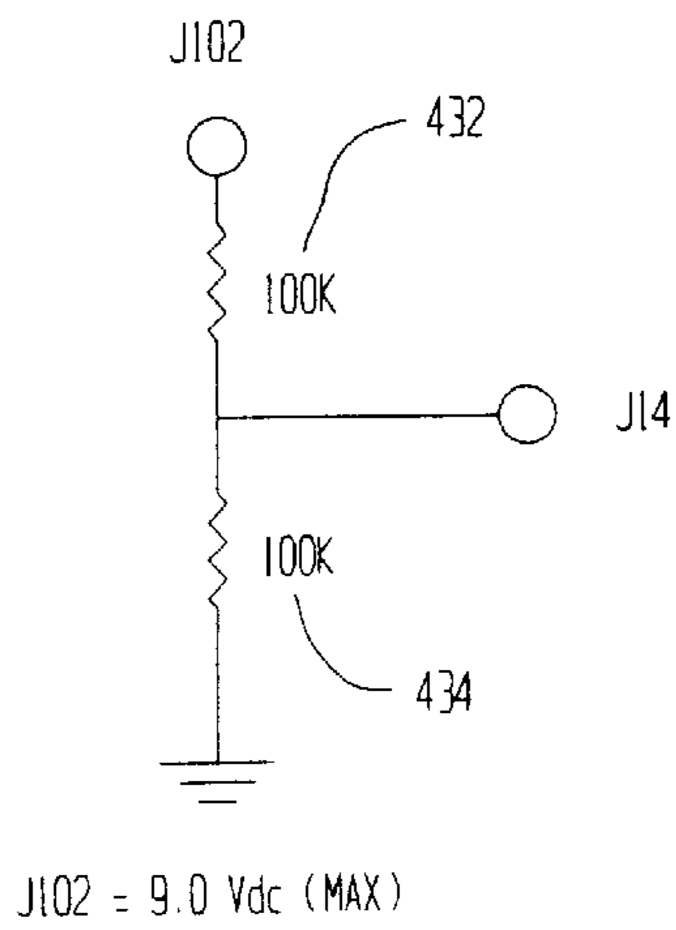
FIG. 32 CPU BATTERY VOLTAGE 430
