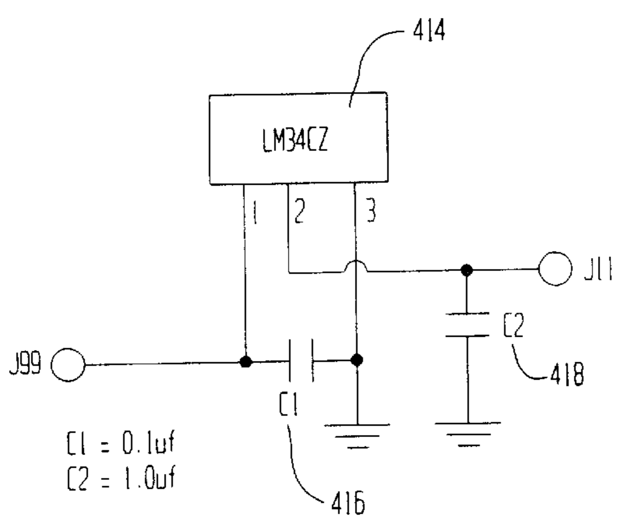
FIG. 30 TEMPERATURE SENSOR: LM34CZ (-40°F TO +230°F) 412
