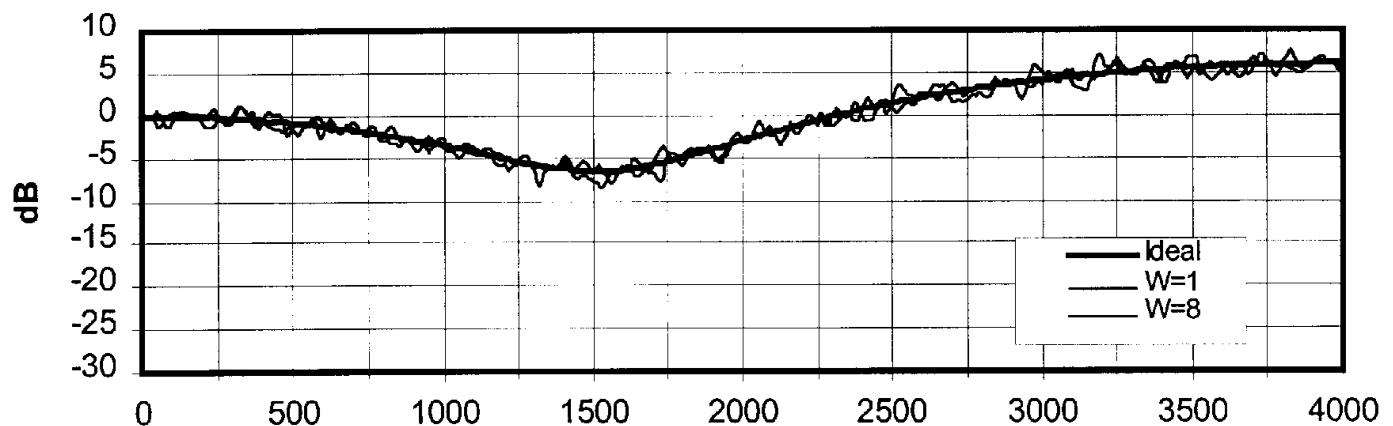
Figure 3d. Test D, ODD, Linear Values
