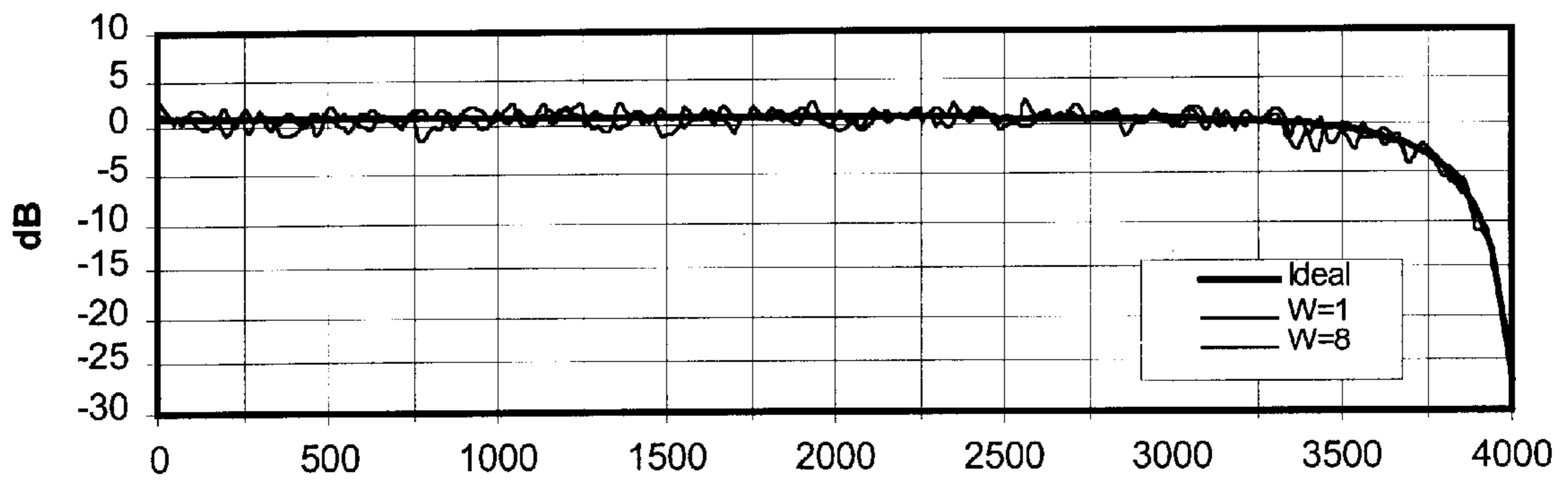
Figure 3b. Test B, LPF, Linear Values
