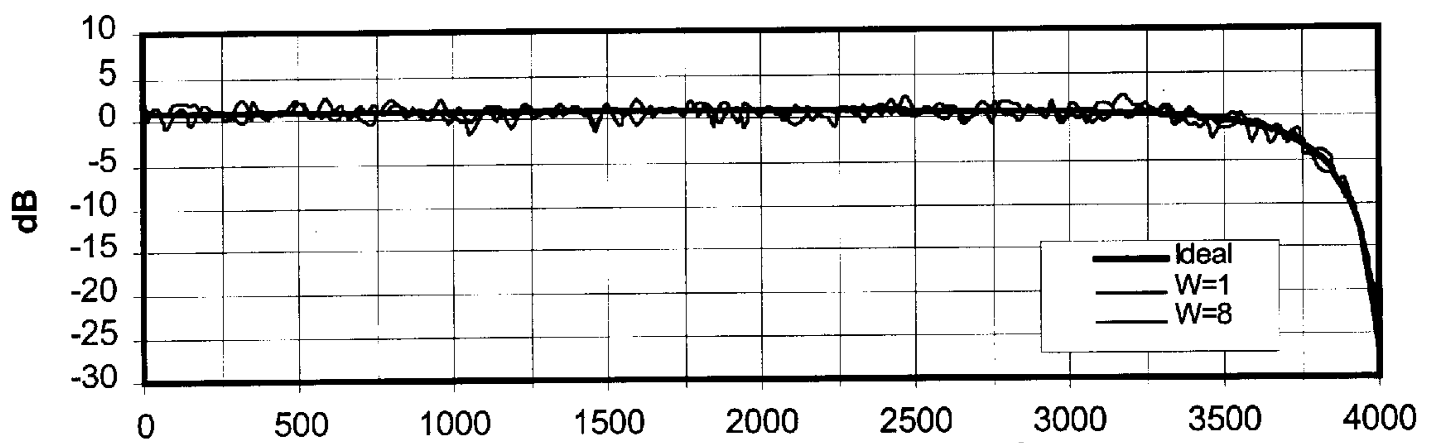
Figure 4b. Test B, LPF, PCM Values
