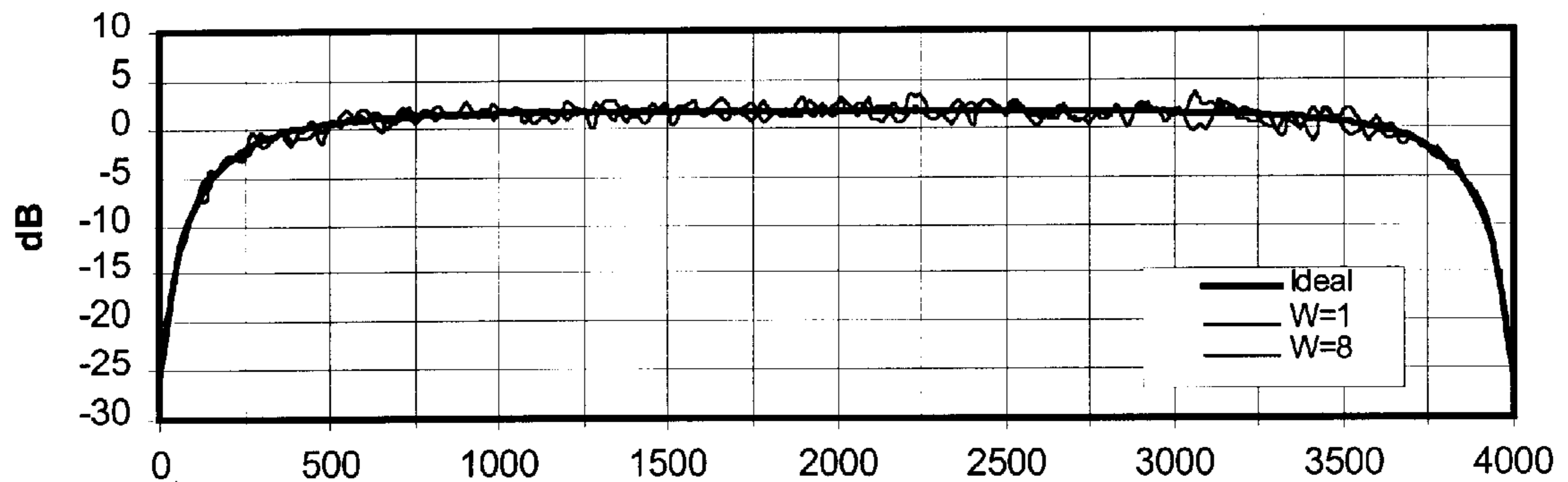
Figure 3c. Test C, BPF, Linear Values
