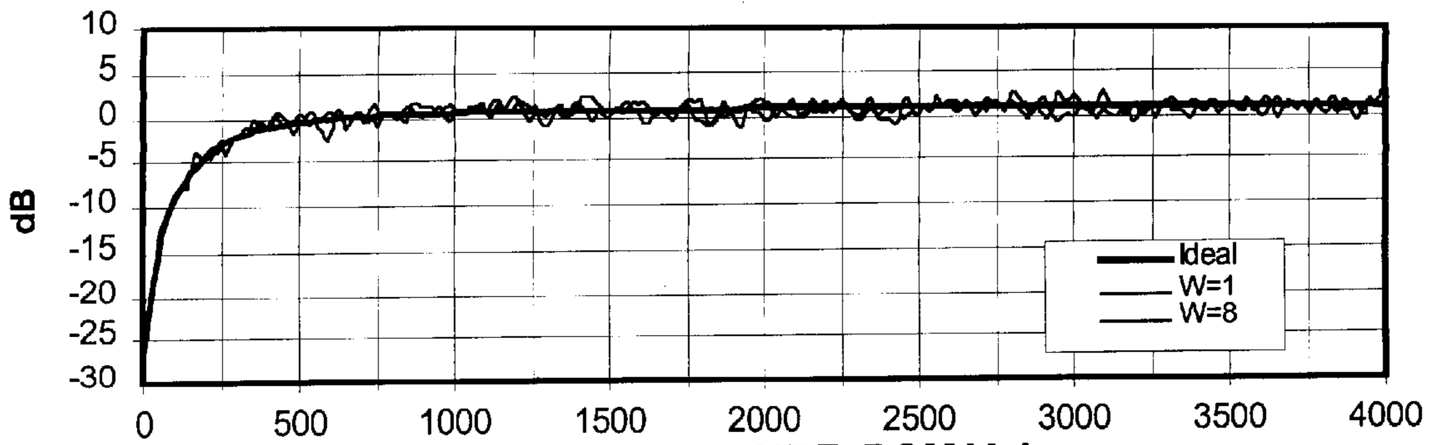
Figure 4a. Test A, HPF, PCM Values
