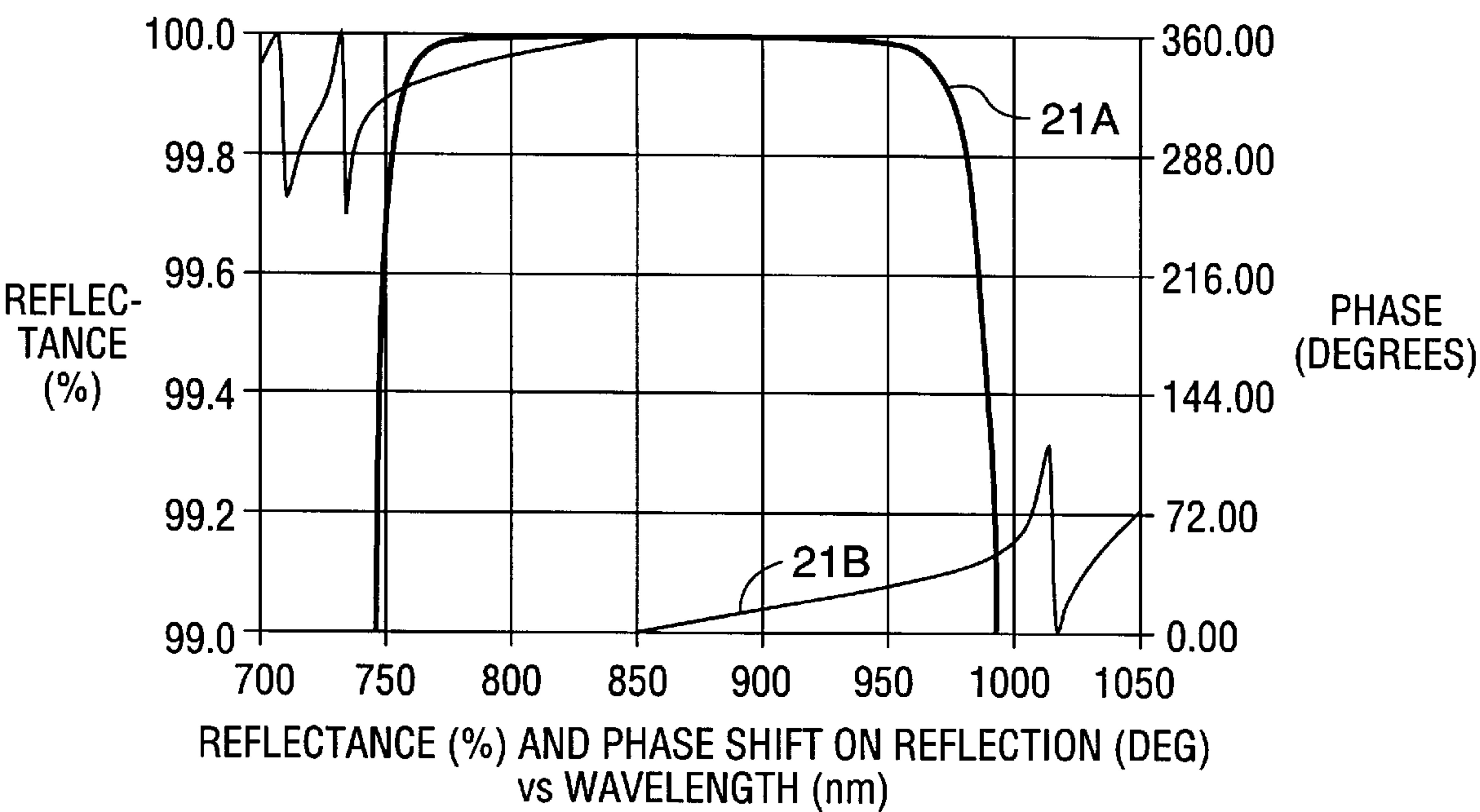
FIG. 24 (PRIOR ART)
