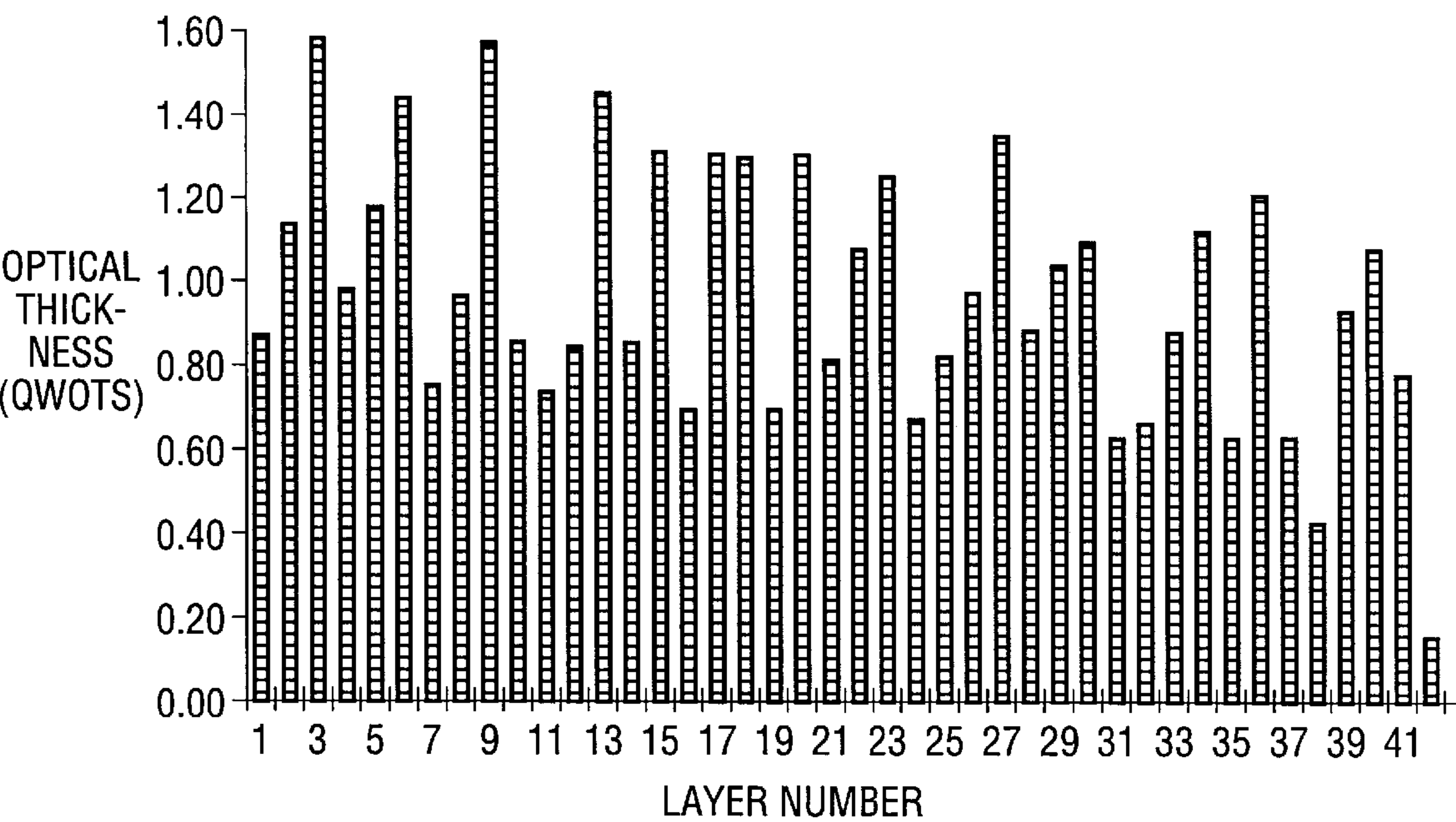
FIG. 1 (PRIOR ART)
