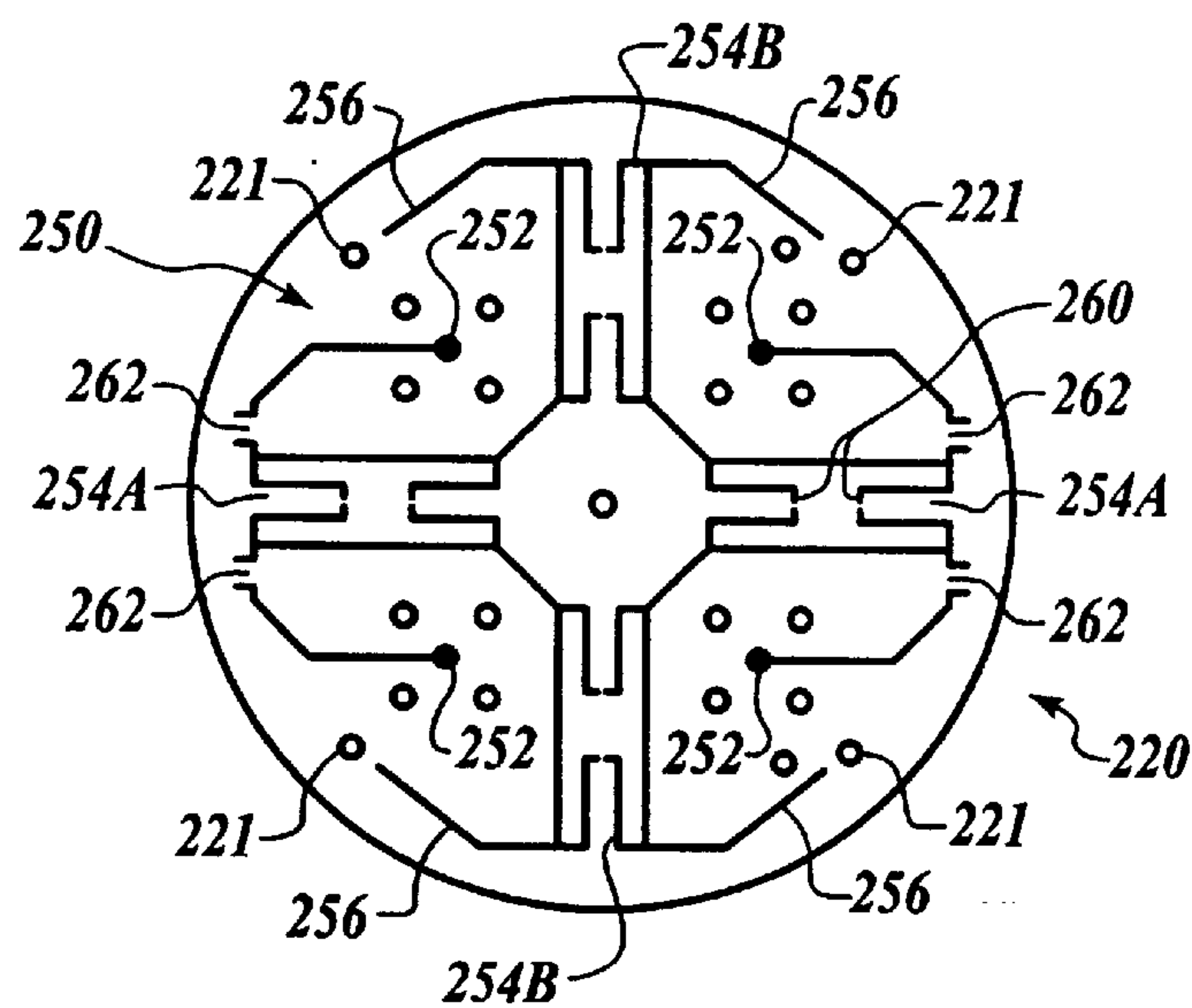
Fig. 11 (PRIOR ART)
