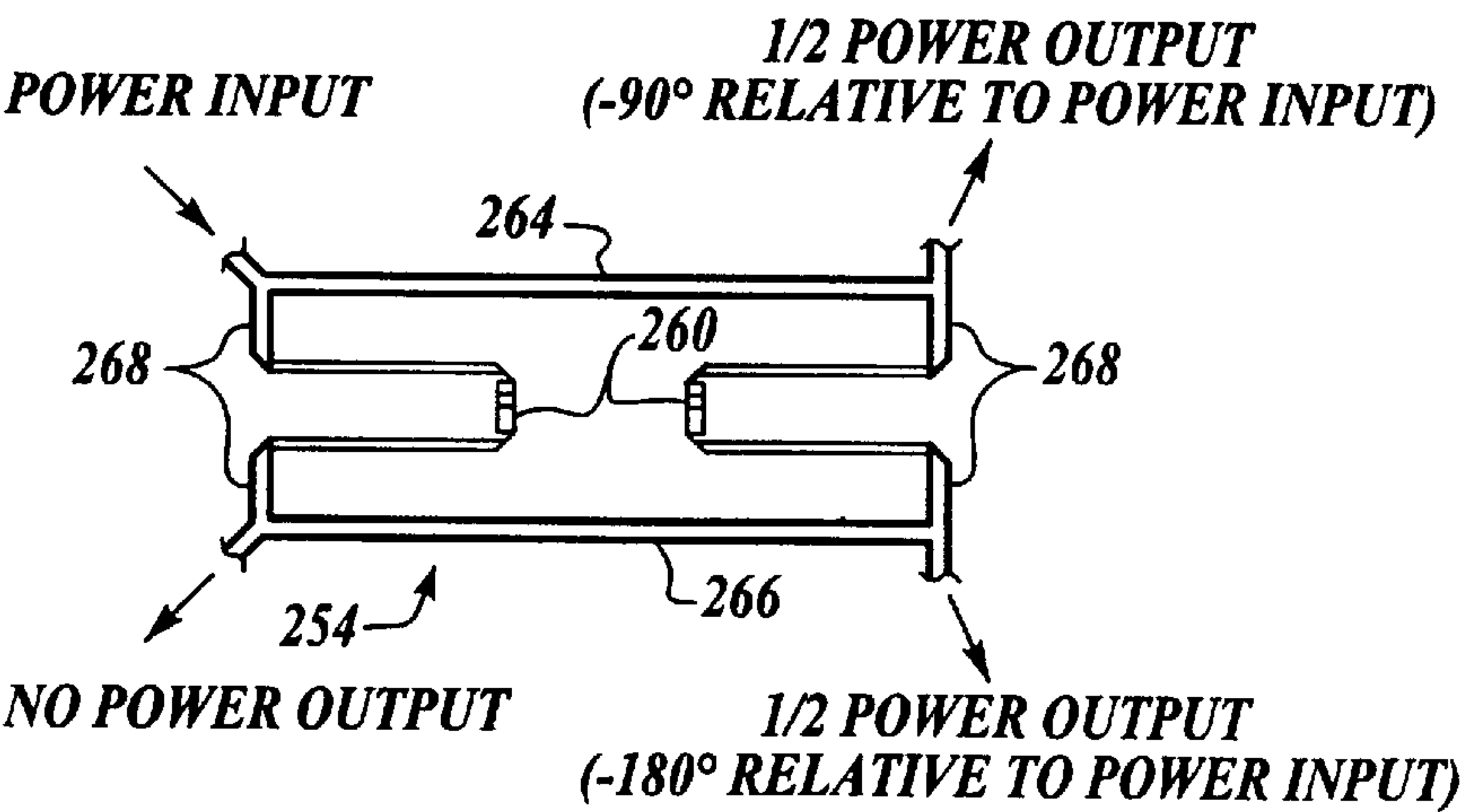
Fig. 12 (PRIOR ART)
