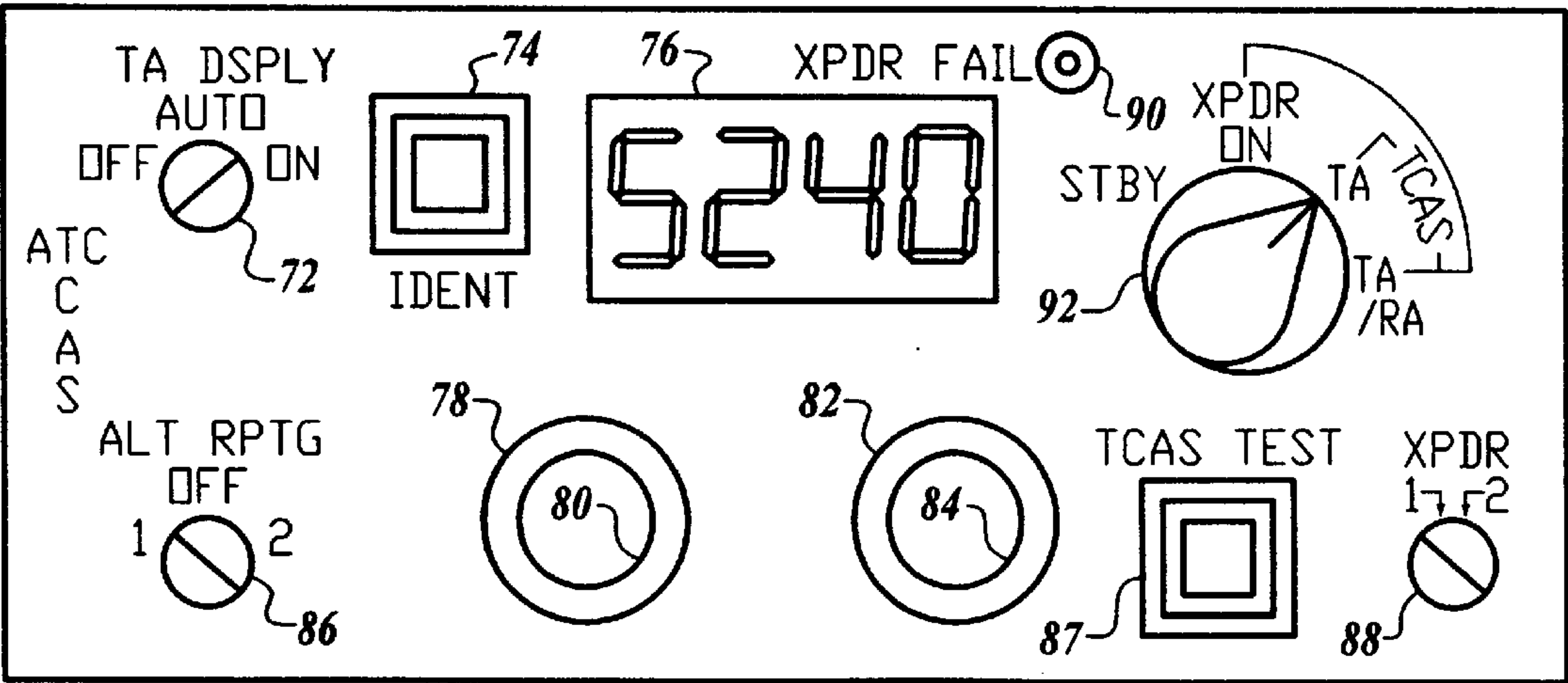
Fig. 4 (PRIOR ART)
