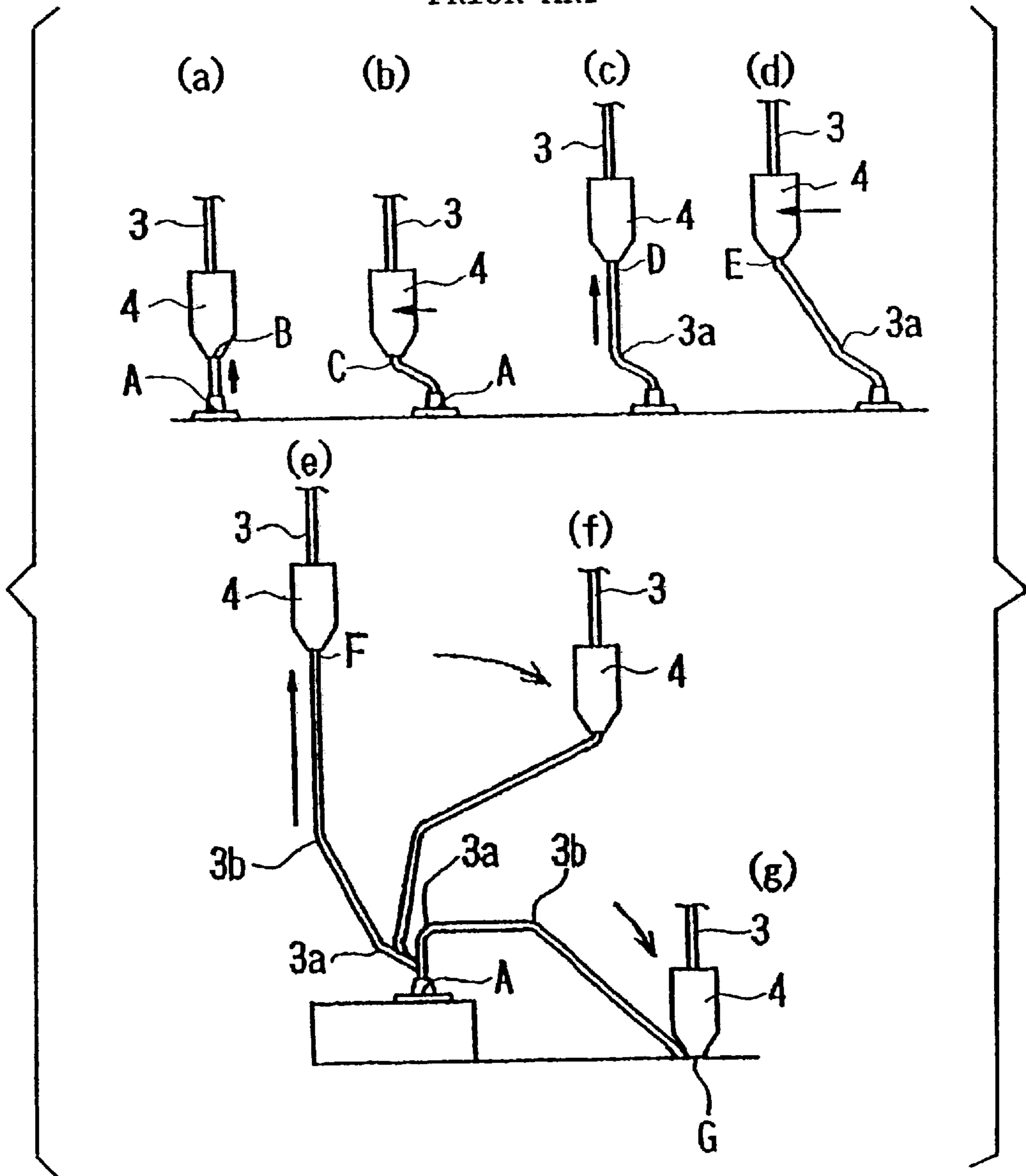
FIG. 4 PRIOR ART
