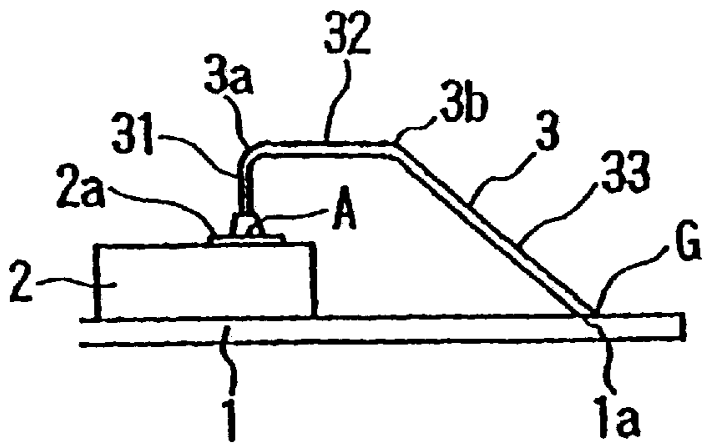
FIG. 4 PRIOR ART
