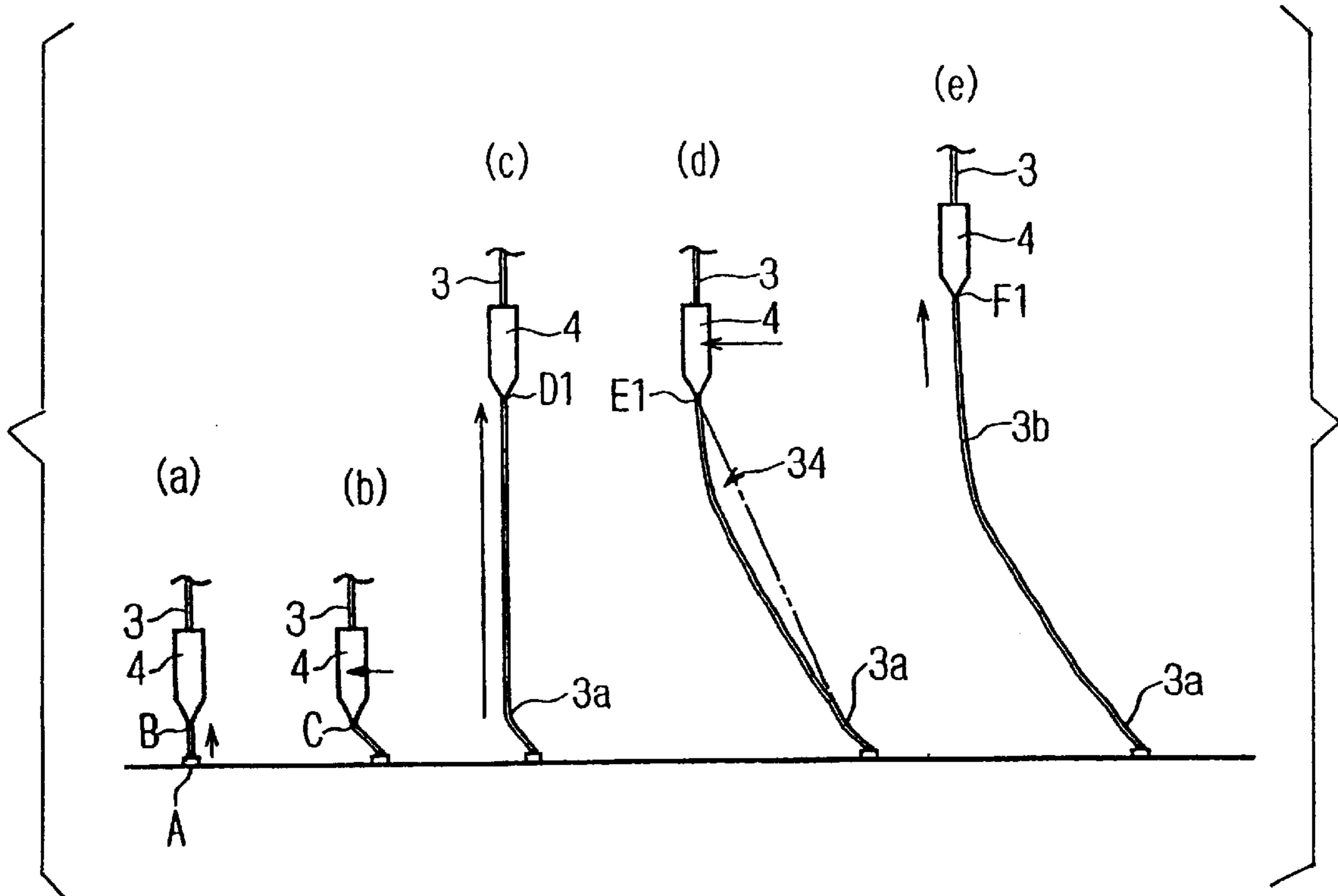
FIG. 7 PRIOR ART
