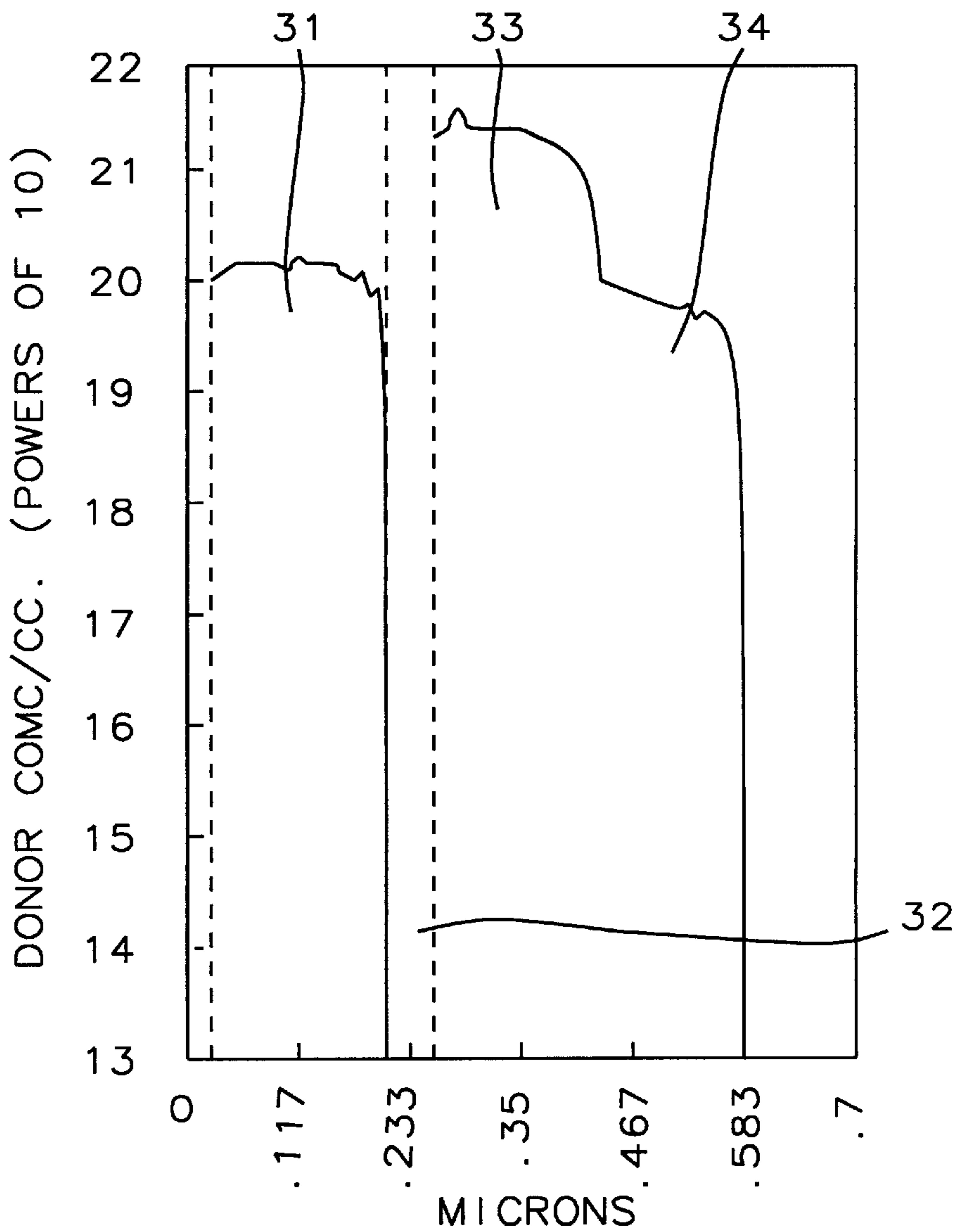
FIG. 3 - Prior Art
