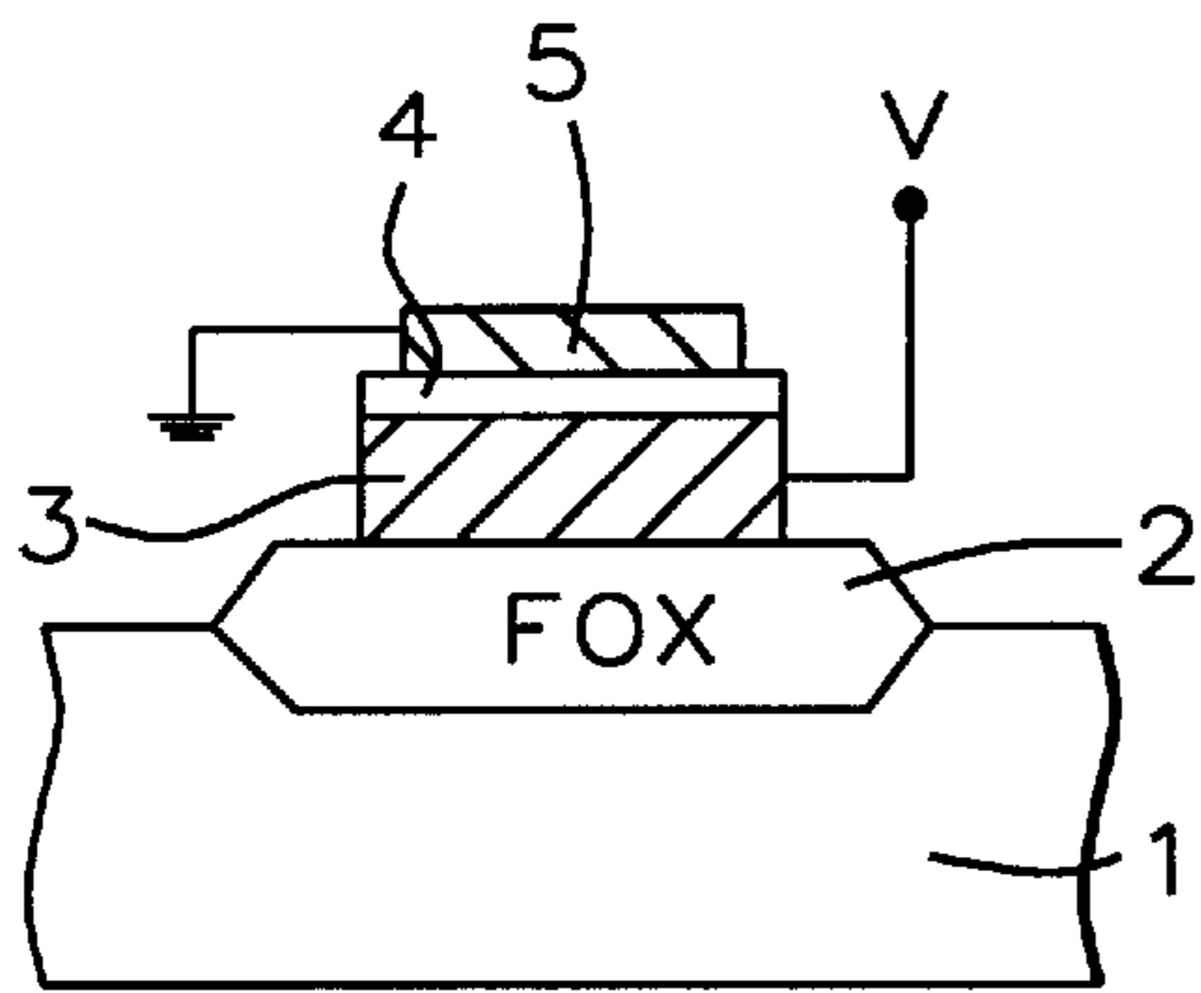
FIG. 4 - Prior Art
