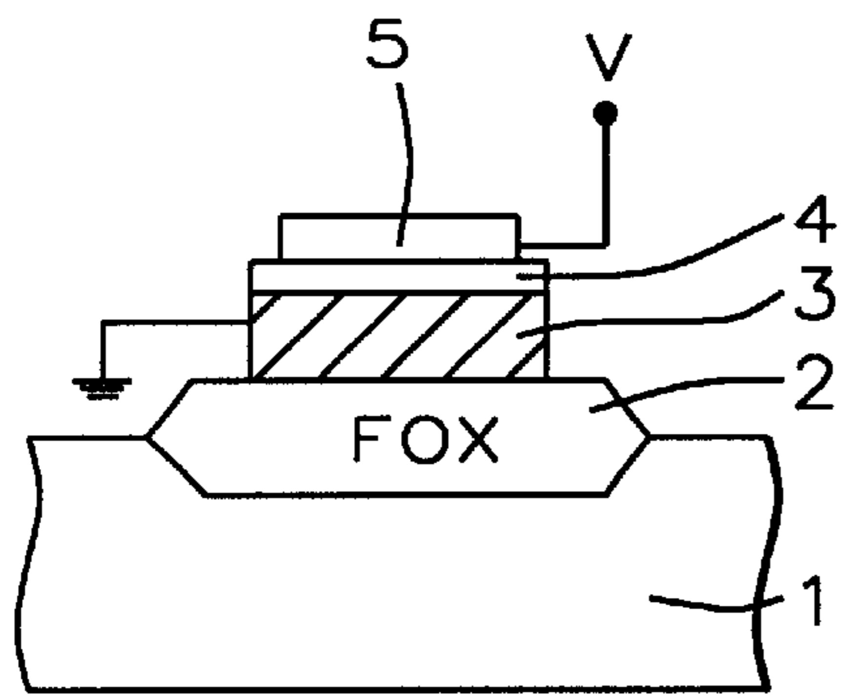
FIG. 1 - Prior Art
