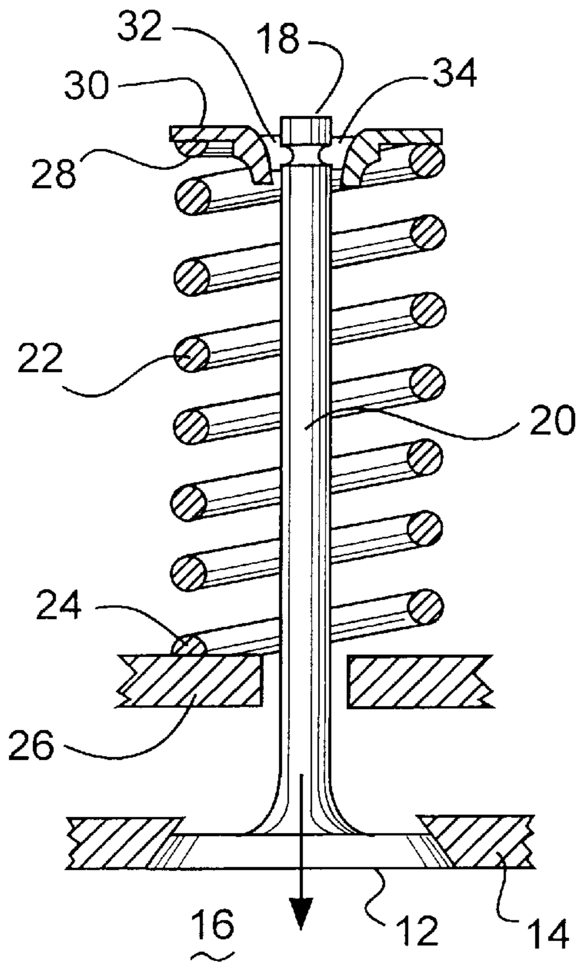
FIG. 1 (PRIOR ART)
