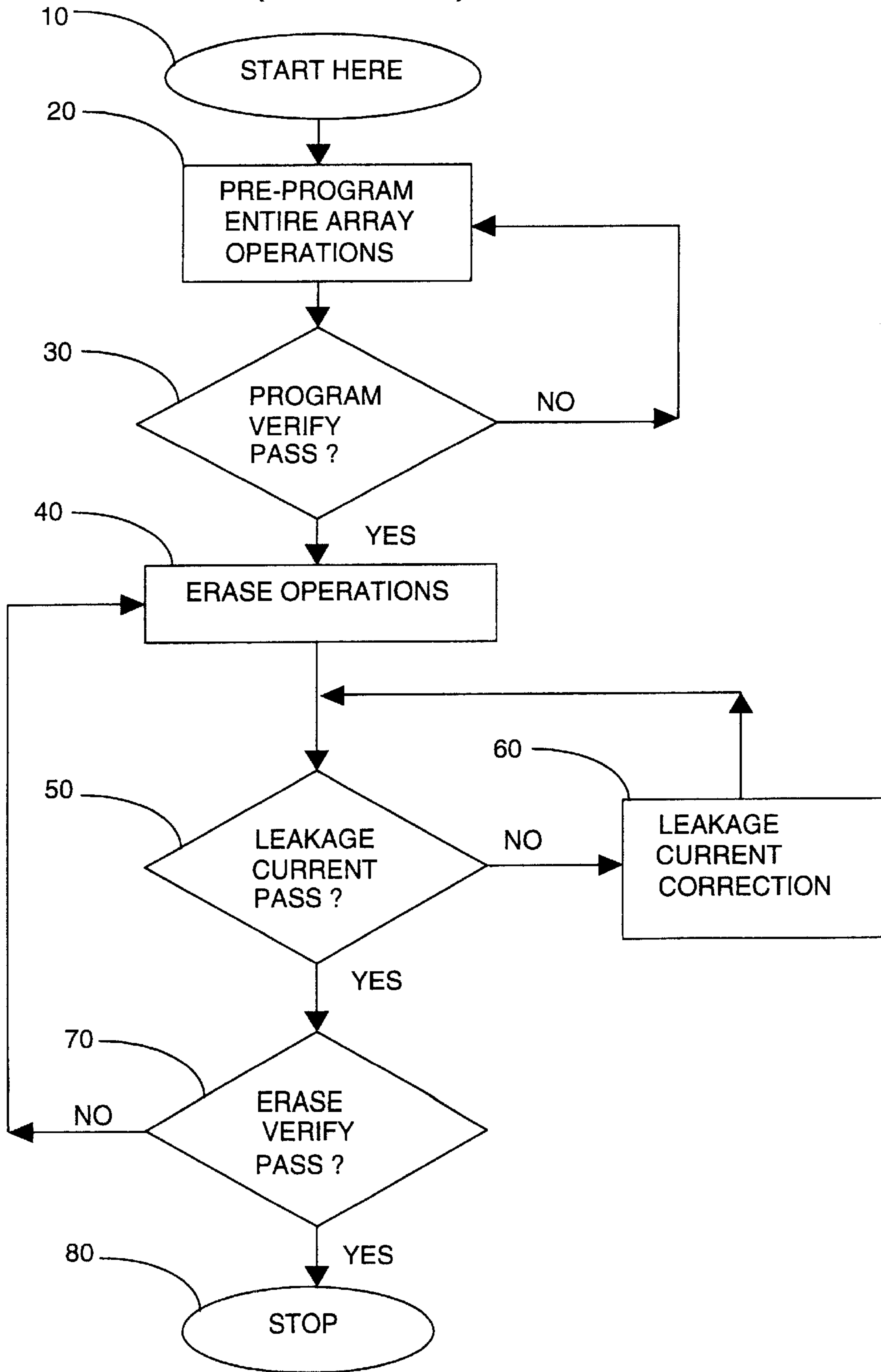
Fig. 1 (Prior Art)
