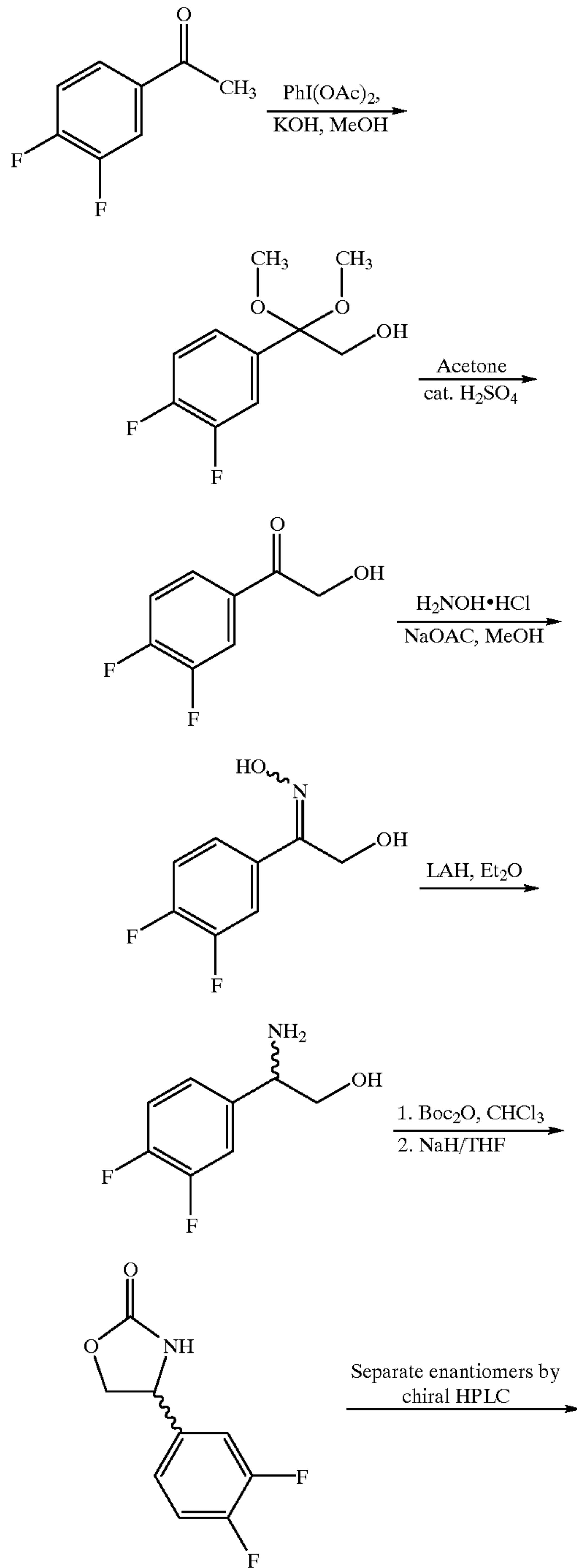
Scheme 2 Synthesis of Chiral Morpholinone Examples
