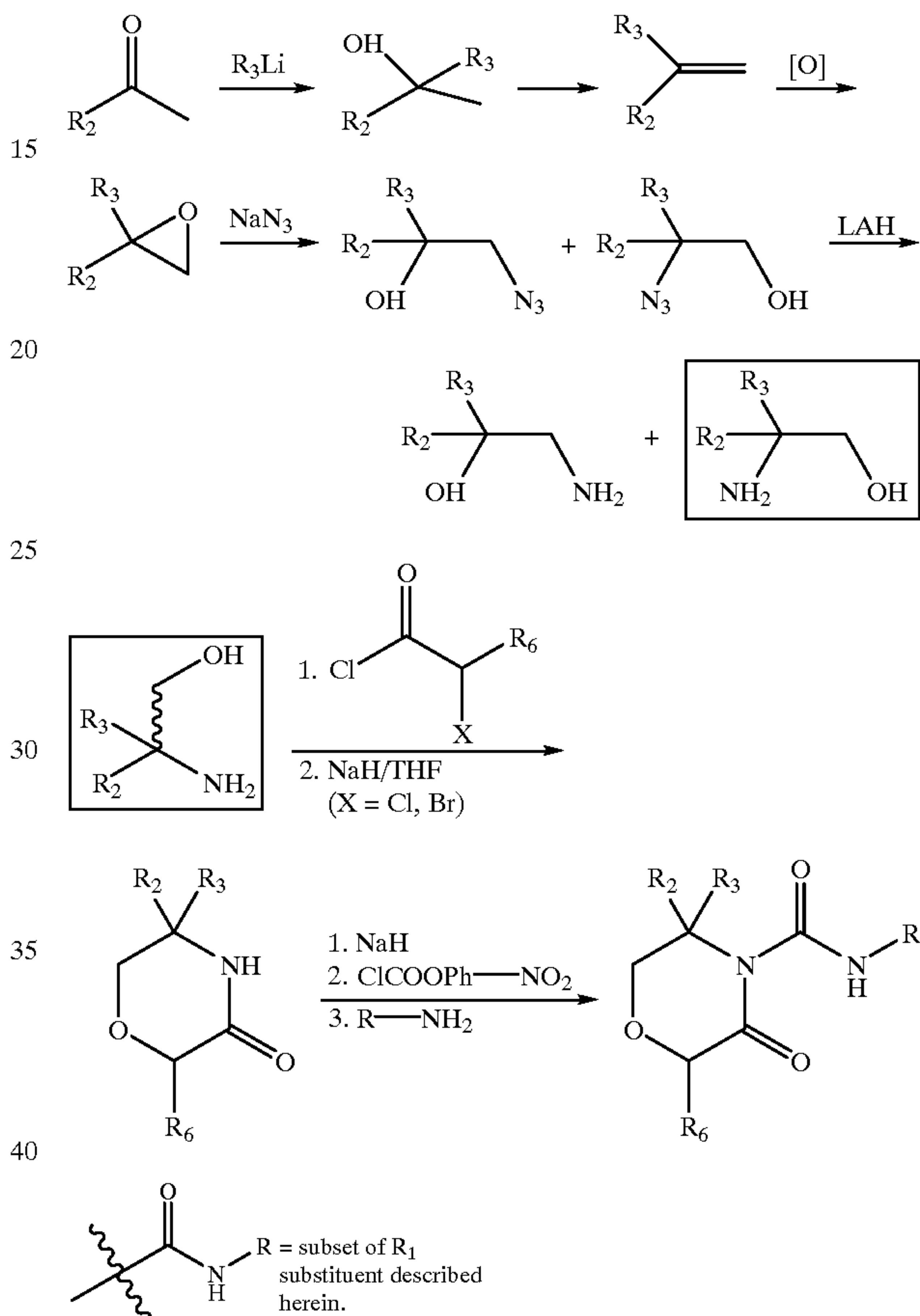
Scheme 9 General Synthesis of Substituted Morpholinones.
