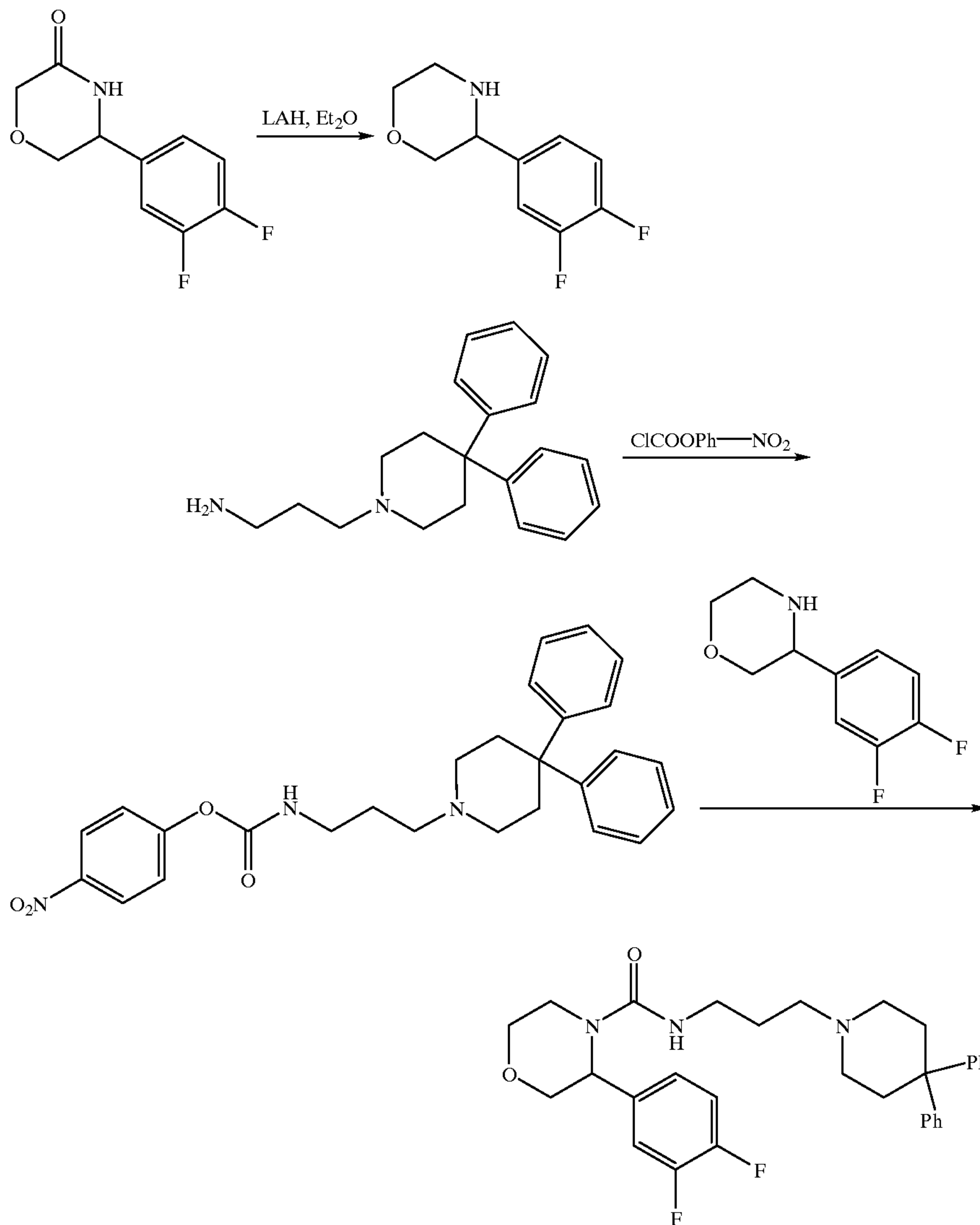
Scheme 6 Synthesis of Morpholine Example (Compound 21).
