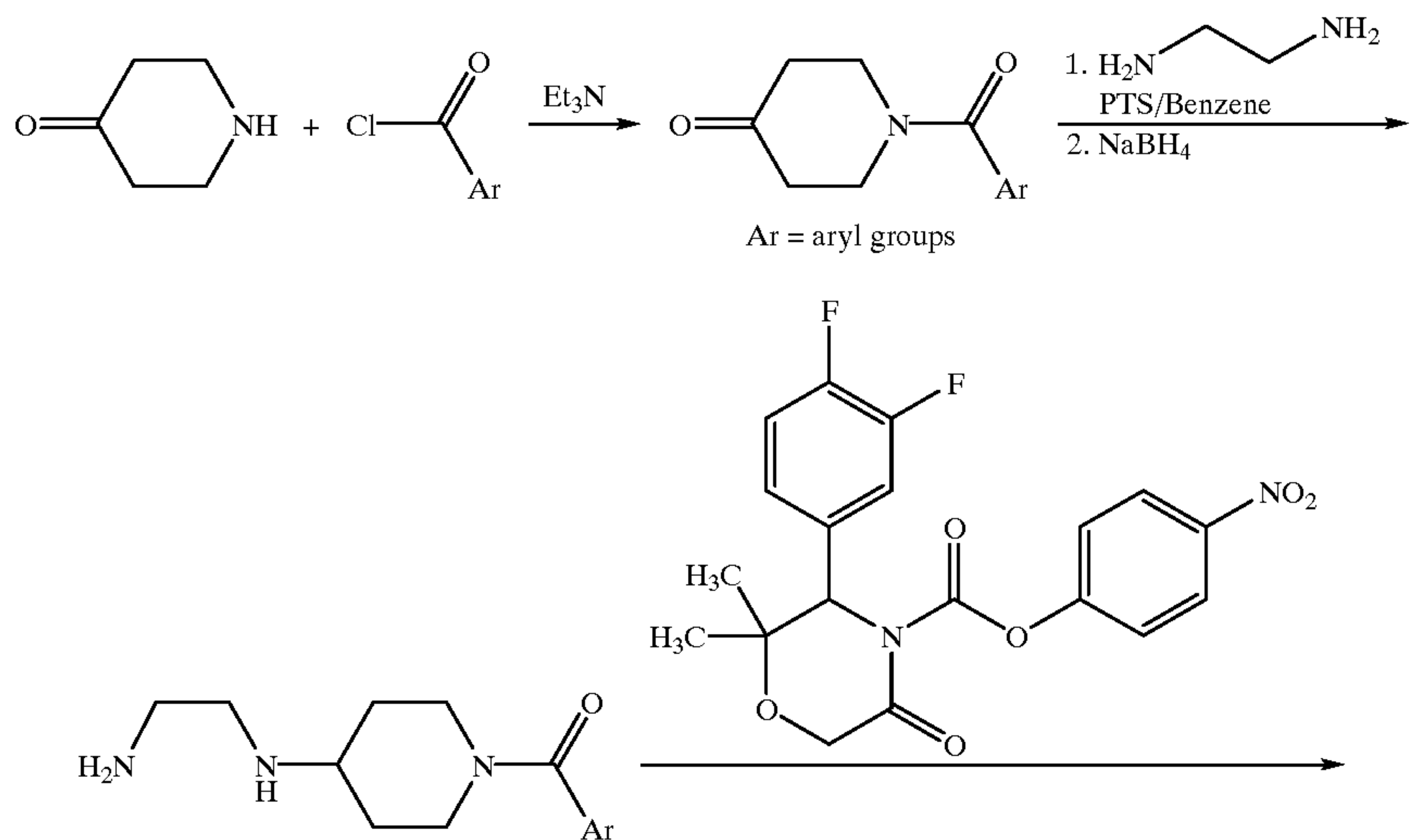
Scheme 5 Synthesis of Morpholinone Examples.
