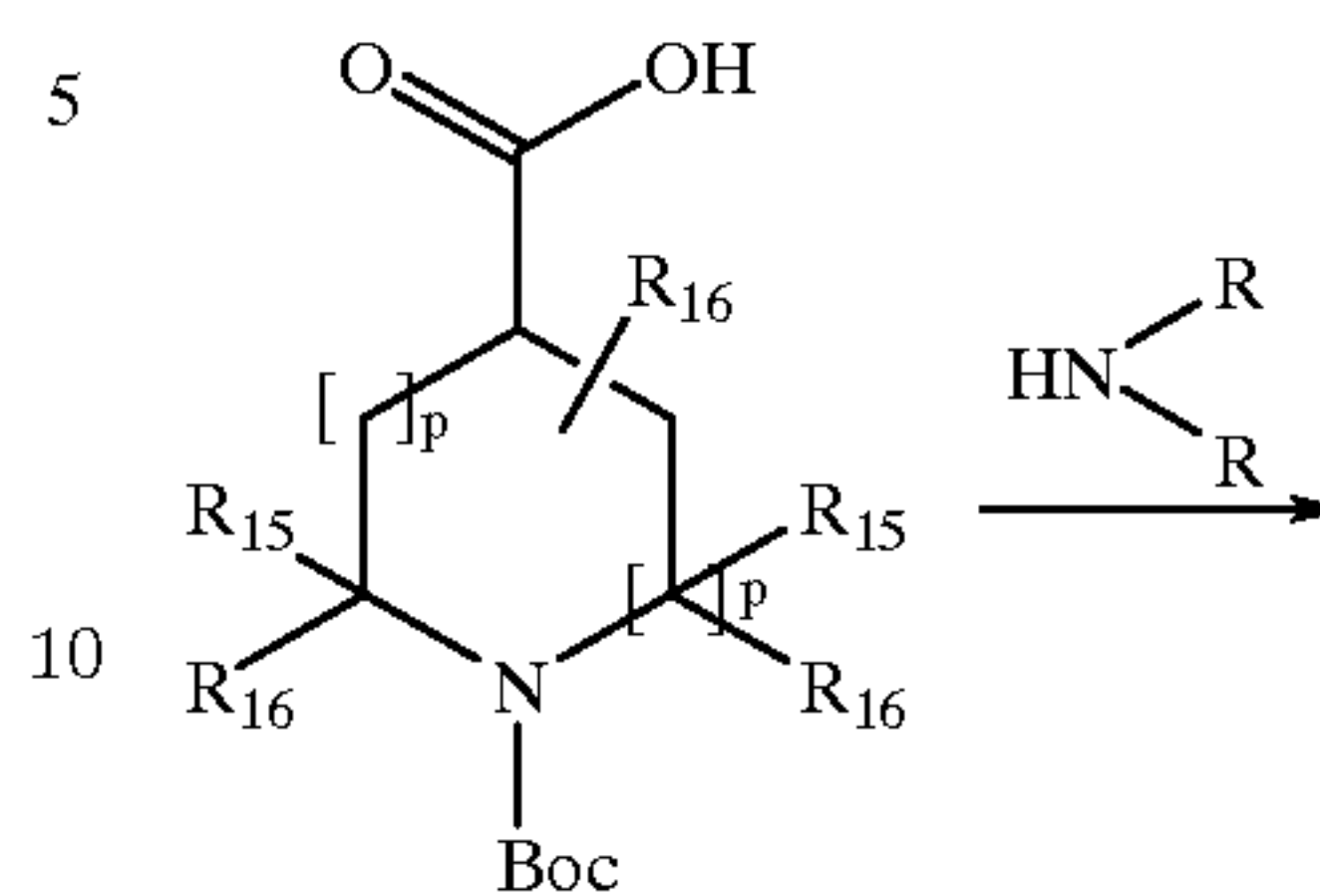
Scheme 21 General Synthesis of Compounds.
