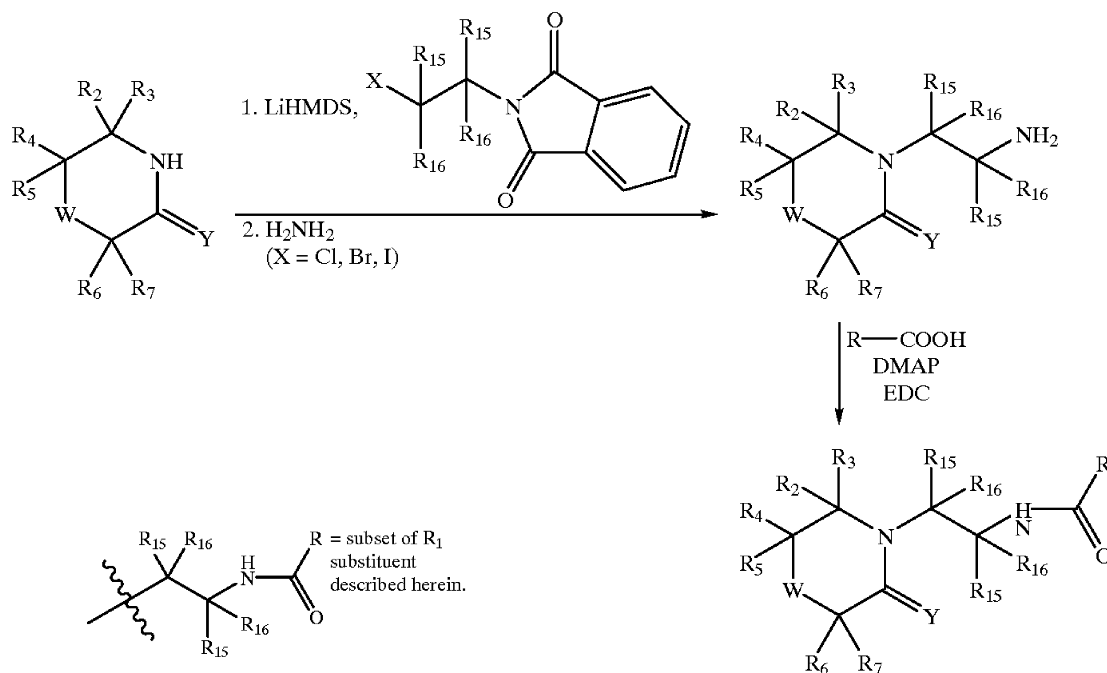
Scheme 17 General Synthesis of Compounds.
