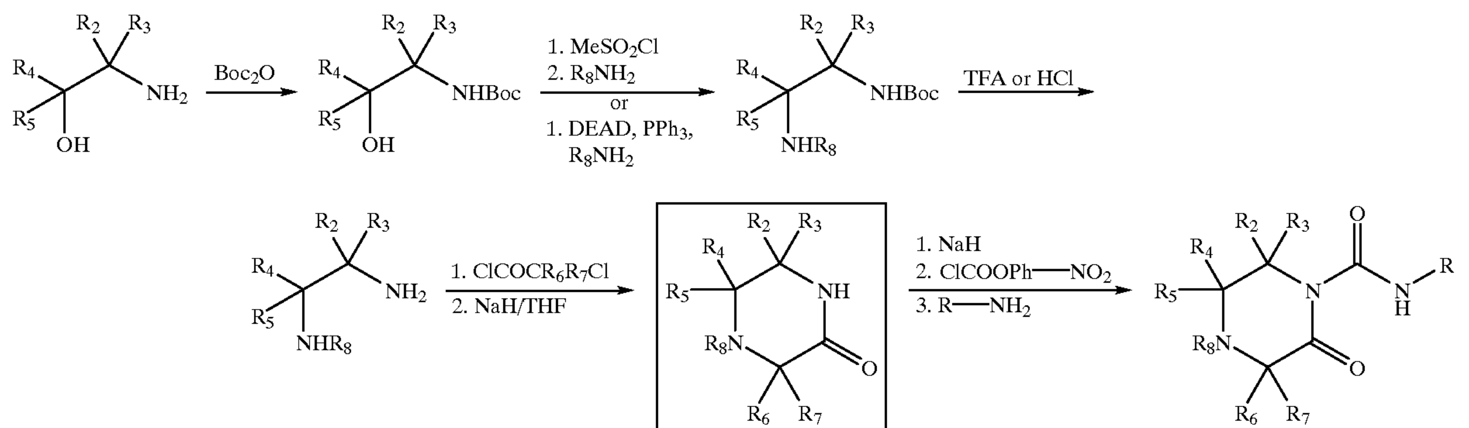
Scheme 13 General Synthesis of Piperizines and piperizinones.
