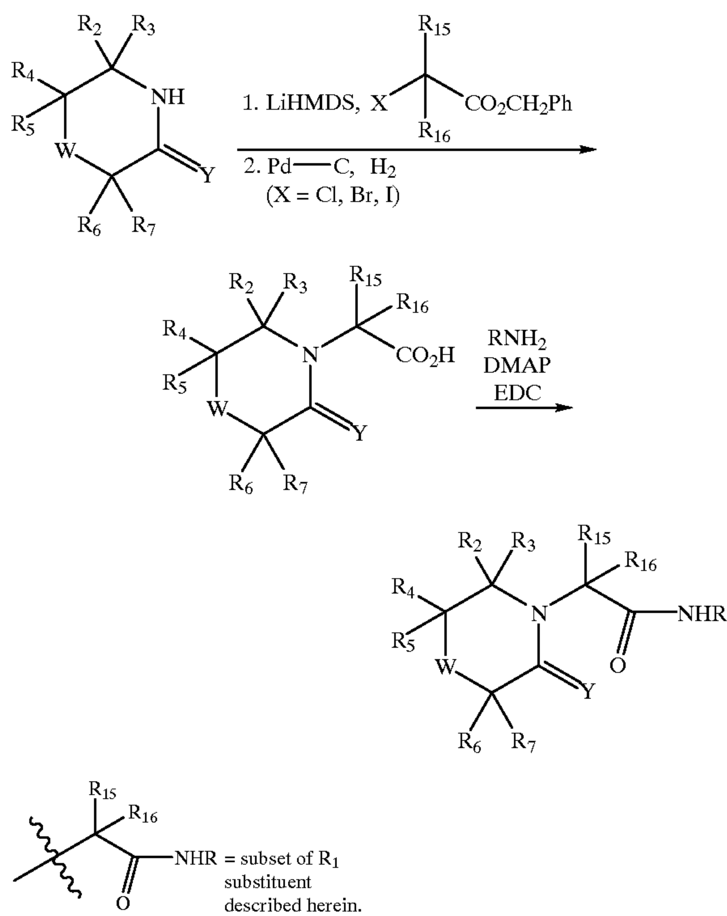
Scheme 18 General Synthesis of Compounds.
