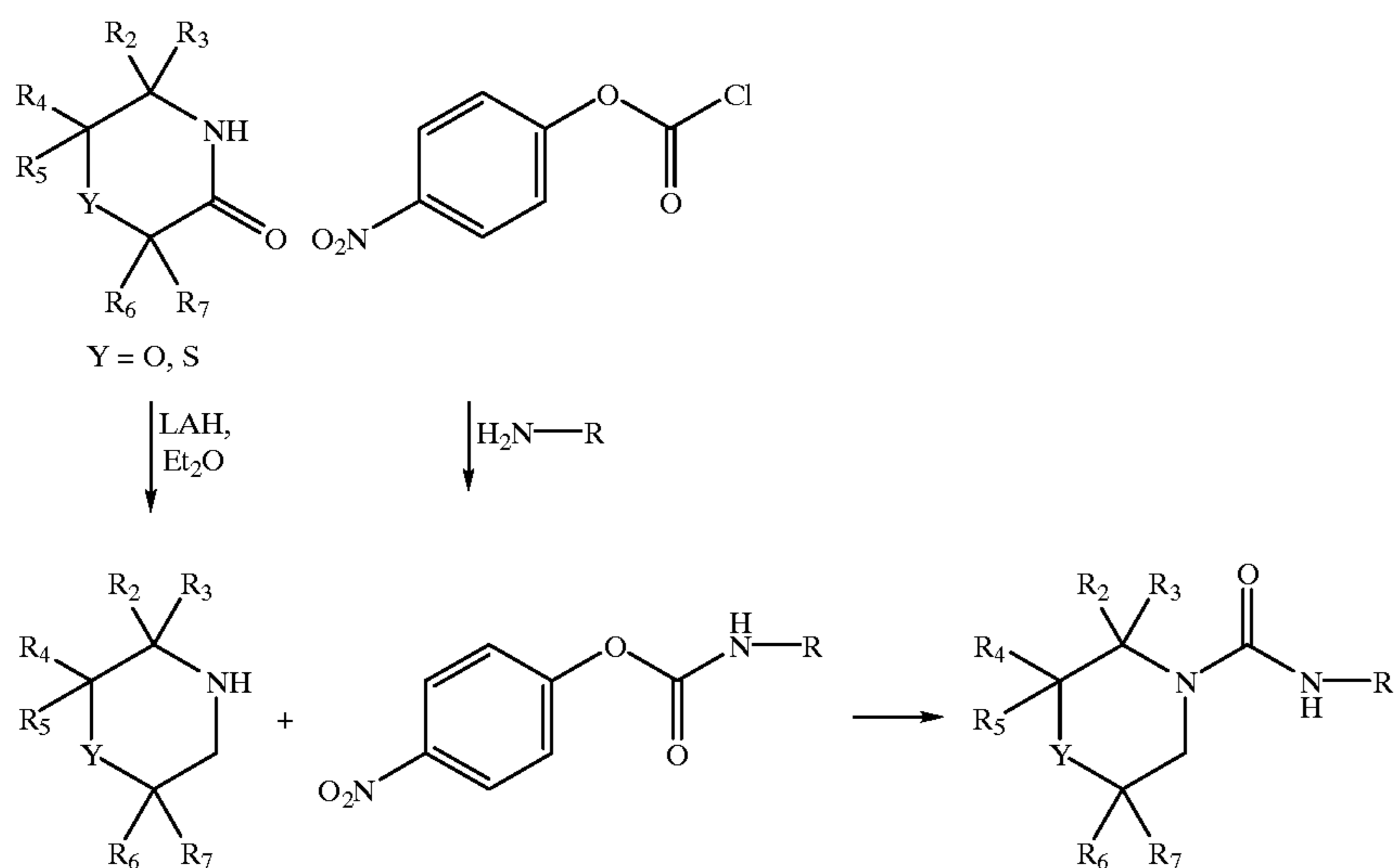
Scheme 12 General Synthesis of Morpholines and Thiomorpholines.
