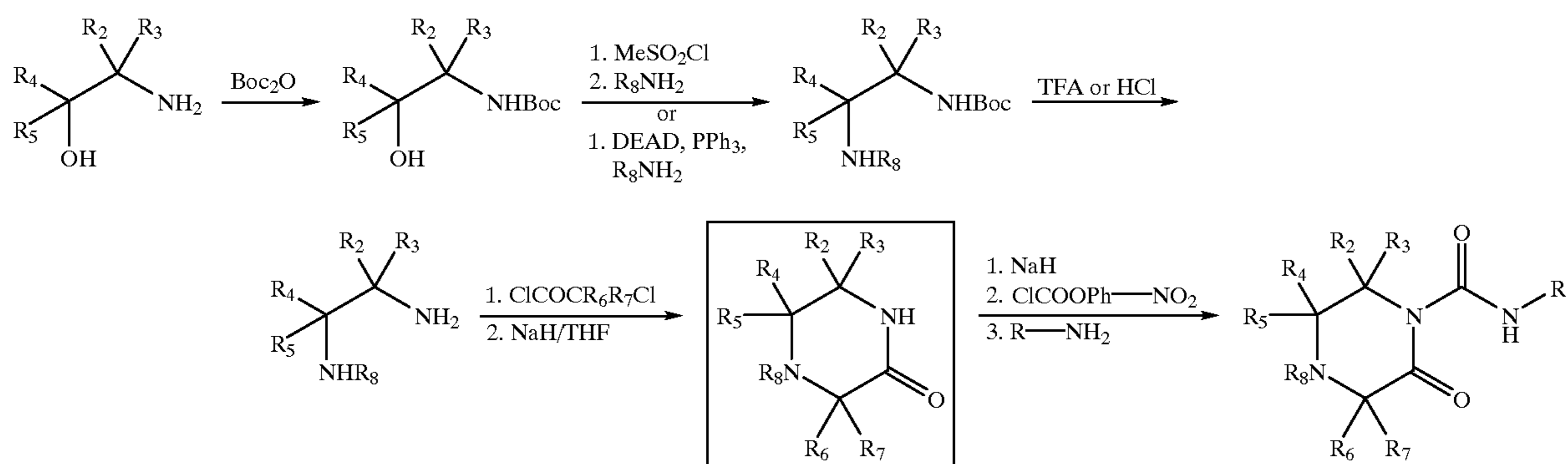
Scheme 13 General Synthesis of Piperizines and piperizinones.
