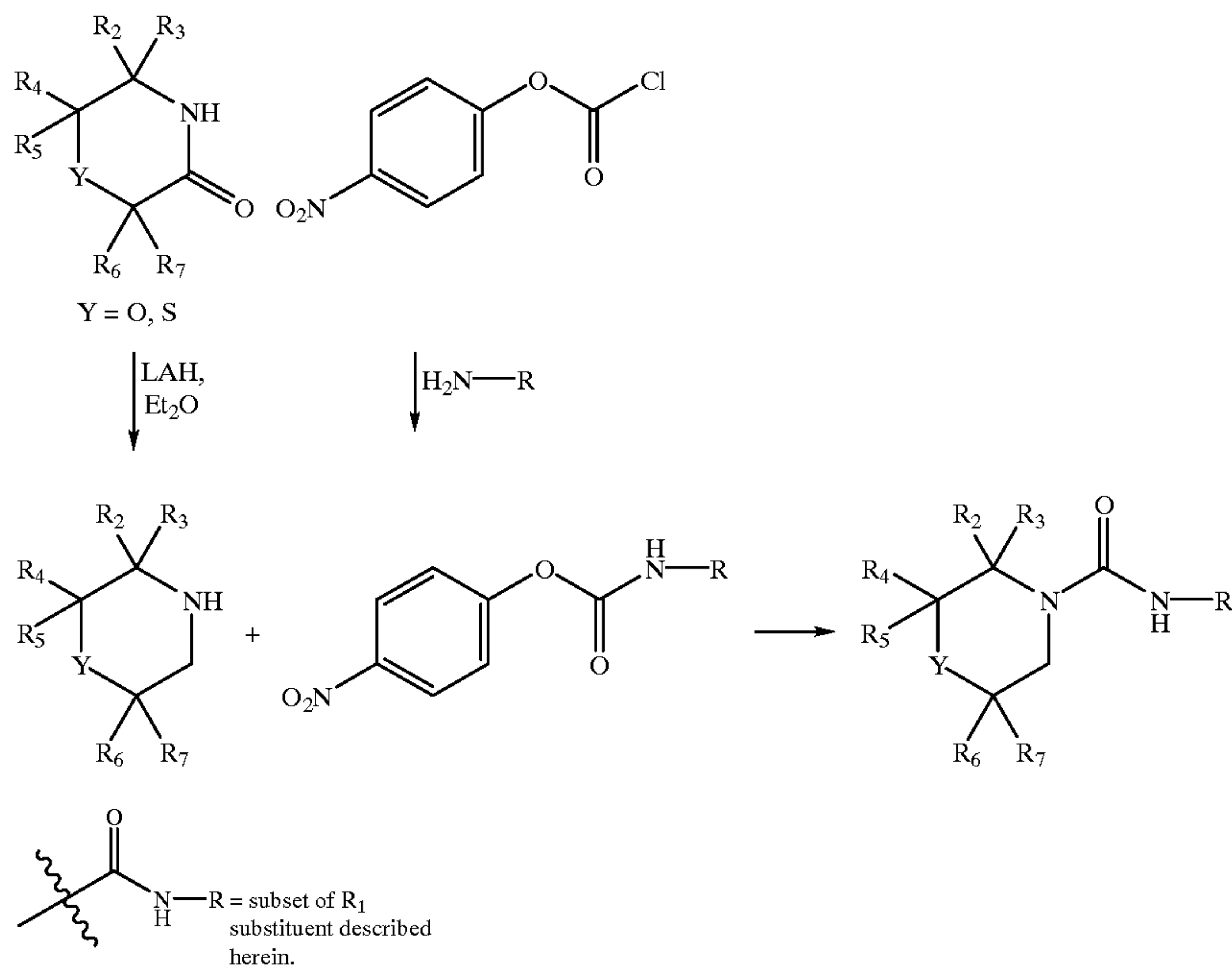
Scheme 12 General Synthesis of Morpholines and Thiomorpholines.
