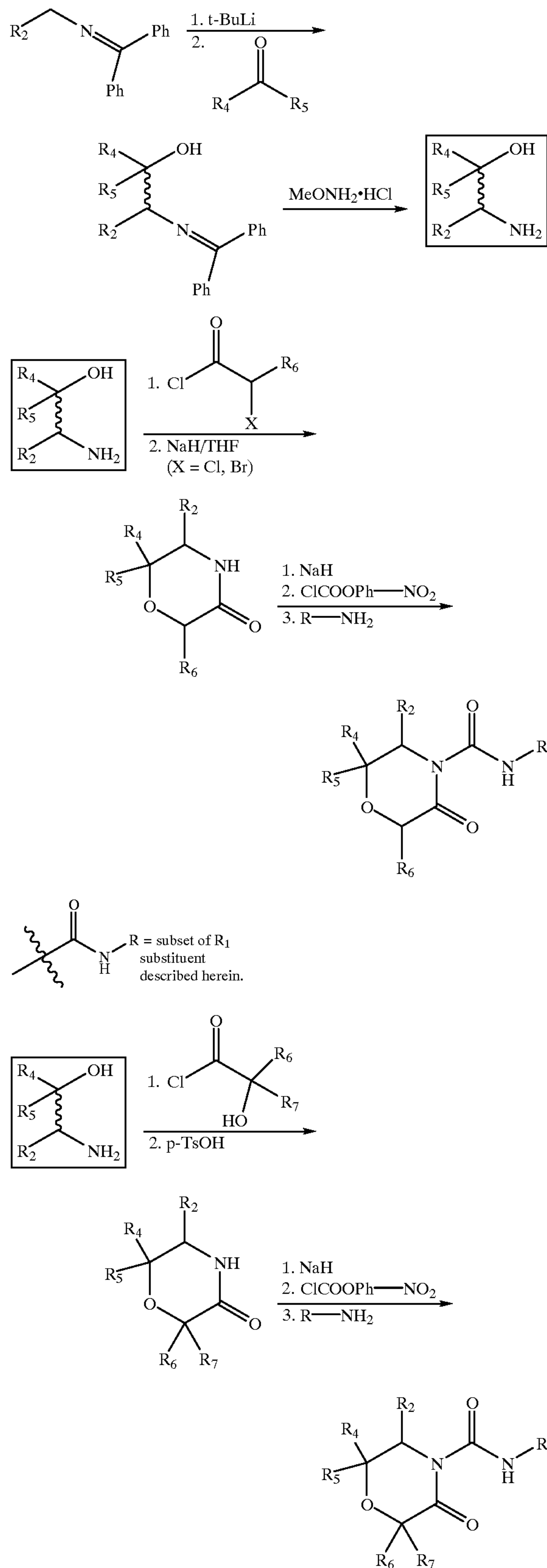
Scheme 8 General Synthesis of Substituted Morpholinones.
