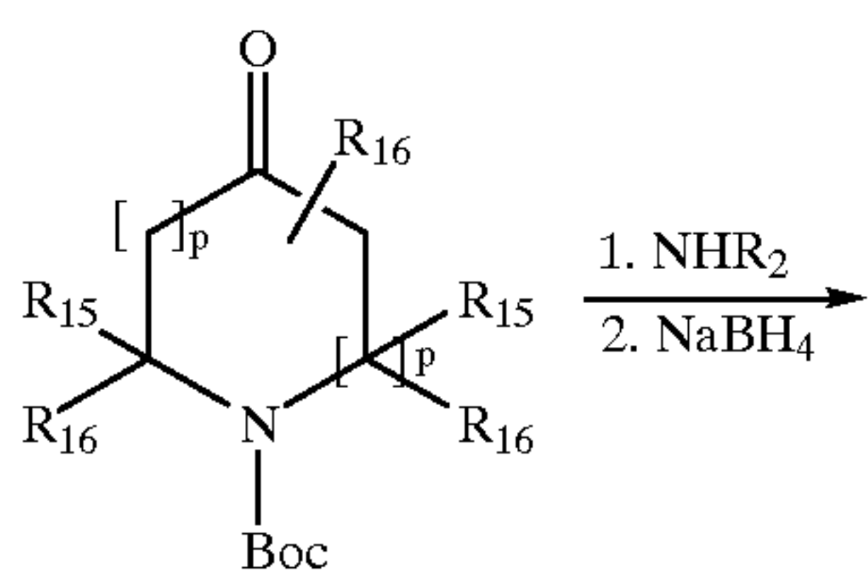
Scheme 20 General Synthesis of Compounds.
