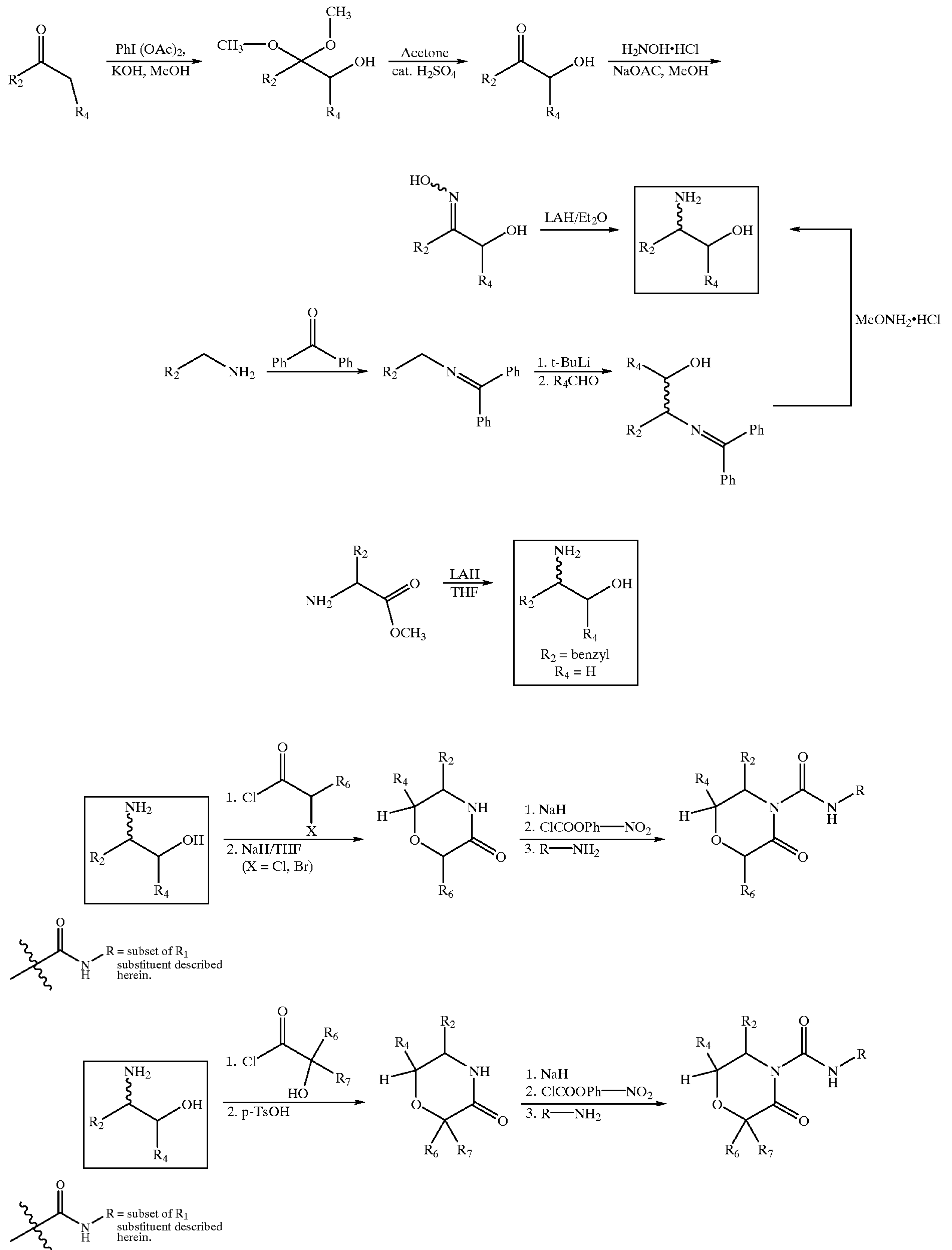
Scheme 7 General Synthesis of Substituted Morpholinones.
