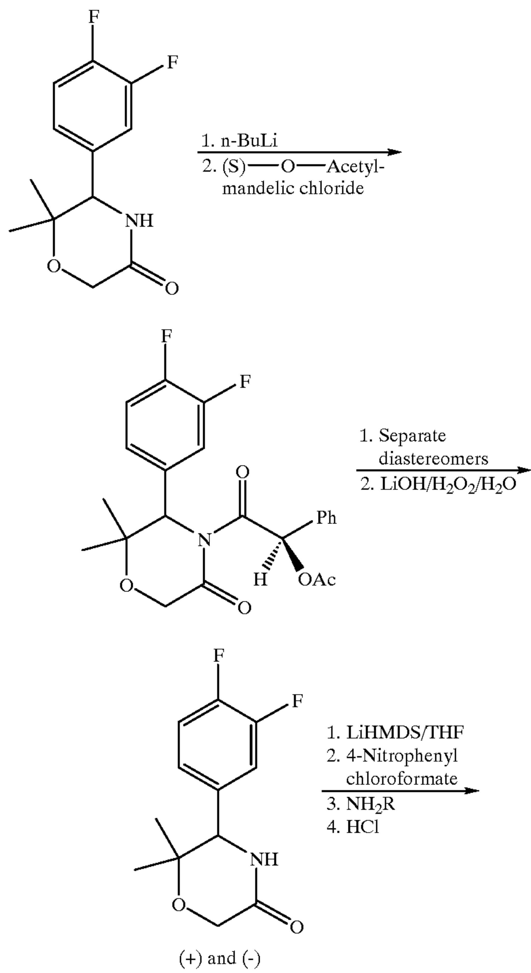
Scheme 4b Synthesis of Chiral Substituted Morpholinone Examples.
