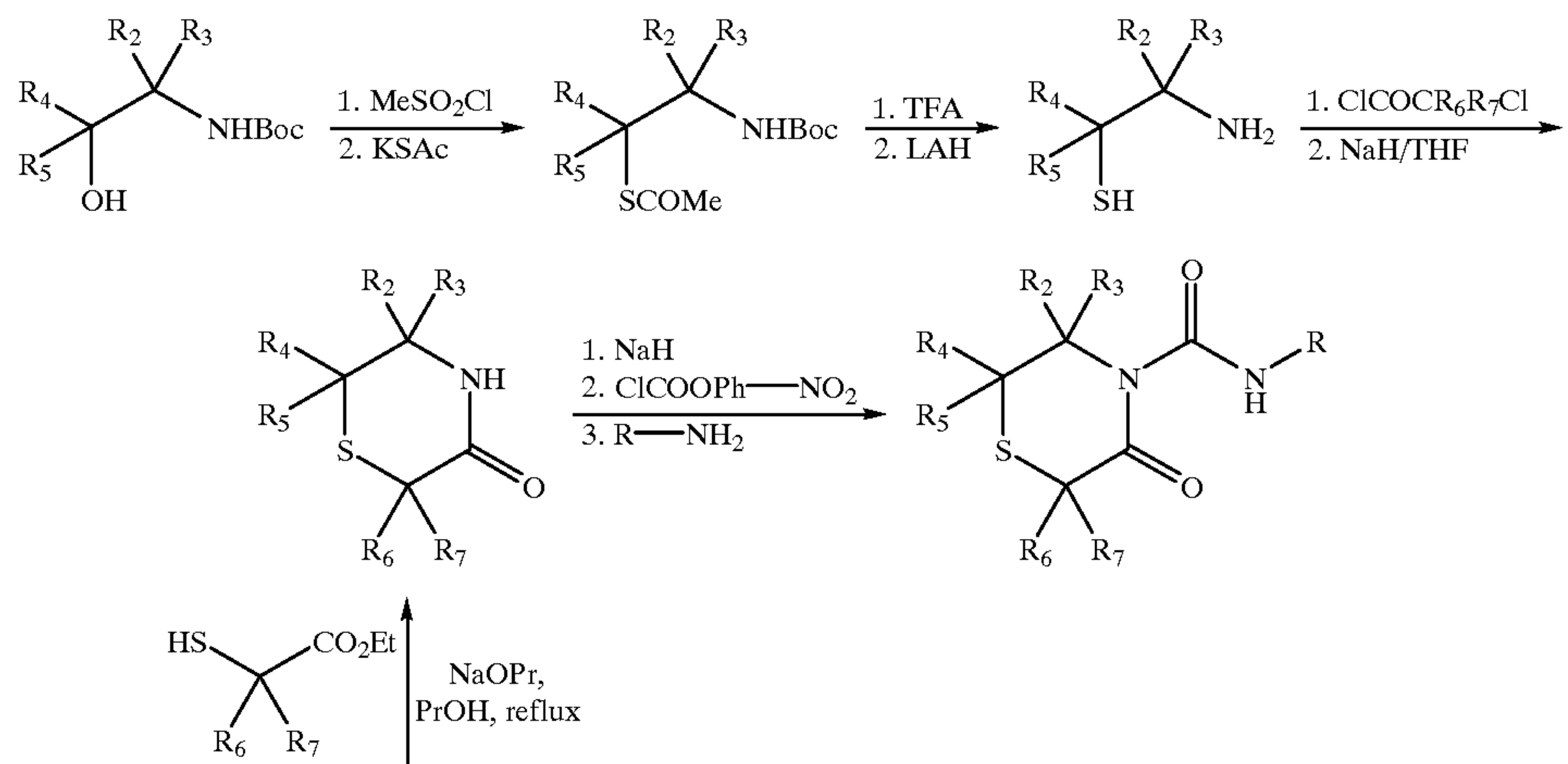
Scheme 11 General Synthesis of Thiomorpholinones.
