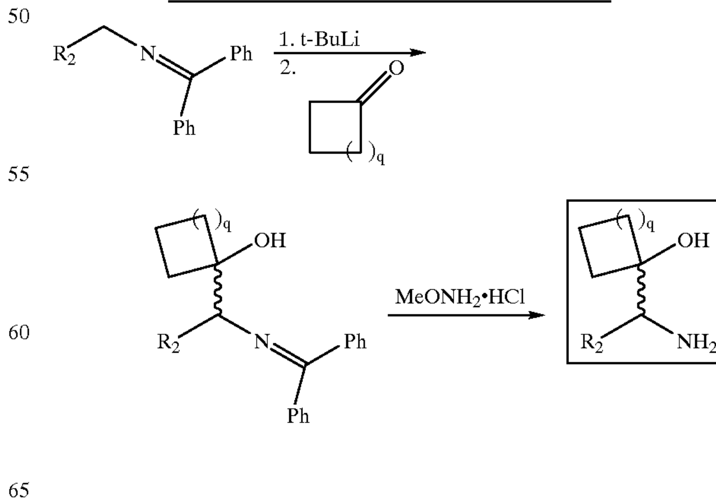
Scheme 10 General Synthesis of Spirocyclic Morpholinones.
