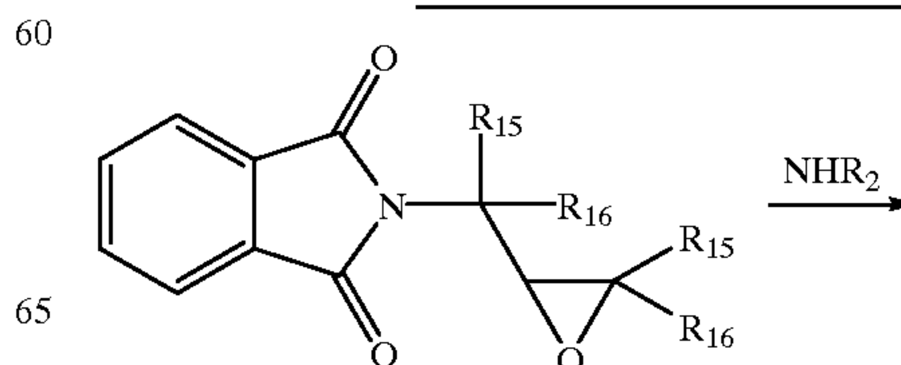
Scheme 22 General Synthesis of Compounds.
