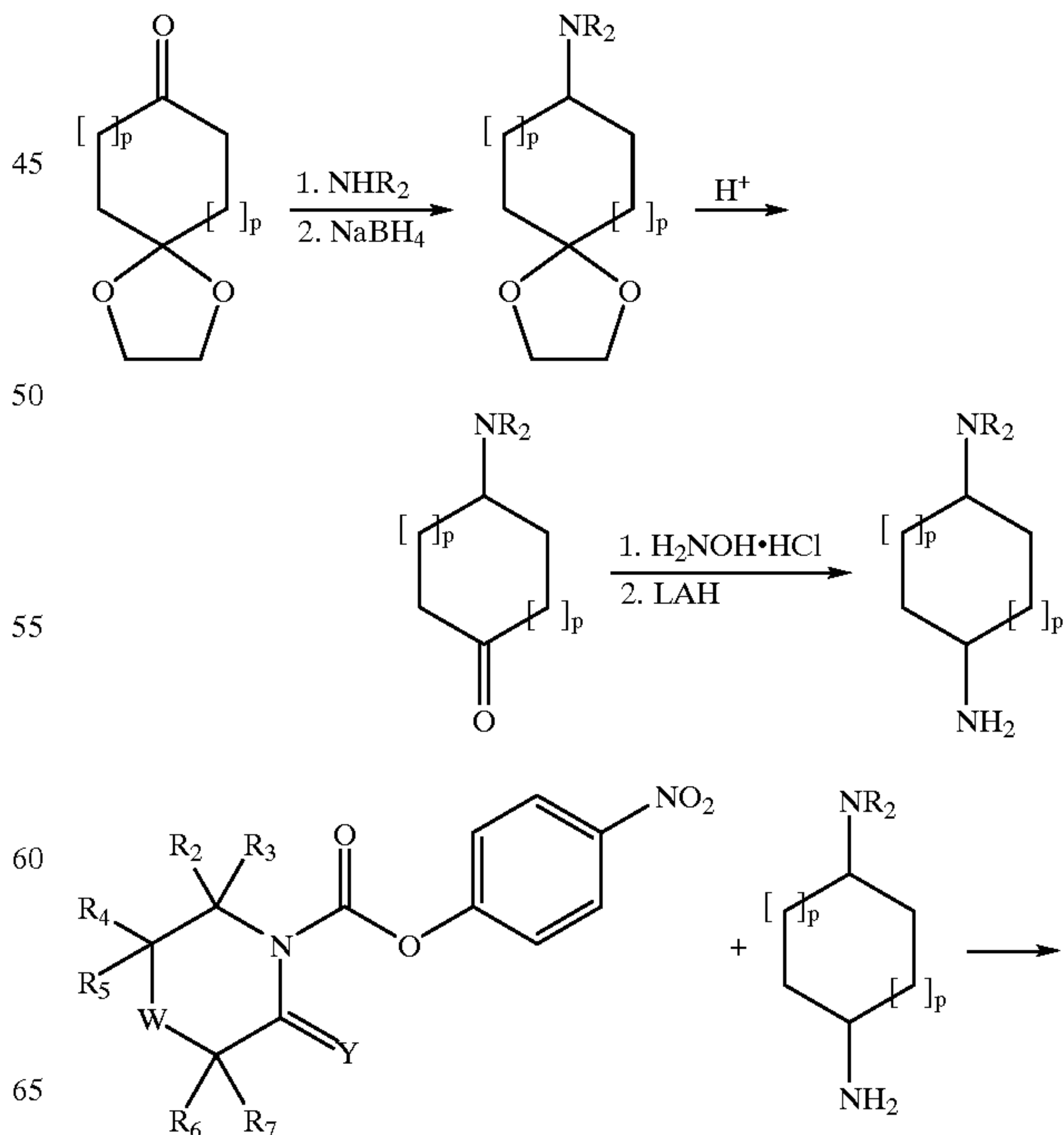
Scheme 19 General Synthesis of Compounds.
