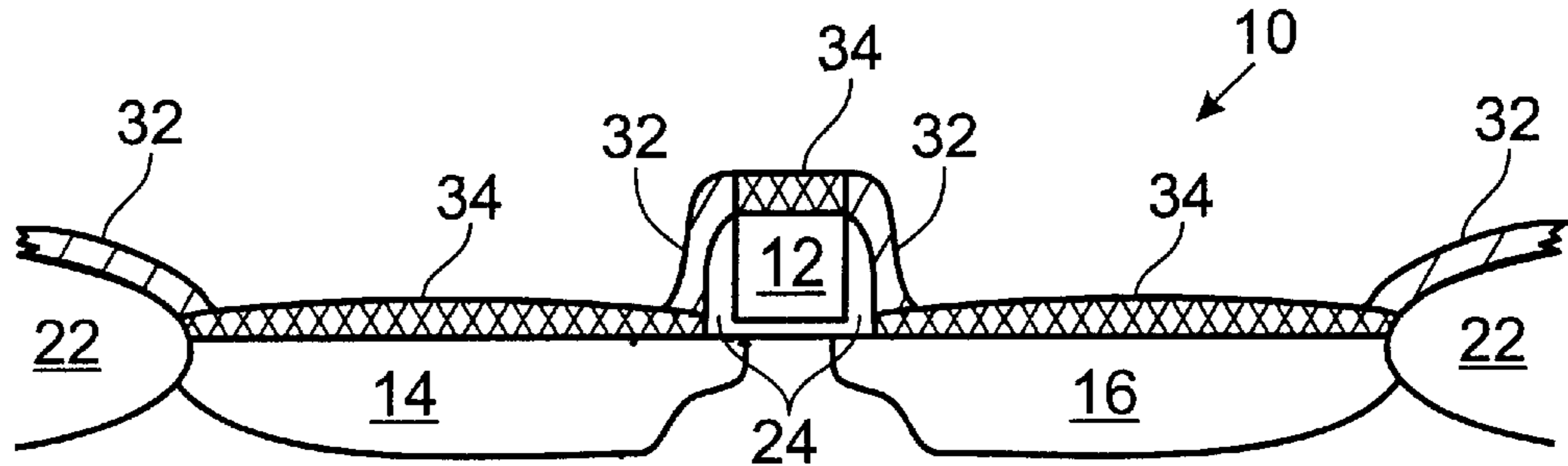
Fig. 4 (PRIOT ART)
