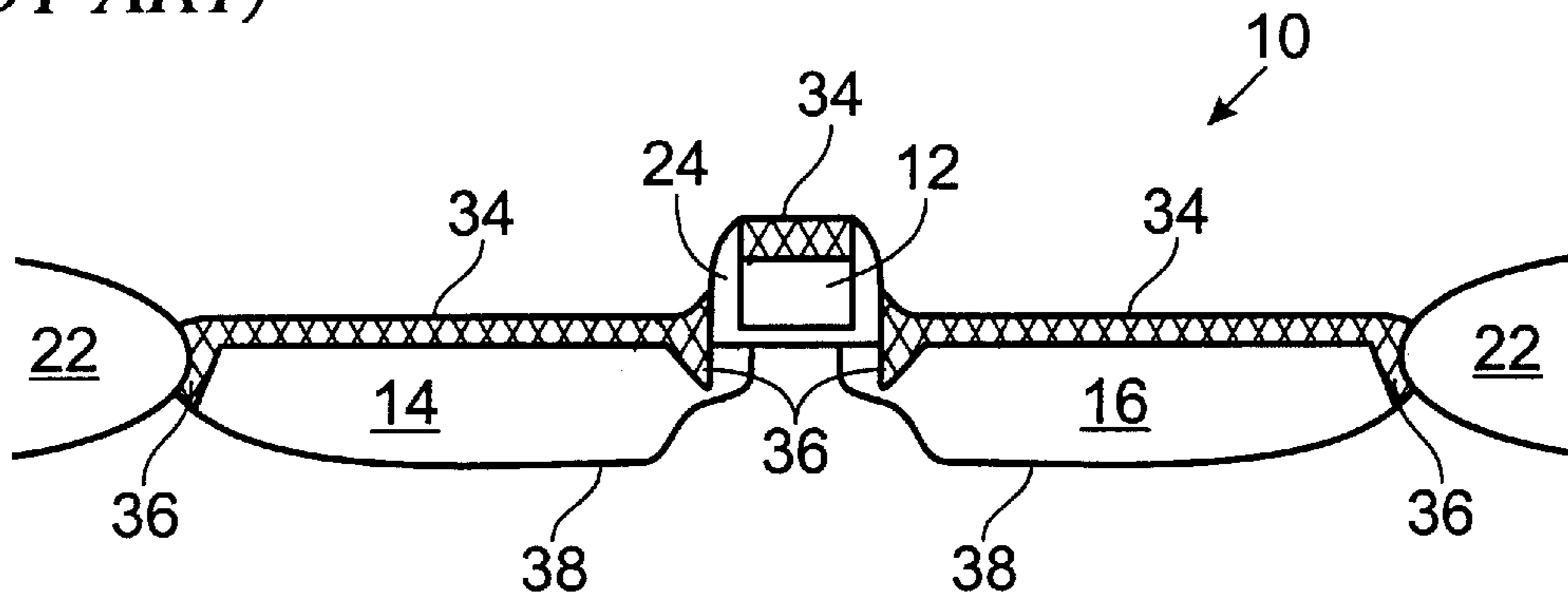
Fig. 5 (PRIOT ART)
