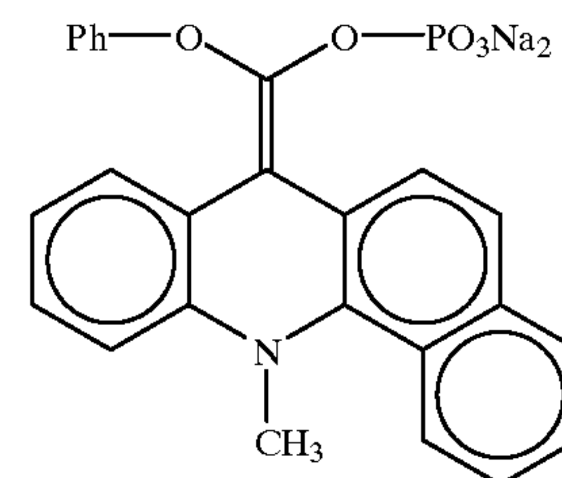
(E/Z mixture)
