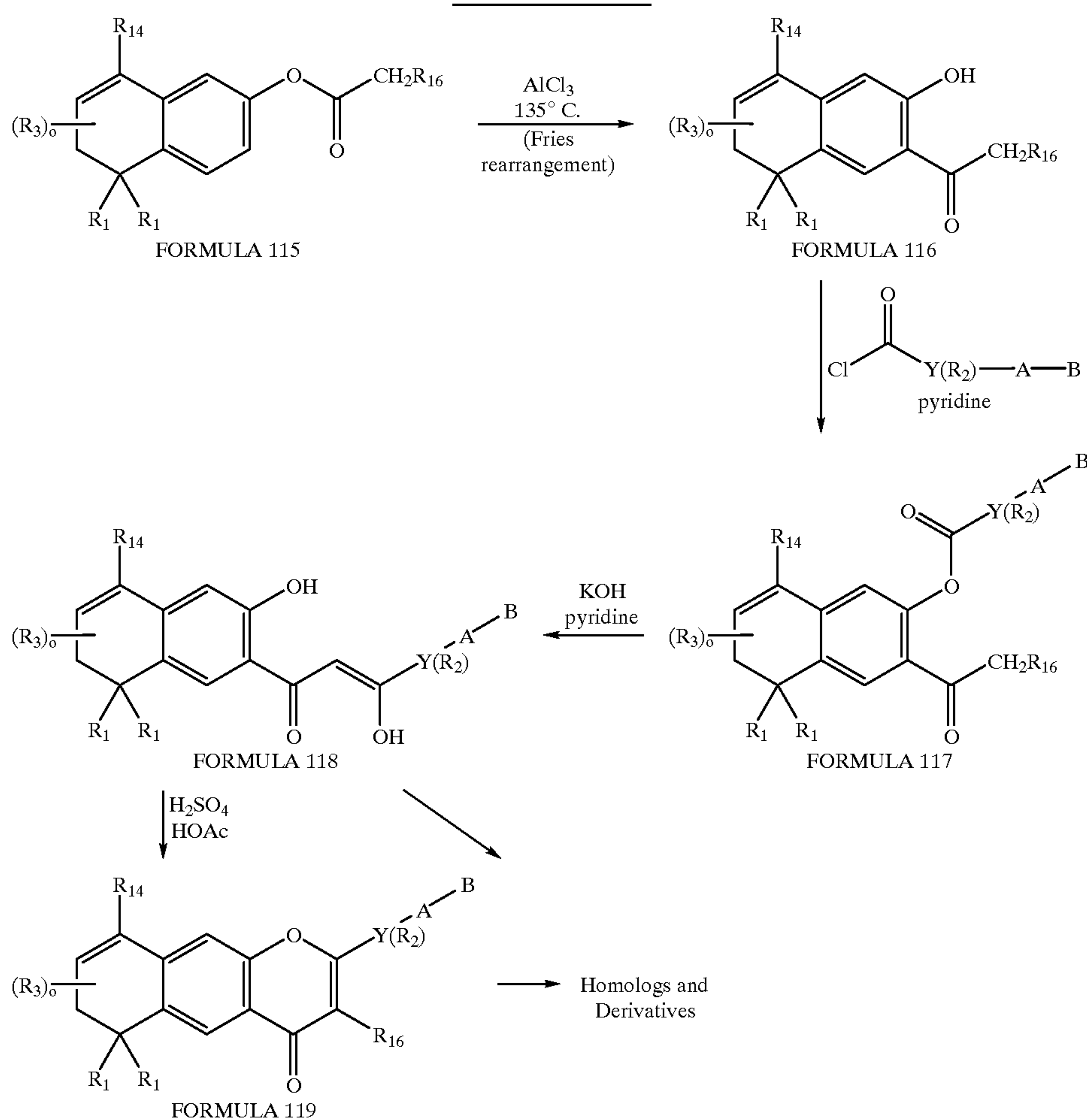
Reaction Scheme 102
