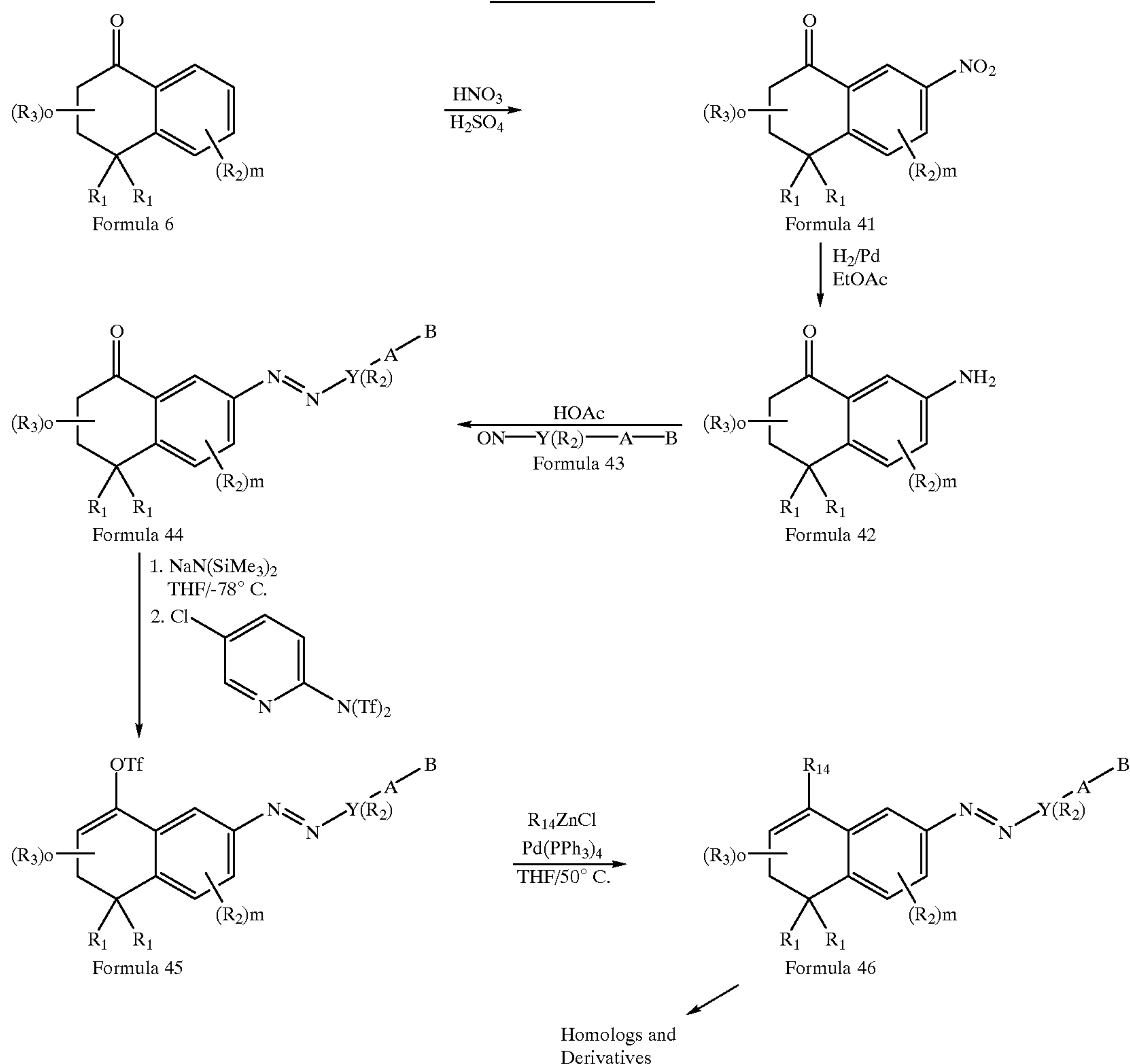
Reaction Scheme 5
