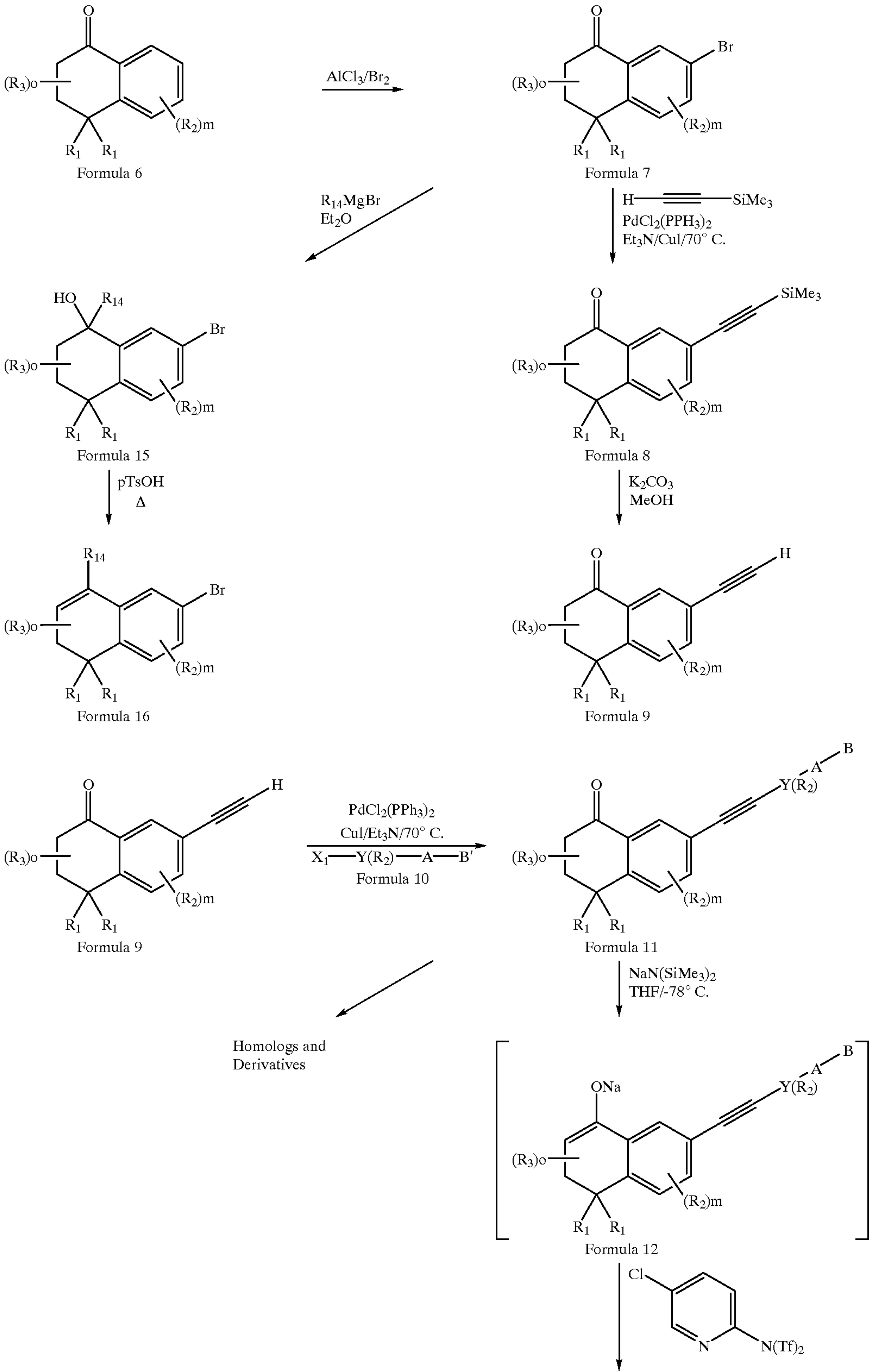
Reaction Scheme 1
