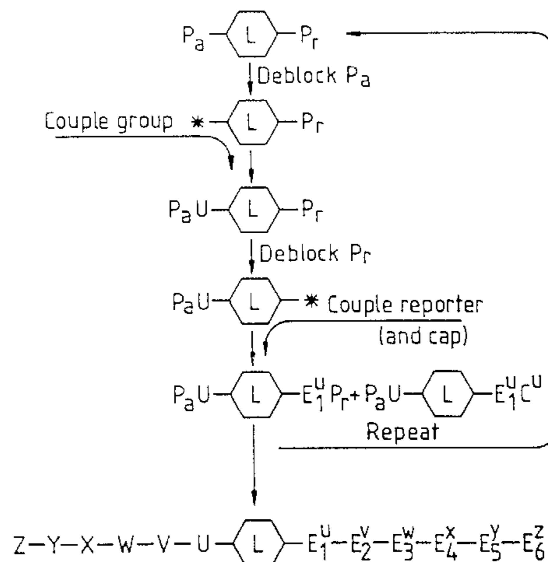
GENERAL SCHEME FOR SYNTHESIS OF MOLECULES WITH SPECIFIC TAGS
