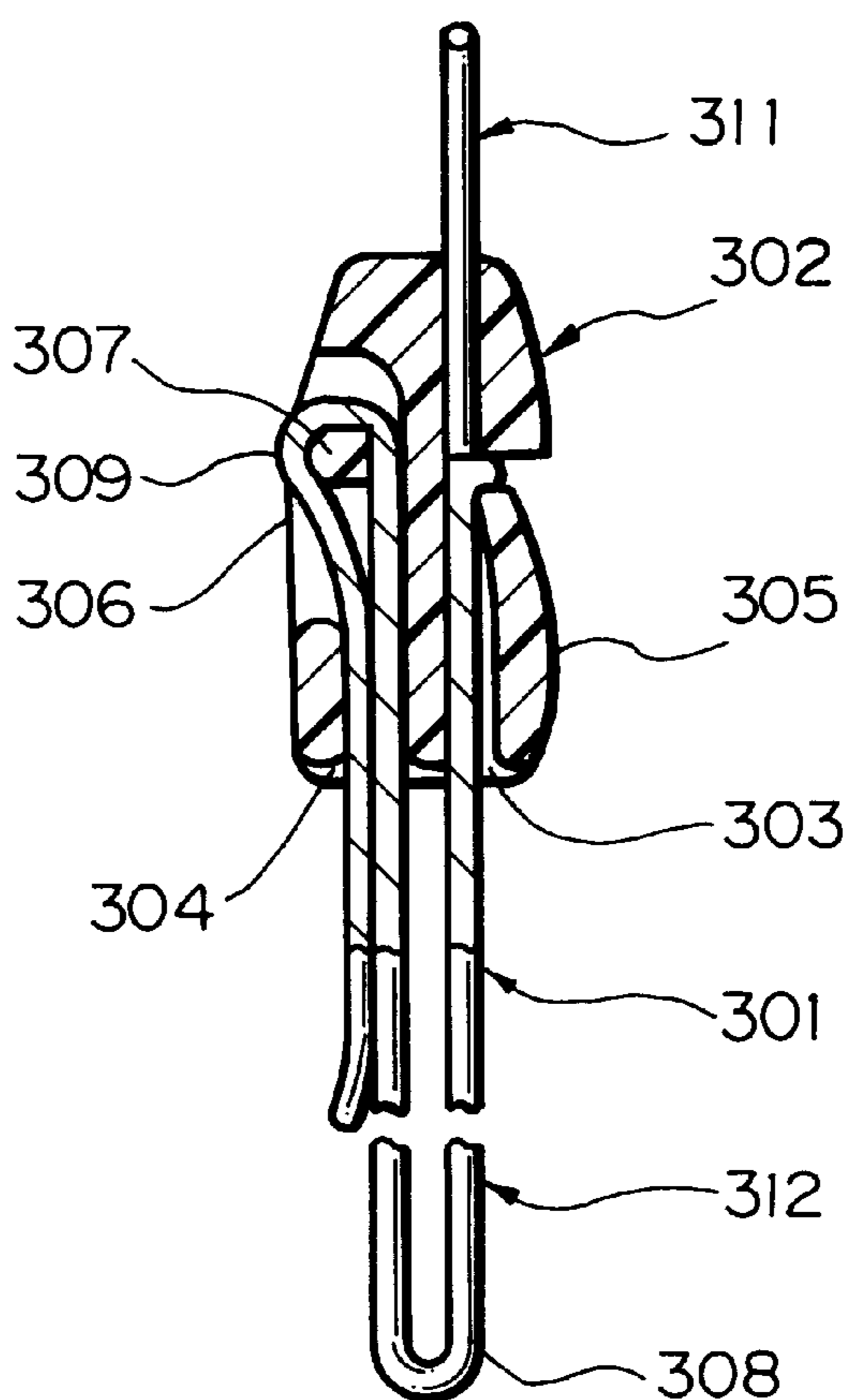
Fig. 2 PRIOR ART
