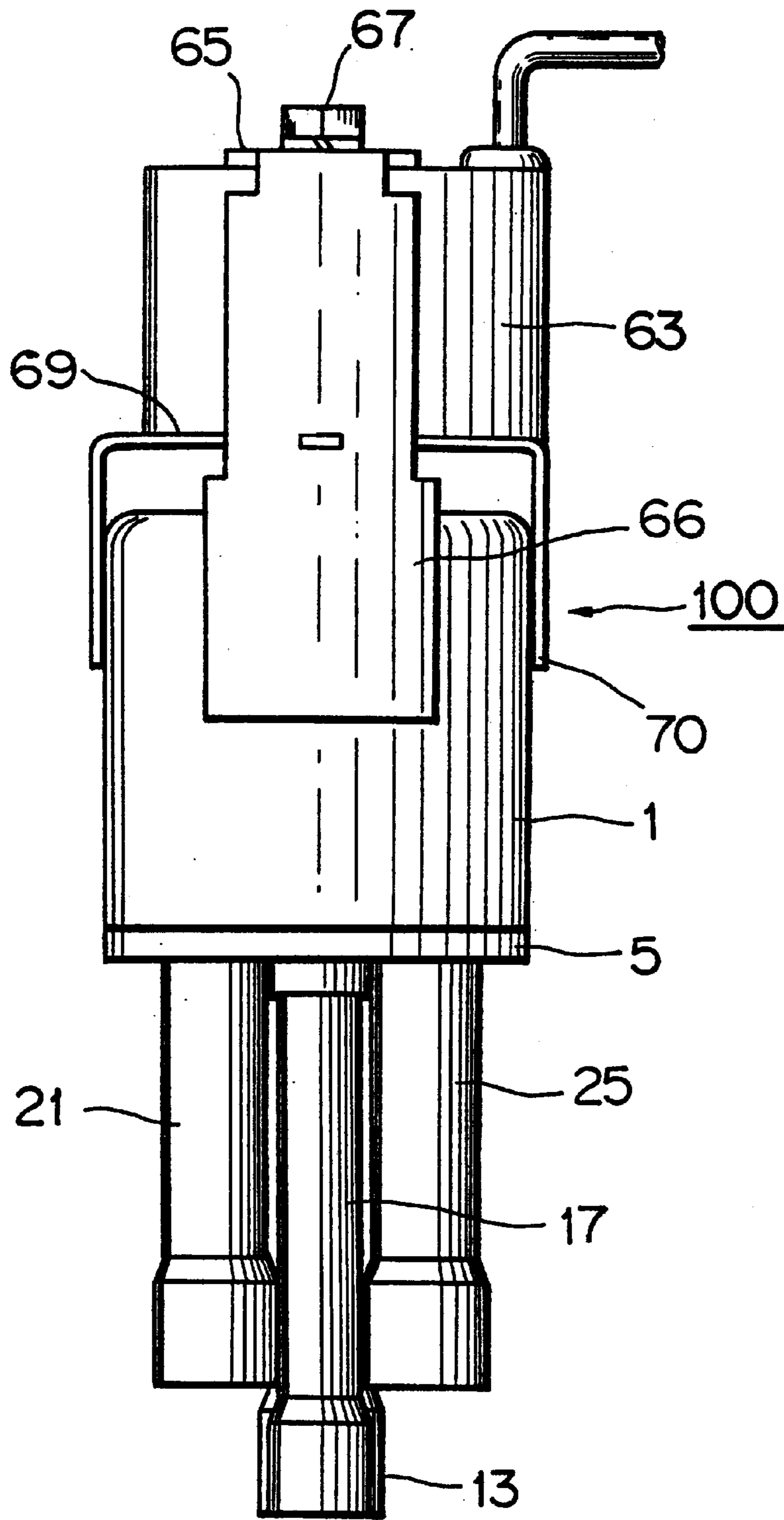
VIEW A (IN FIG. 1)
