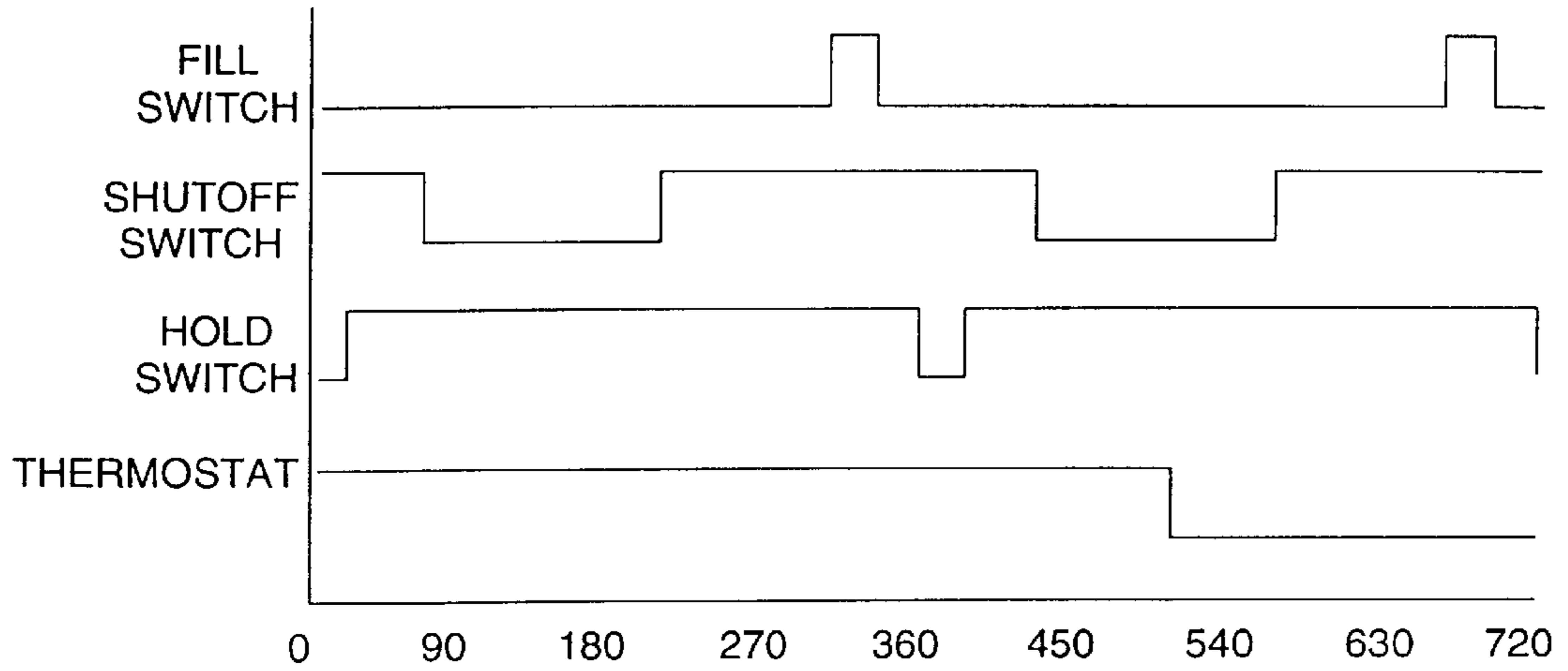
SWITCH STATE DIAGRAM FOR CURRENTLY AVAILABLE ICEMAKERS
