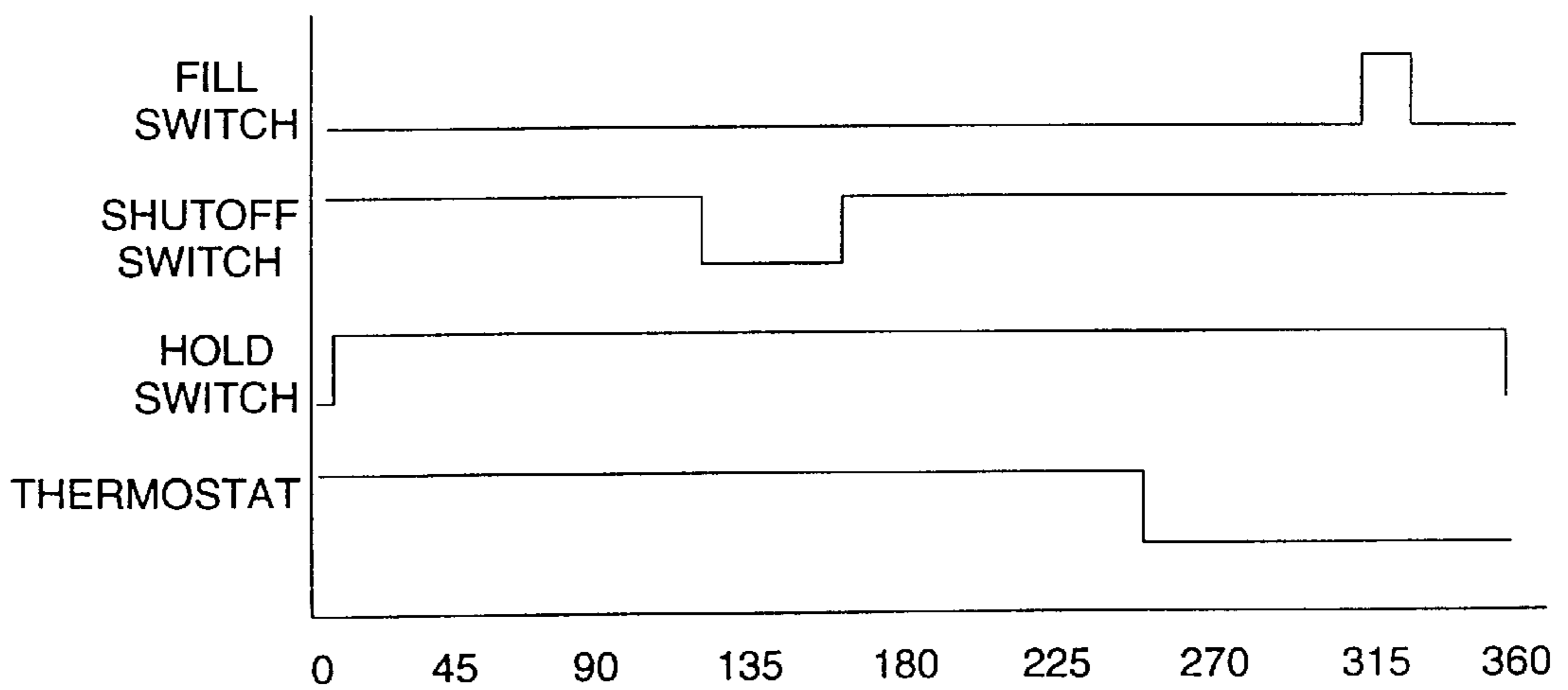
SWITCH STATE DIAGRAM FOR NEW CONTROL CIRCUIT
