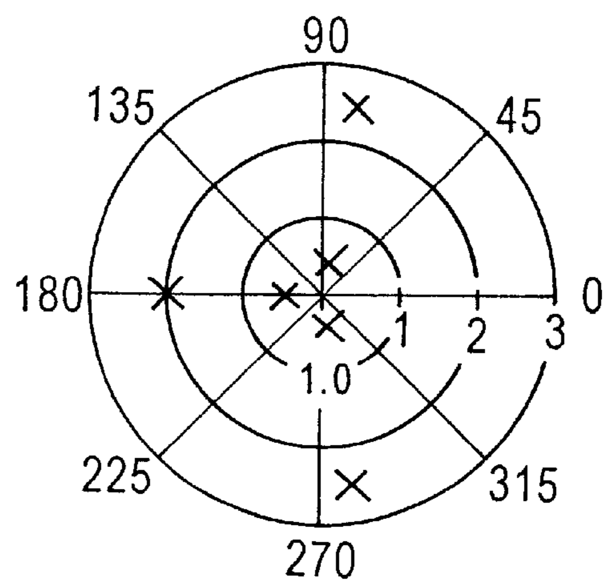
Complex Roots of X(z)
