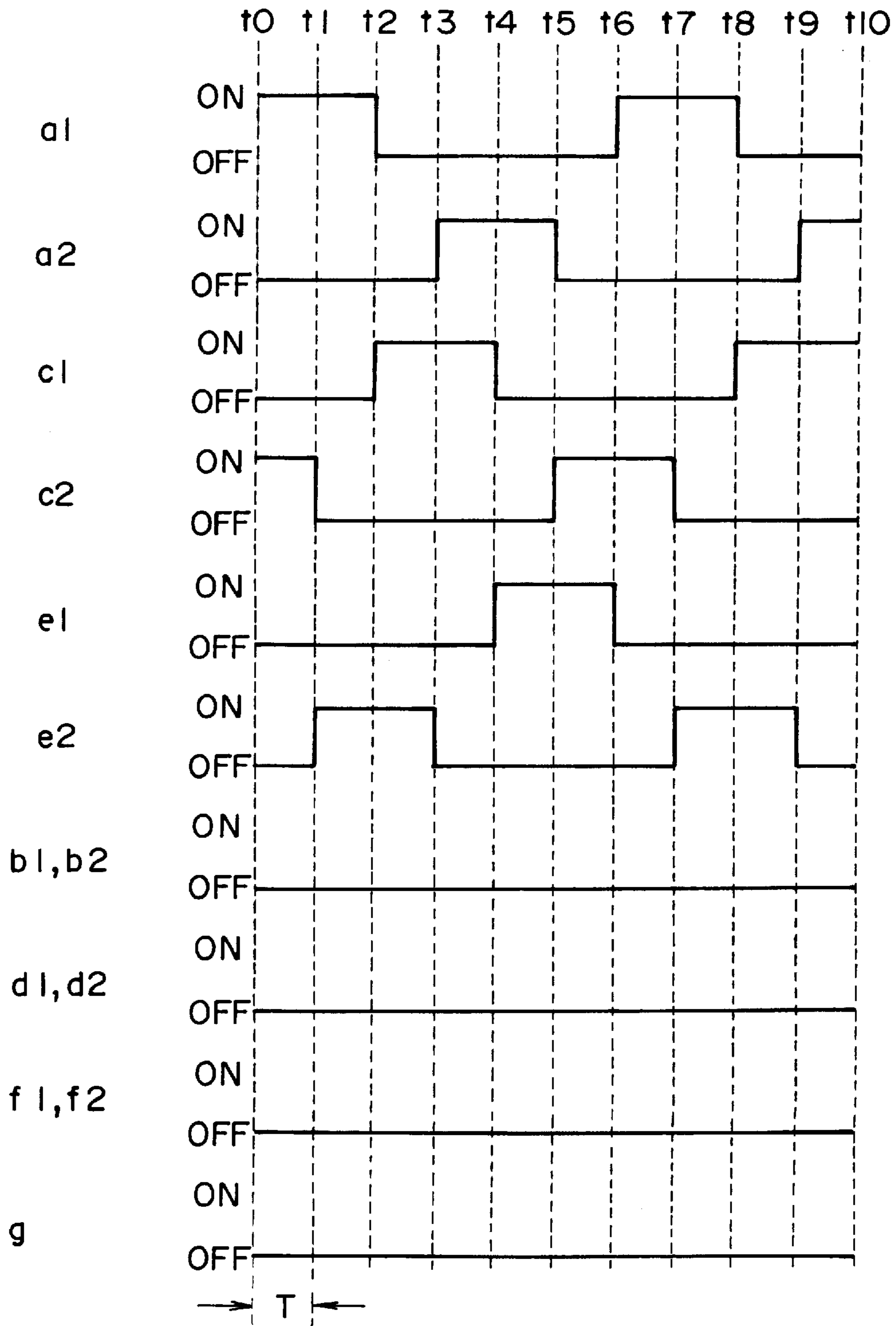
TIMING CHARTS
