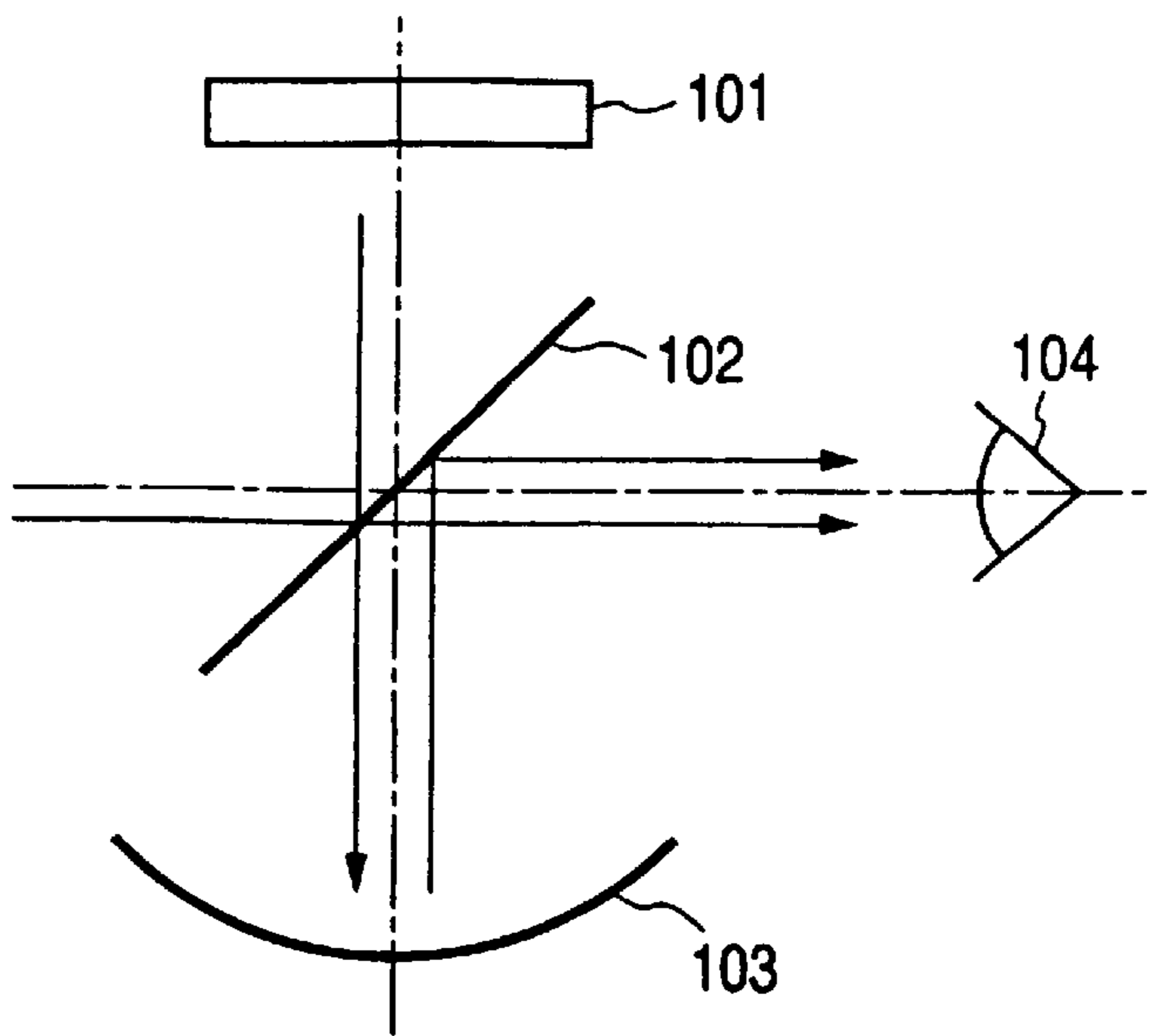
FIG. 18 PRIOR ART
