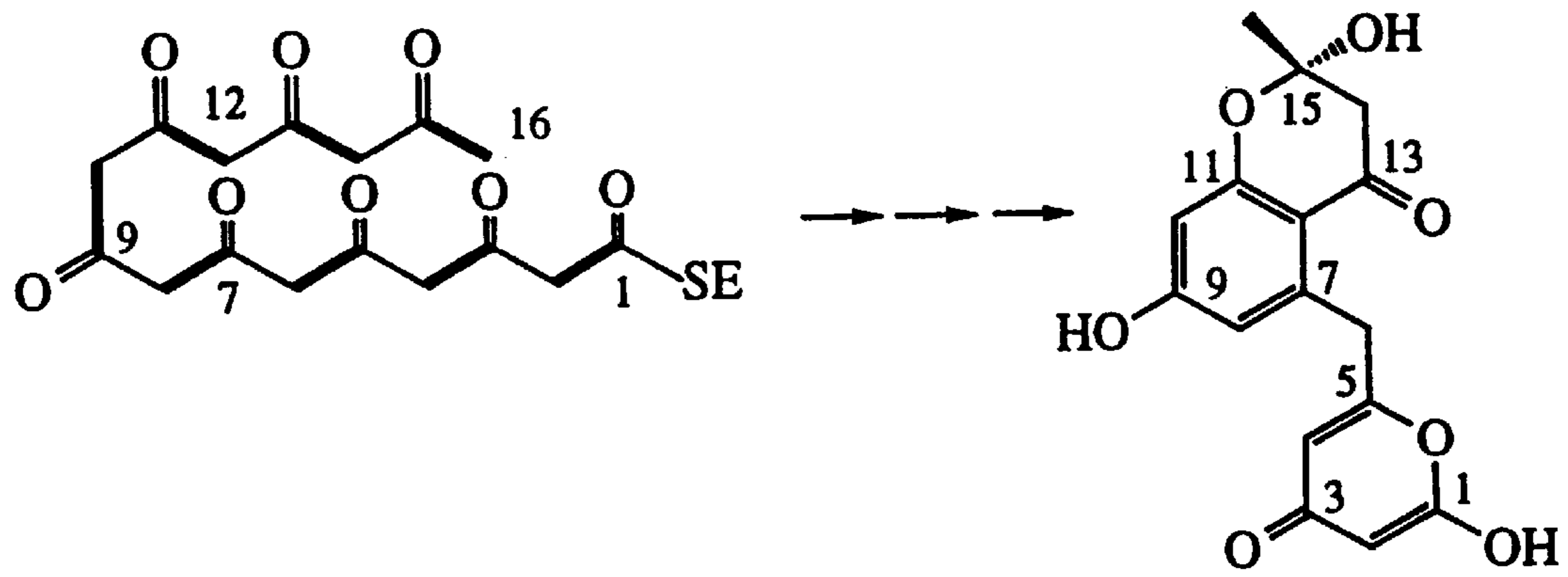
SEK4 (12)
