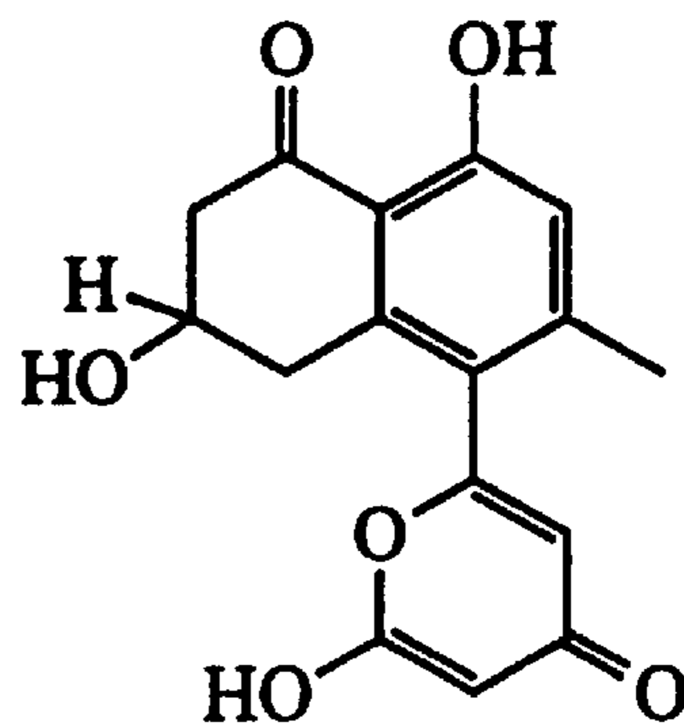
MUTACTIN (6)
