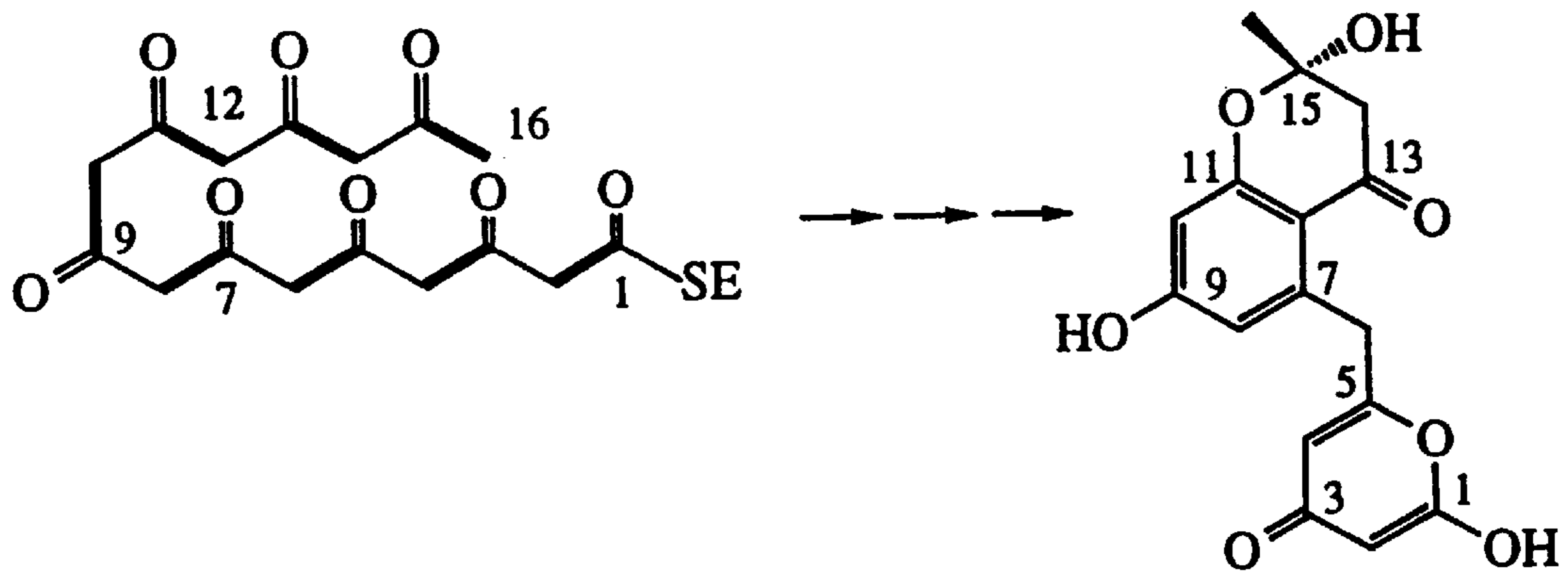
SEK4 (12)
