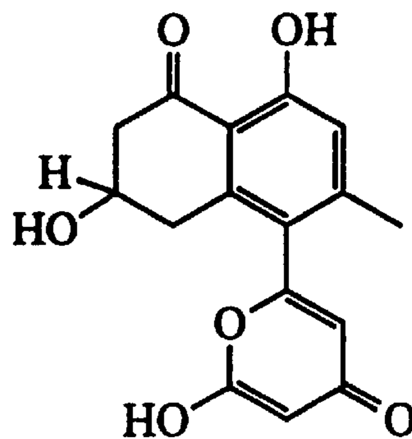
MUTACTIN (6)
