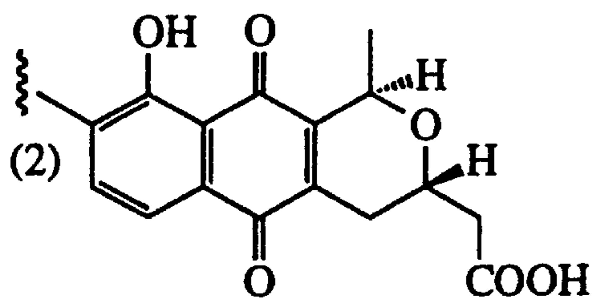
ACTINORHODIN (3)
