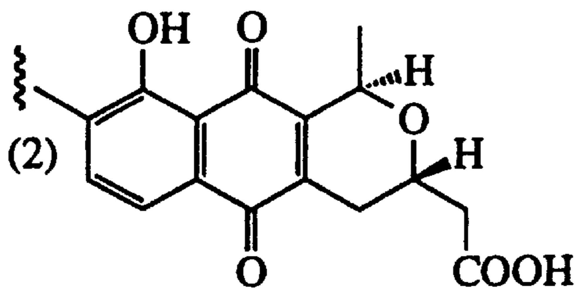
ACTINORHODIN (3)
