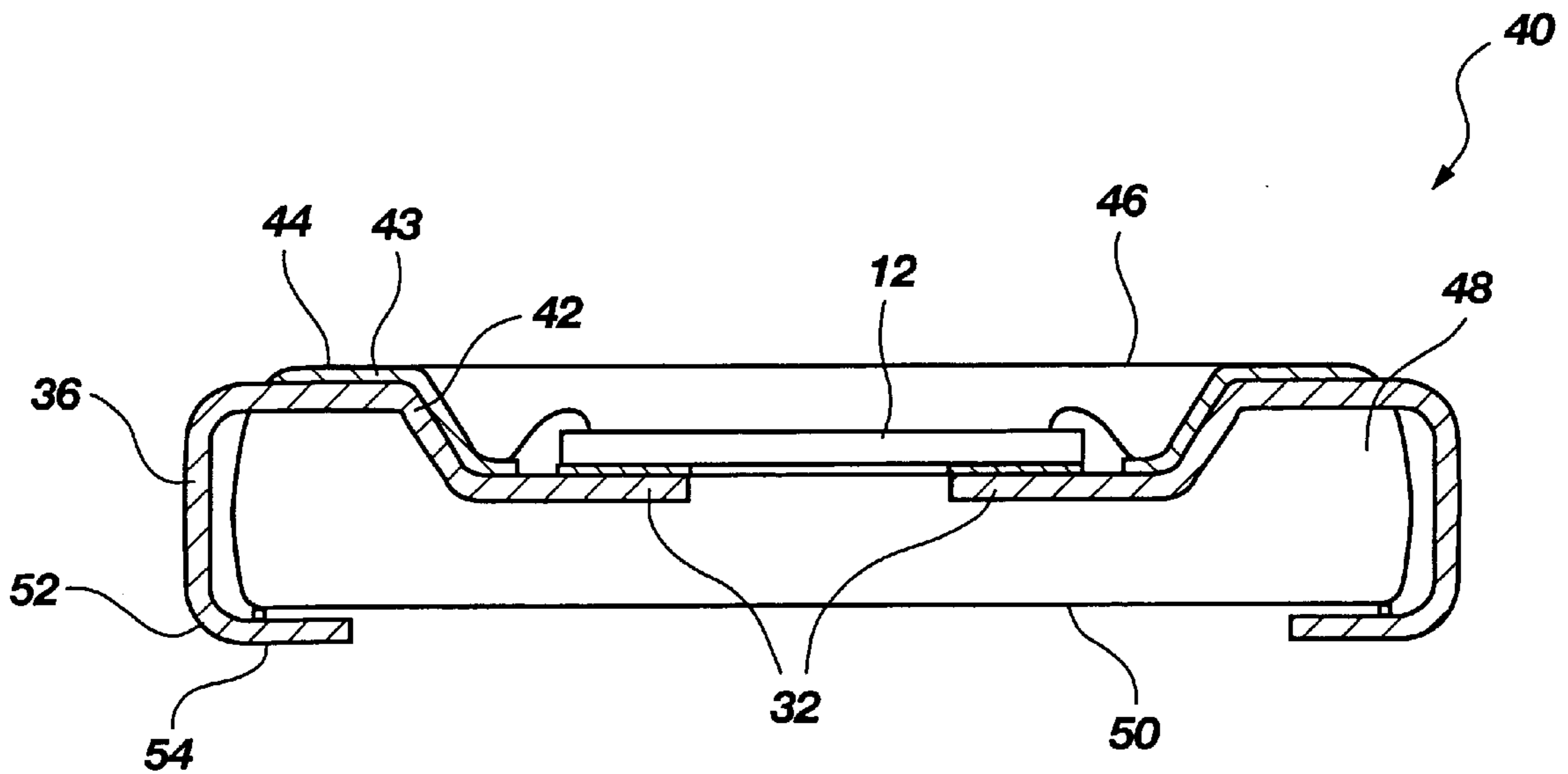
Fig. 4 (PRIOR ART)
