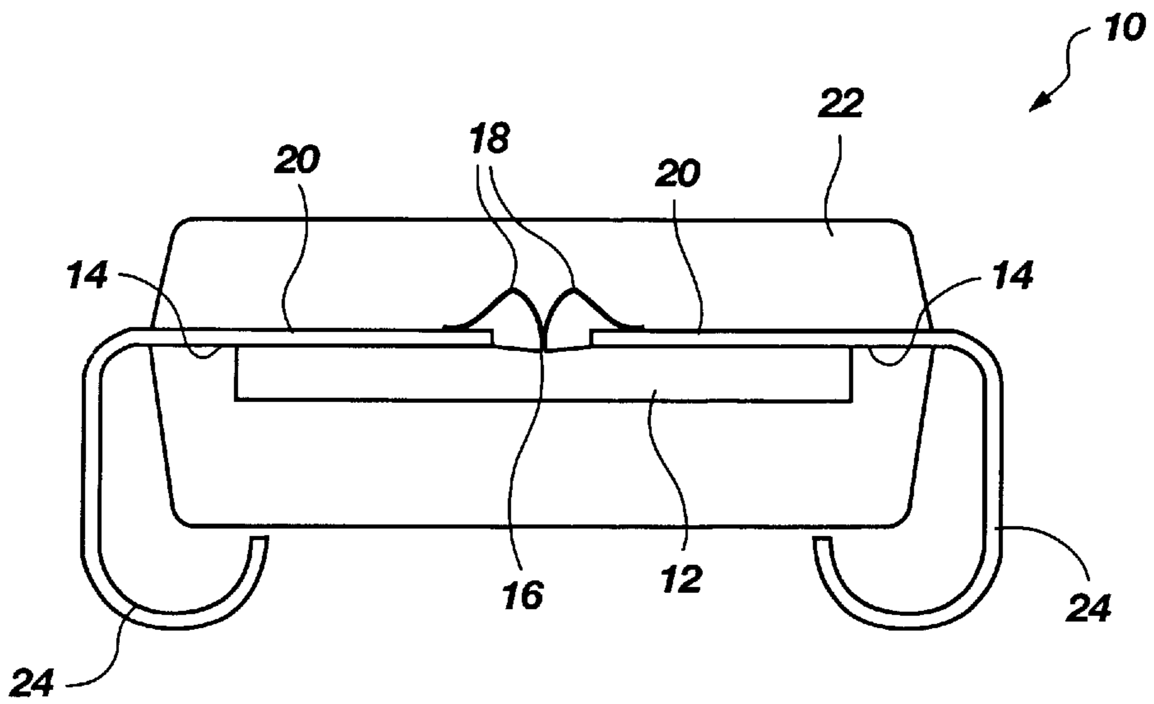
Fig. 1 (PRIOR ART)
