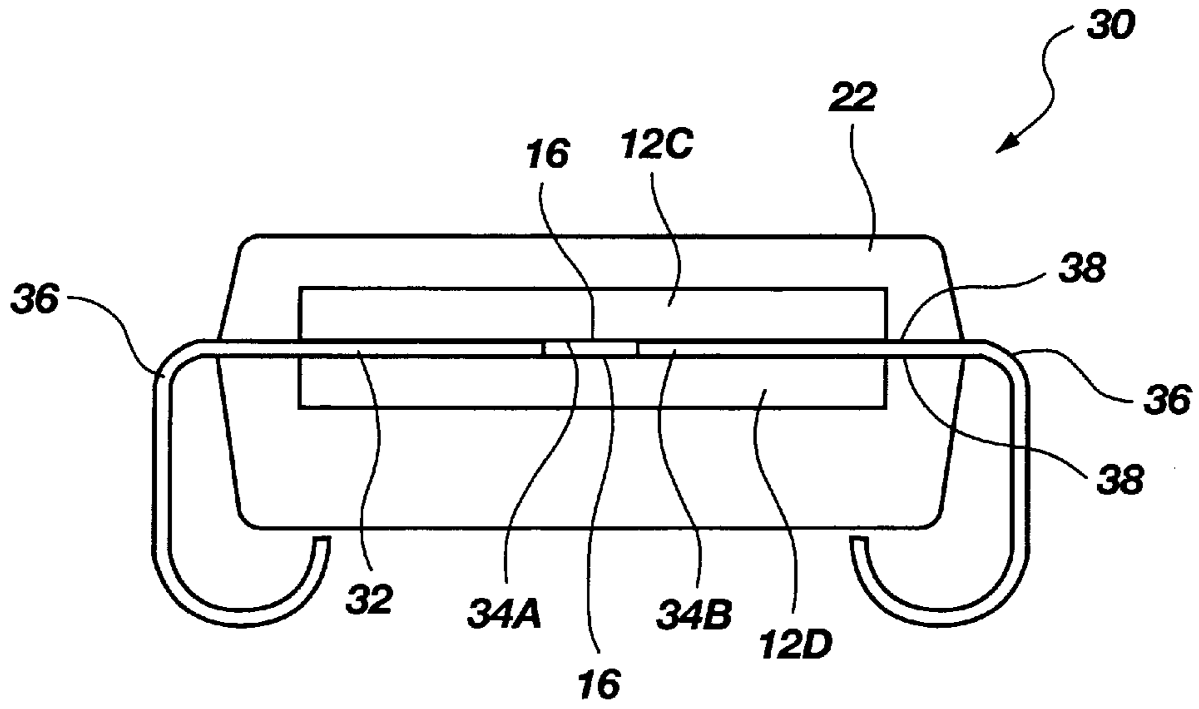
Fig. 3 (PRIOR ART)
