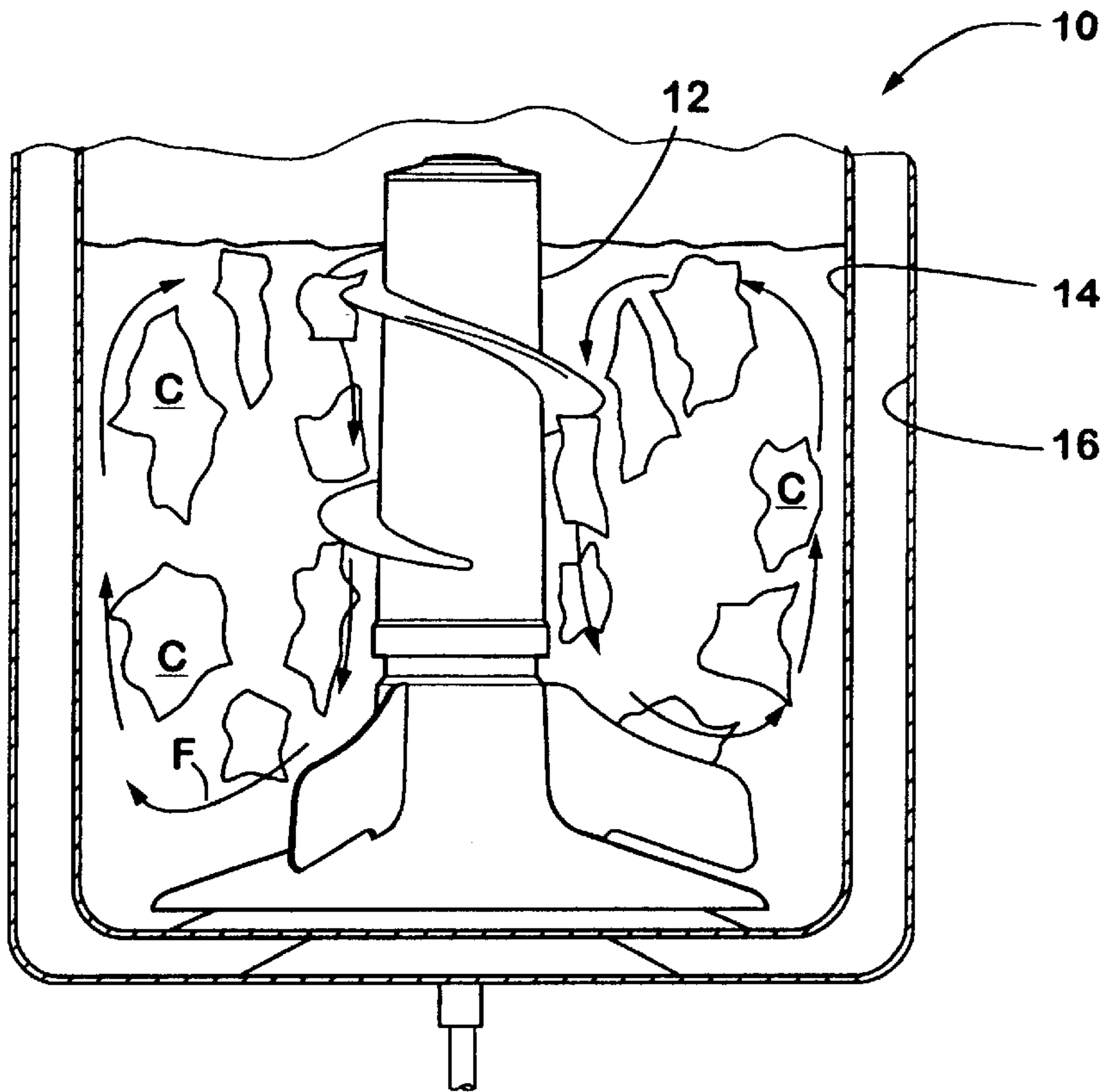
Fig. 1 PRIOR ART
