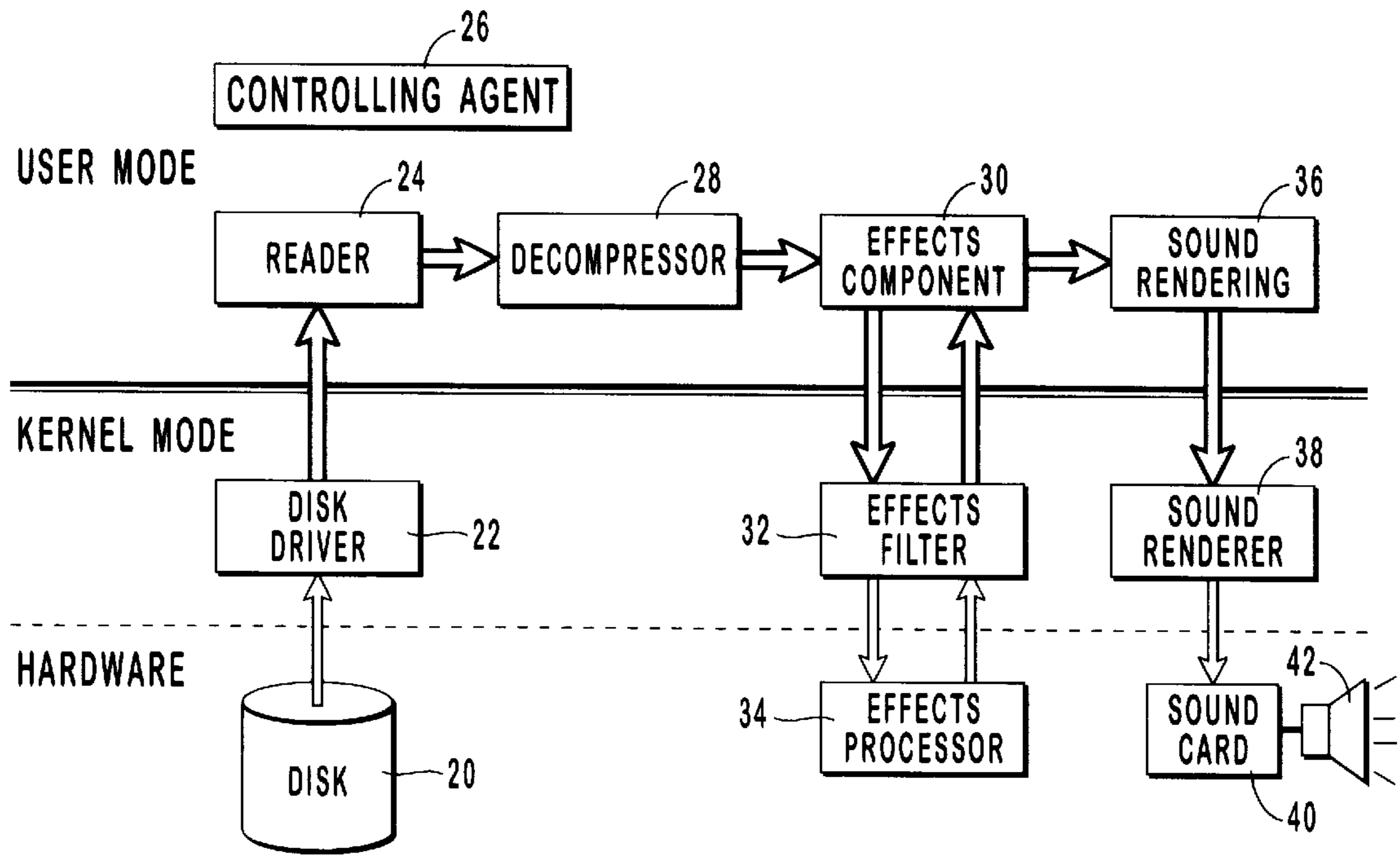
FIG. 1 (PRIOR ART)
